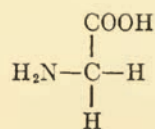
L-Glycine or aminoacetic acid
