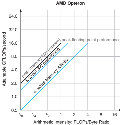
FIGURE 6.20 Roofline model with ceilings. The top graph shows the computational “ceilings” of 8 GFLOPs/sec if the floating-point operation mix is imbalanced and 2 GFLOPs/sec if the optimizations to increase ILP and SIMD are also missing. The bottom graph shows the memory bandwidth ceilings of 11 GB/sec without software prefetching and 4.8 GB/sec if memory affinity optimizations are also missing.
