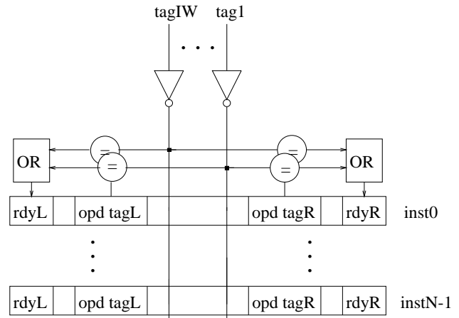
Figure 4: Wakeup logic.
