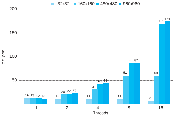
FIGURE 6.27 DGEMM performance versus the number of threads for four matrix sizes. The performance improvement compared unoptimized code in Figure 3.21 for the 960 × 960 matrix with 16 threads is an astounding 212 times faster!
