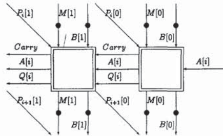
Fig. 2. The rightmost cells.
