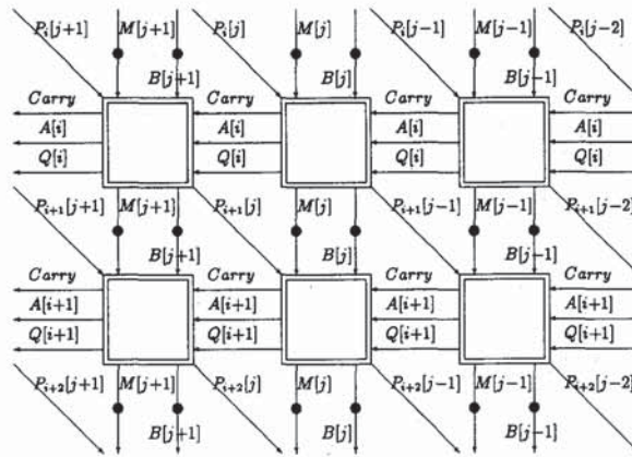
Fig. 1. Arrangement of modular multiplication cells.
