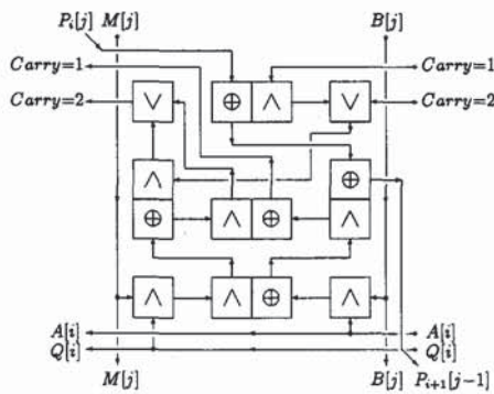
Fig. 3. The typical cell for radix r = 2 .
