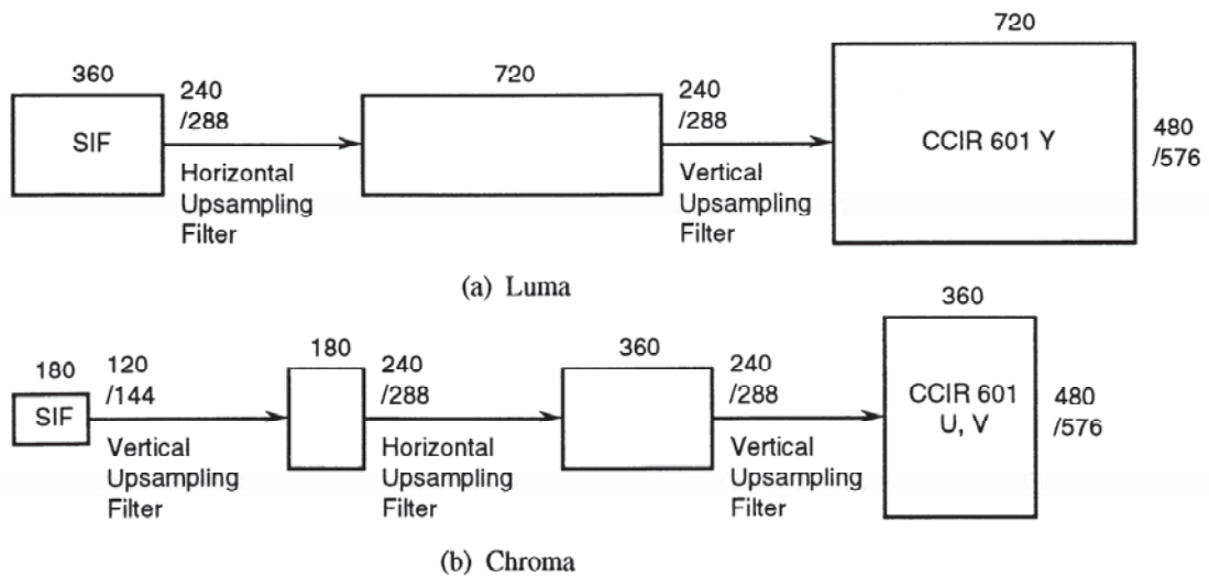
Figure D.41 -- Simplified decoder block diagram
