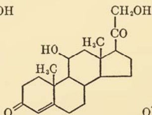
Corticosterone, C_{21}H_{30}O_4
