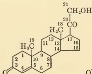
11-Desoxycorticosterone, C_{21}H_{30}O_3
