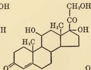
17-Hydroxycorticosterone, C_{21}H_{30}O_5
