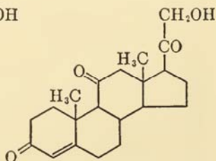
11-Dehydrocorticosterone, C_{21}H_{28}O_4
