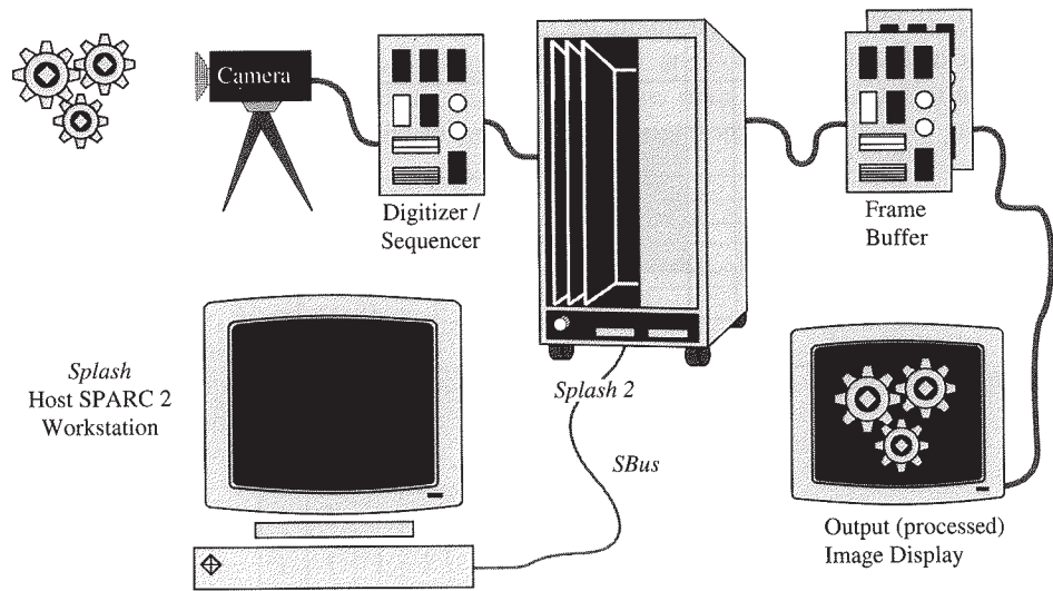
FIGURE 11.1 Components in the VTSPLASH Laboratory System
