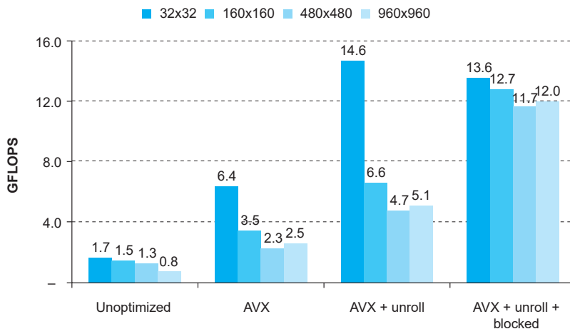
FIGURE 5.49 Performance of four versions of DGEMM from matrix dimensions 32x32 to 960x960. The fully optimized code for largest matrix is almost 15 times as fast as the unoptimized version in Figure 3.21 in Chapter 3.
