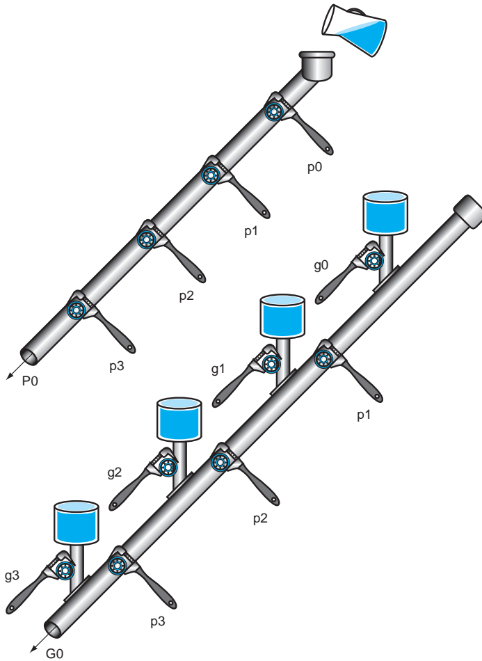
FIGURE B.6.2 A plumbing analogy for the next-level carry-lookahead signals P0 and G0 . P0 is open only if all four propagates ( p_i ) are open, while water flows in G0 only if at least one generate ( g_i ) is open and all the propagates downstream from that generate are open.
