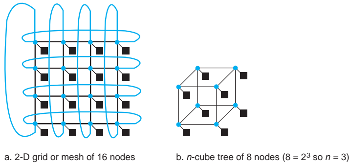
FIGURE 6.14 Network topologies that have appeared in commercial parallel processors. The colored circles represent switches and the black squares represent processor-memory nodes. Even though a switch has many links, generally only one goes to the processor. The Boolean n -cube topology is an n -dimensional interconnect with 2n nodes, requiring n links per switch (plus one for the processor) and thus n nearest-neighbor nodes. Frequently, these basic topologies have been supplemented with extra arcs to improve performance and reliability.
