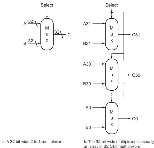
FIGURE B.3.6 A multiplexor is arrayed 32 times to perform a selection between two 32-bit inputs. Note that there is still only one data selection signal used for all 32 1-bit multiplexors.
