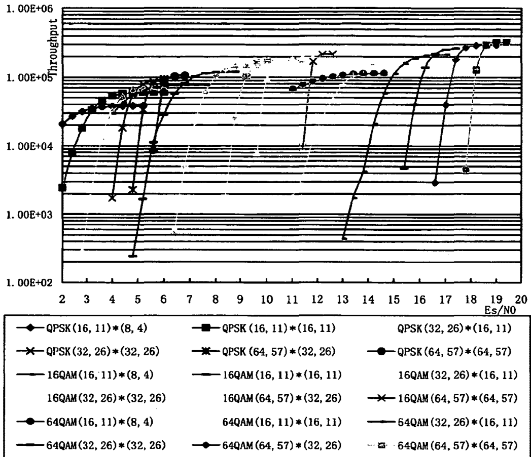
Throughput, in AWGN Channel, TPC+AMC
