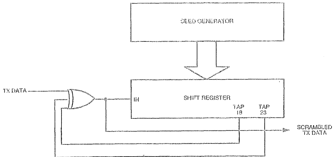
Fig 11-10 Scrambler
