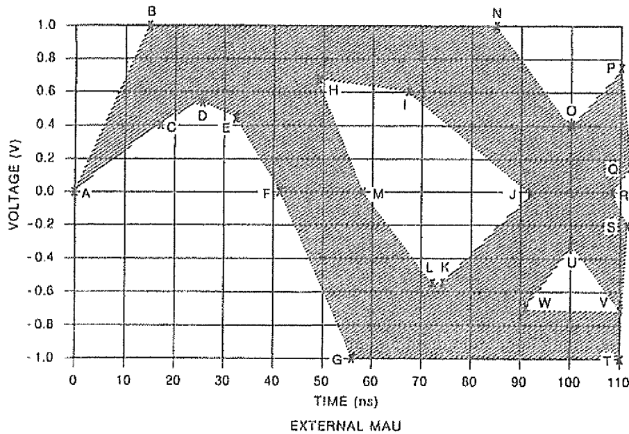
Fig 14-9 Voltage Template
