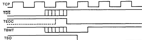
TRANSMITTER START-UP
