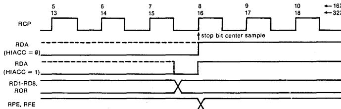
RECEIVER TIMING DETAIL
