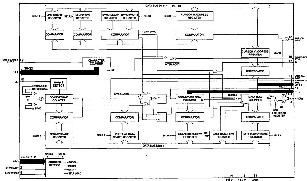
BLOCK DIAGRAM
