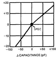
Typical \Delta Output Delay Versus \Delta Capacitance (pF)
