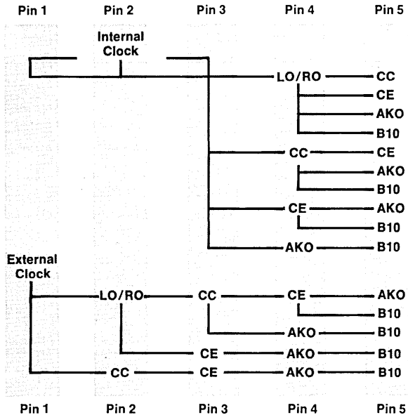
OPTION SELECTION/PIN ASSIGNMENT FIGURE 1
