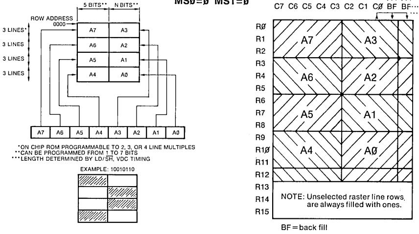
FIGURE 1 WIDE GRAPHICS MODE MS0=0 MS1=0
