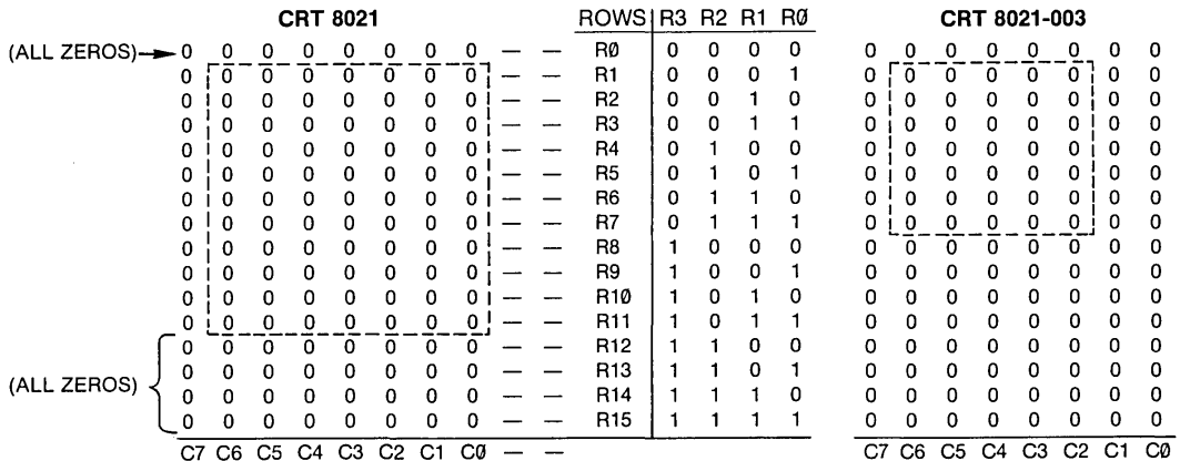
FIGURE 2 TYPICAL CHARACTER MODE BLOCK FORMATS
