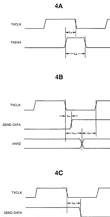
TRANSMITTER TIMING FIGURE 4
