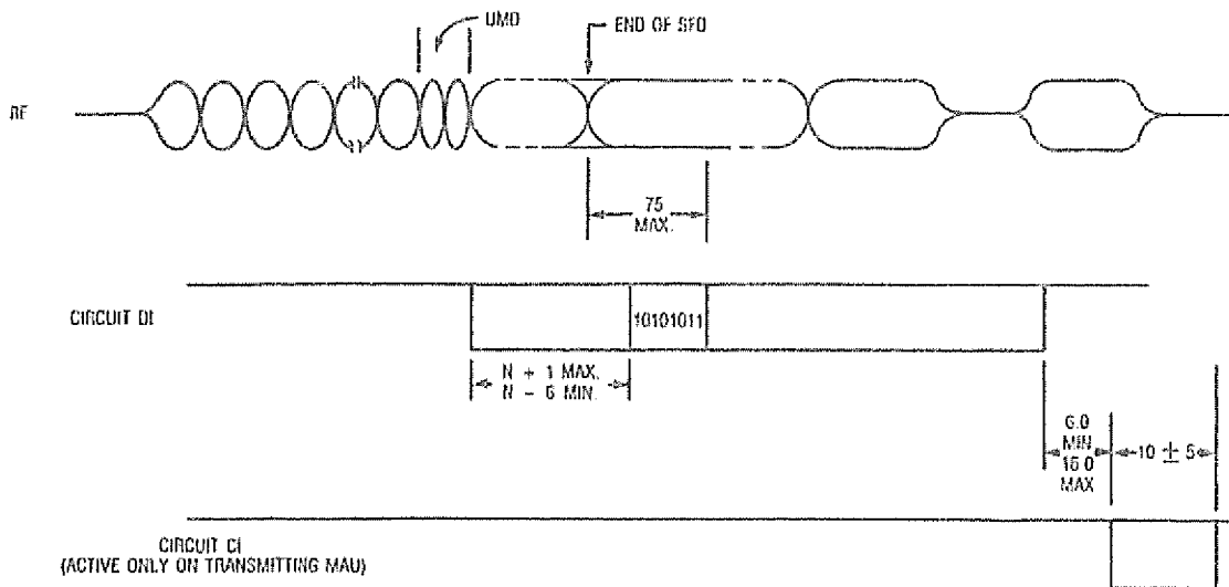
Fig 11-13 No Collision Timing Diagram (Coax to AUI)
