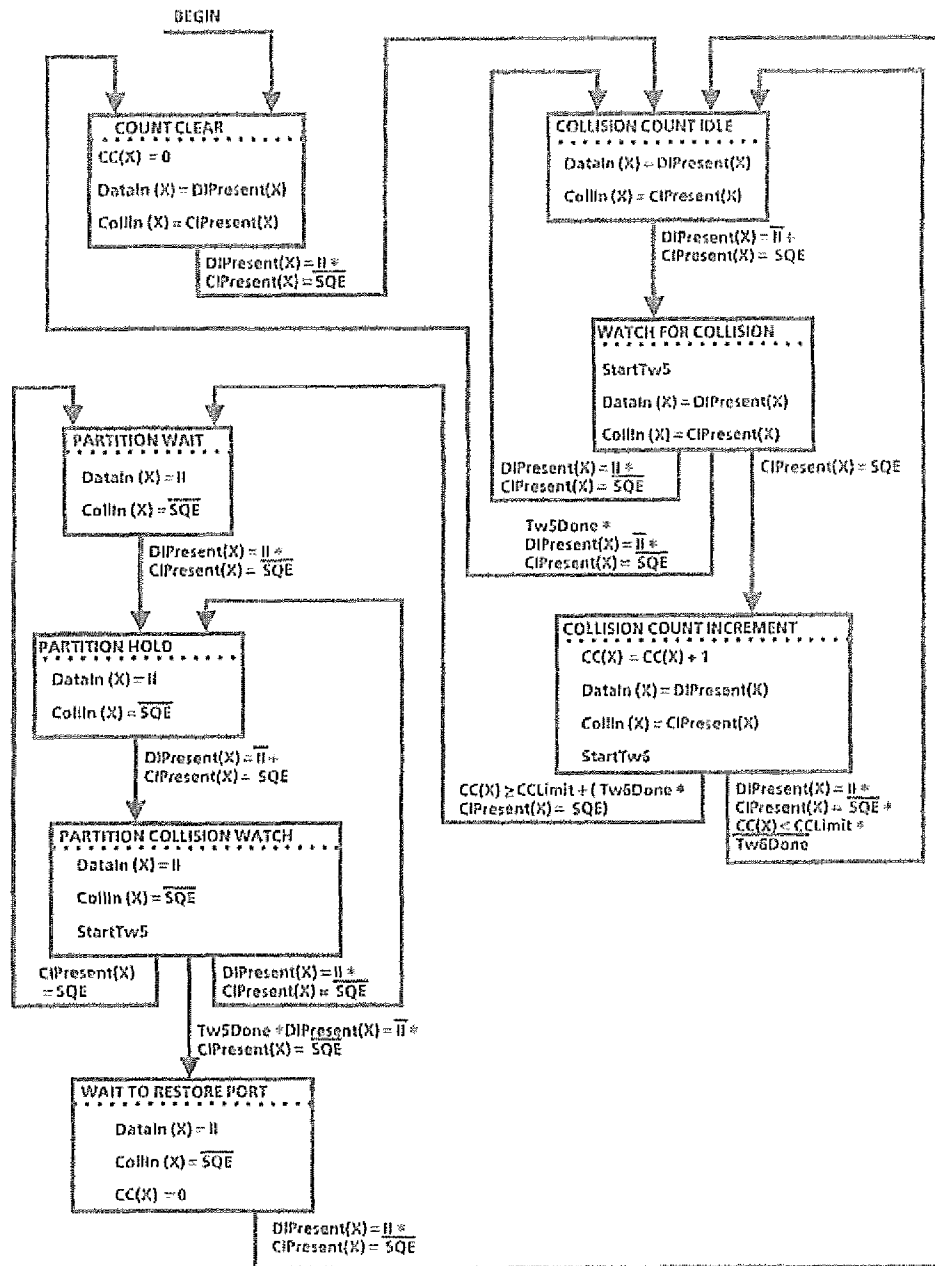
Fig 9-6 Partitioning State Diagram for Port X
