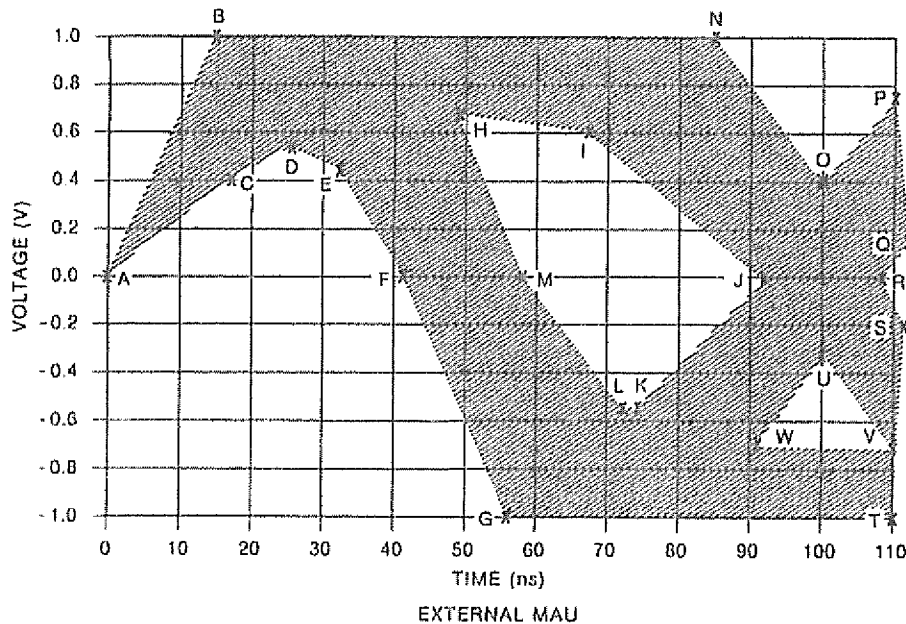
Fig 14-9 Voltage Template
