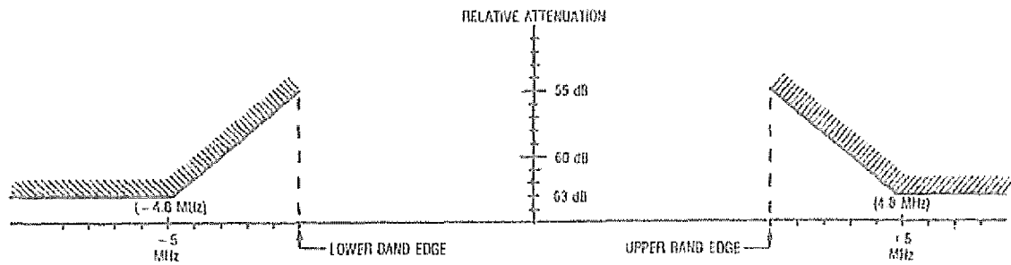
Fig 11-7 Spectrum Mask for RF Data Signal
