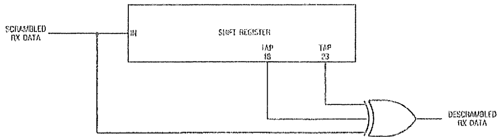
Fig 11-12 Descrambler
