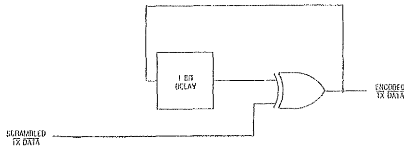
Fig 11-11 Differential Encoder
