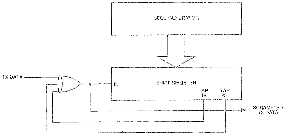
Fig 11-10 Scrambler
