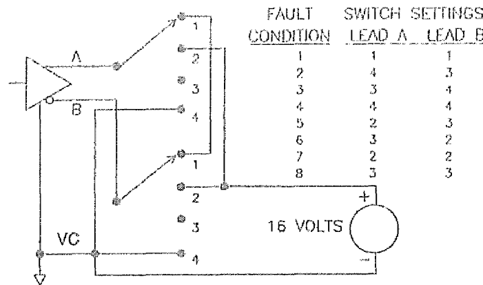
Fig 7-14 Driver Fault Conditions
