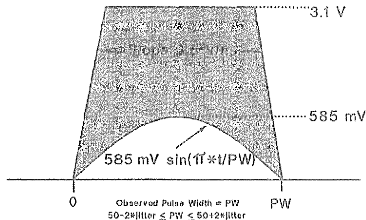
Fig 14-16 Receiver Differential Input Voltage—Narrow Pulse
