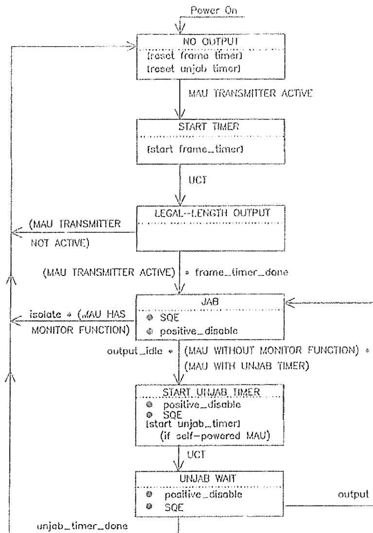
Fig 8-4 Jabber Function
