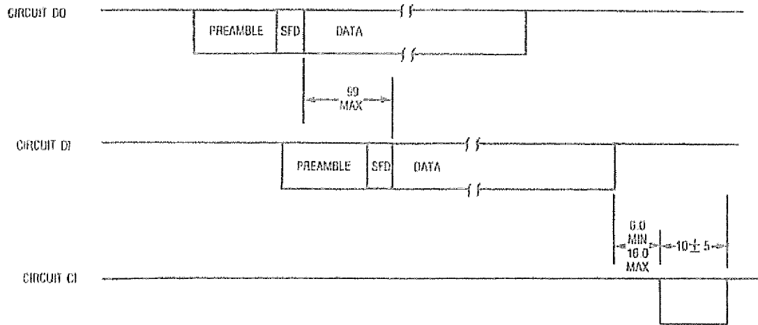
Fig 11-16 Timing at AUI for Zero-Length Coax
