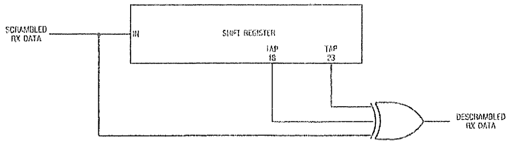
Fig 11-12 Descrambler
