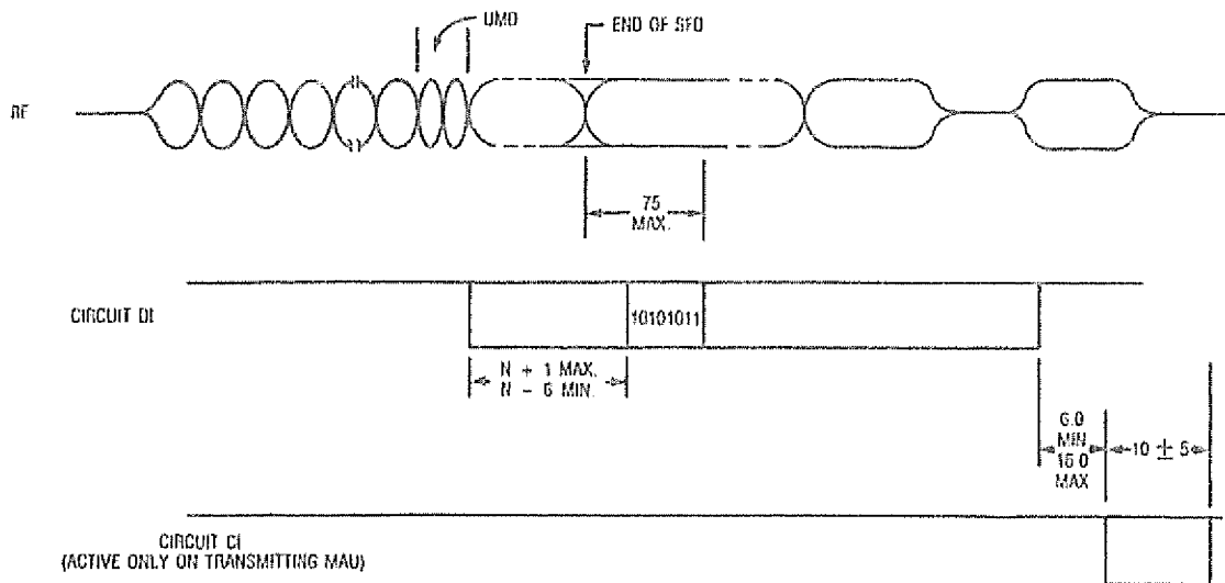
Fig 11-13 No Collision Timing Diagram (Coax to AUI)
