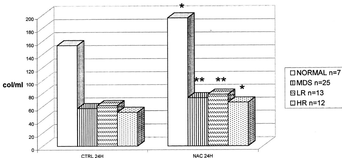
Fig. 2. Effect of NAC on clonogenic activity (CFU-GM) after 24 h of liquid culture. * P < 0.05 , ** P < 0.01 versus controls.
