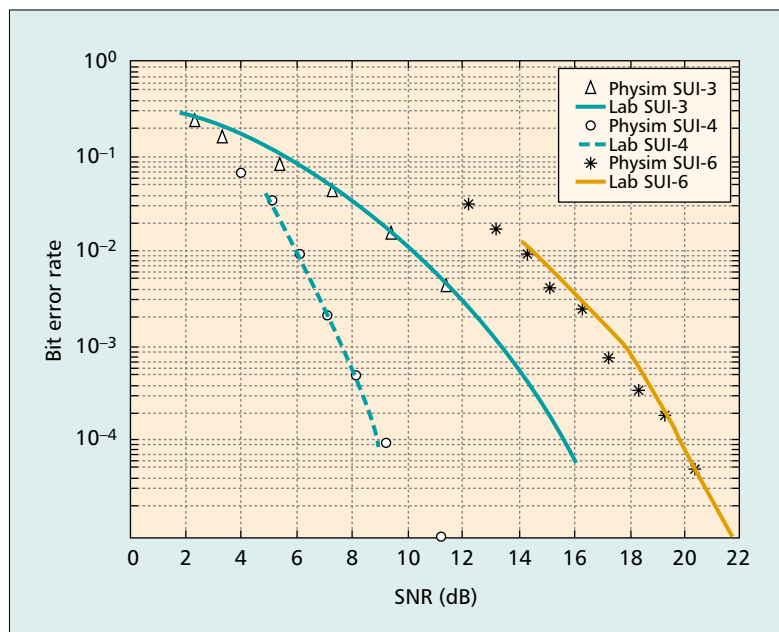
■ Figure 3. Sample BER vs. SNR for several SUI models and link modes.
