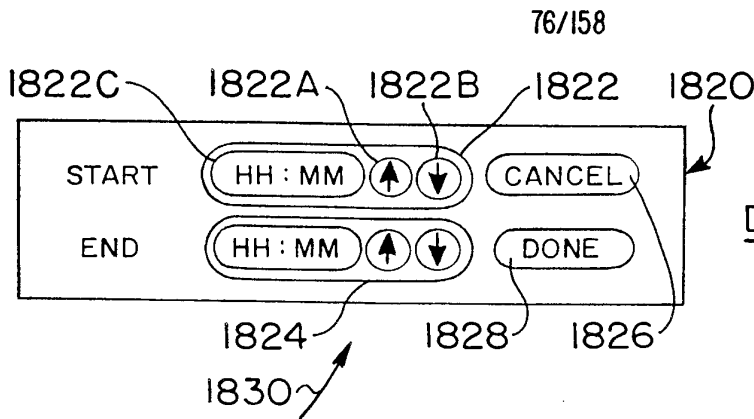
FIG. 85 SCHEDULE QUEUE
