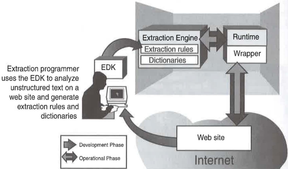
Figure 29-3 The extractor development process
