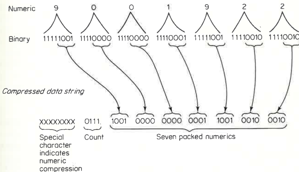
Figure 2.17 Half-byte encoding example. For 8-level character transmission, a multiple of 8 bits of compressed data is transferred. Thus, a half-byte counter with an even number of packed characters will require 4 trailing null bits
