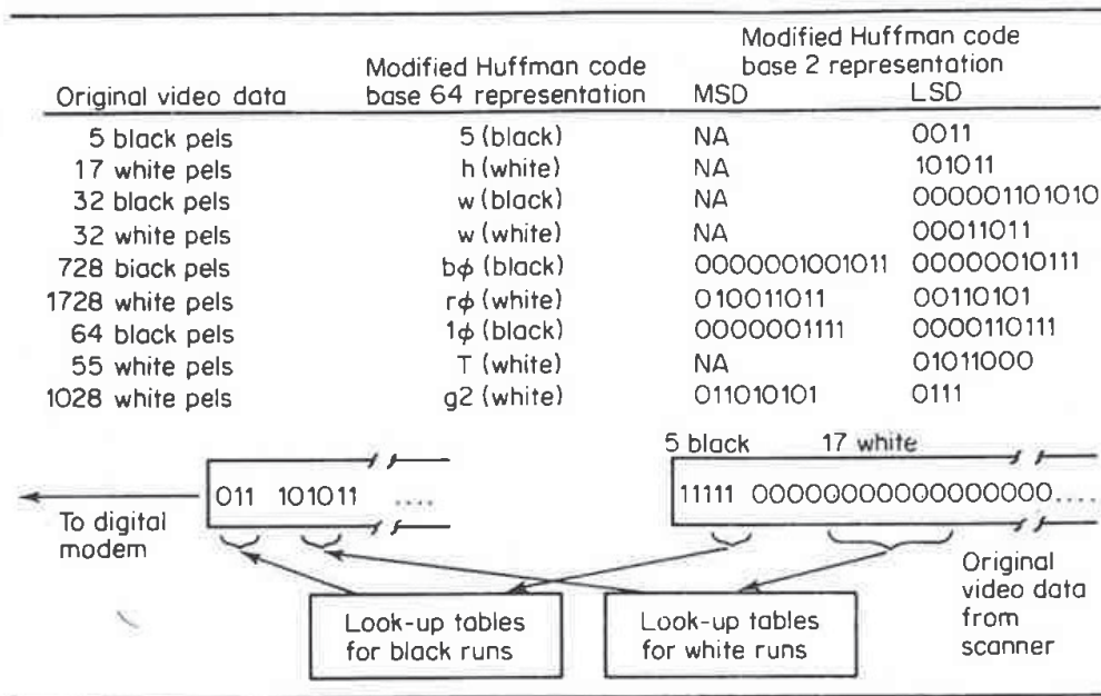
Figure 2.50 Encoding using the modified Huffman code. By a sequence of tabular references for black and white runs the modified Huffman code is constructed
