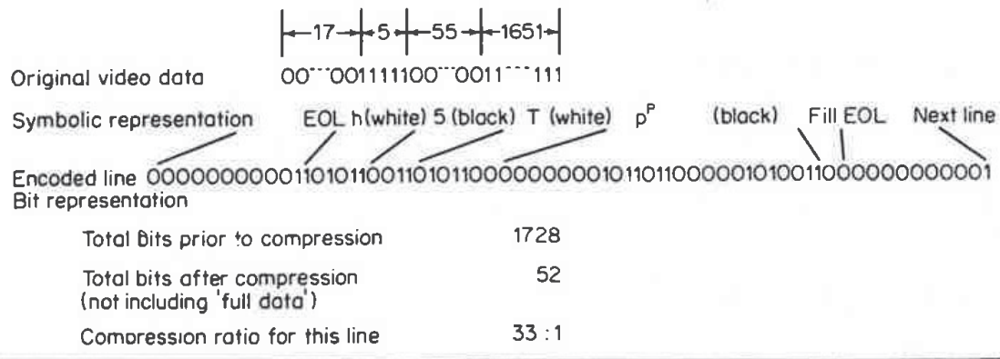
Figure 2.51 Rules define line format. To denote the beginning and end of each scan line an end-of-line code (EOL) is employed.
