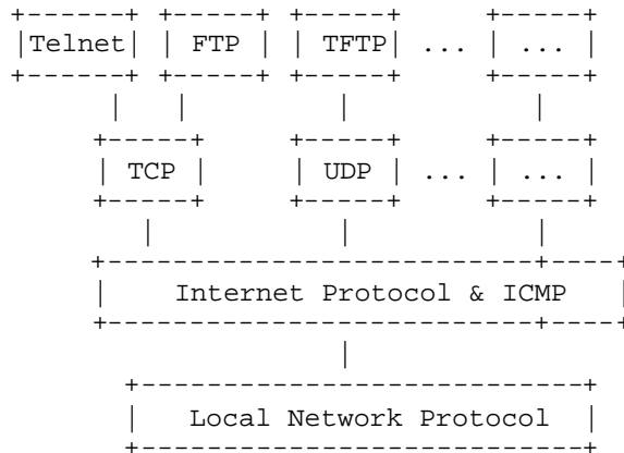
Protocol Relationships
