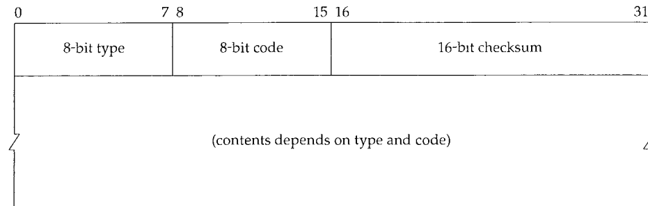
Figure 6.2 ICMP message.
