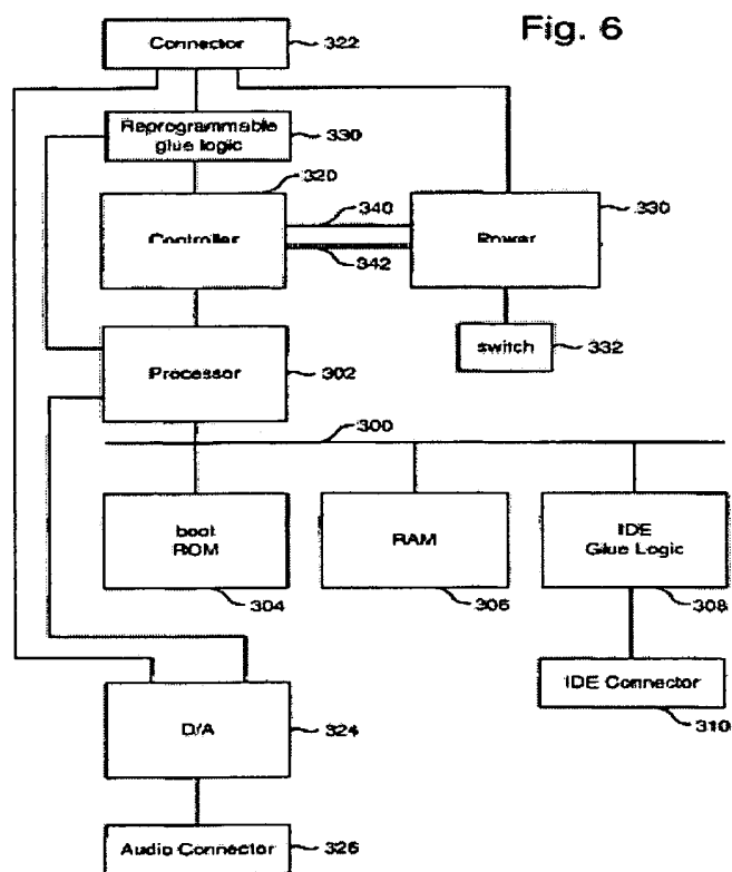
Figure 6 is a block diagram of one embodiment of the components within music server 102 shown in Figure 1. Ex. 1103, 5:23–24. Controller 320’s generating a signal to convey to a car stereo that processor 302 is connected
