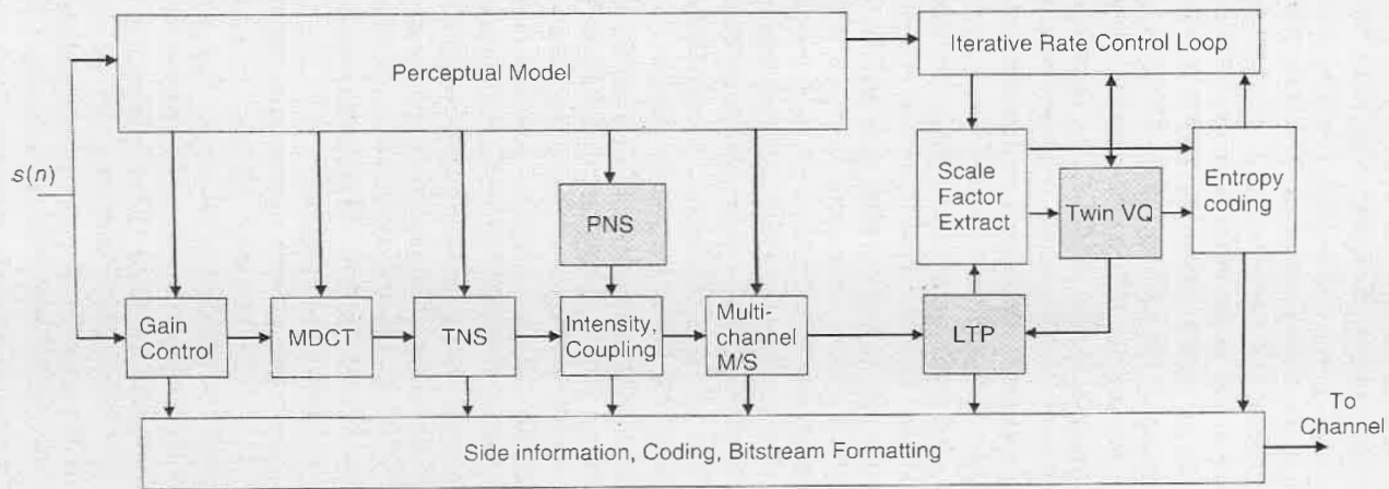
Figure 10.14. MPEG-4 GA coder.
