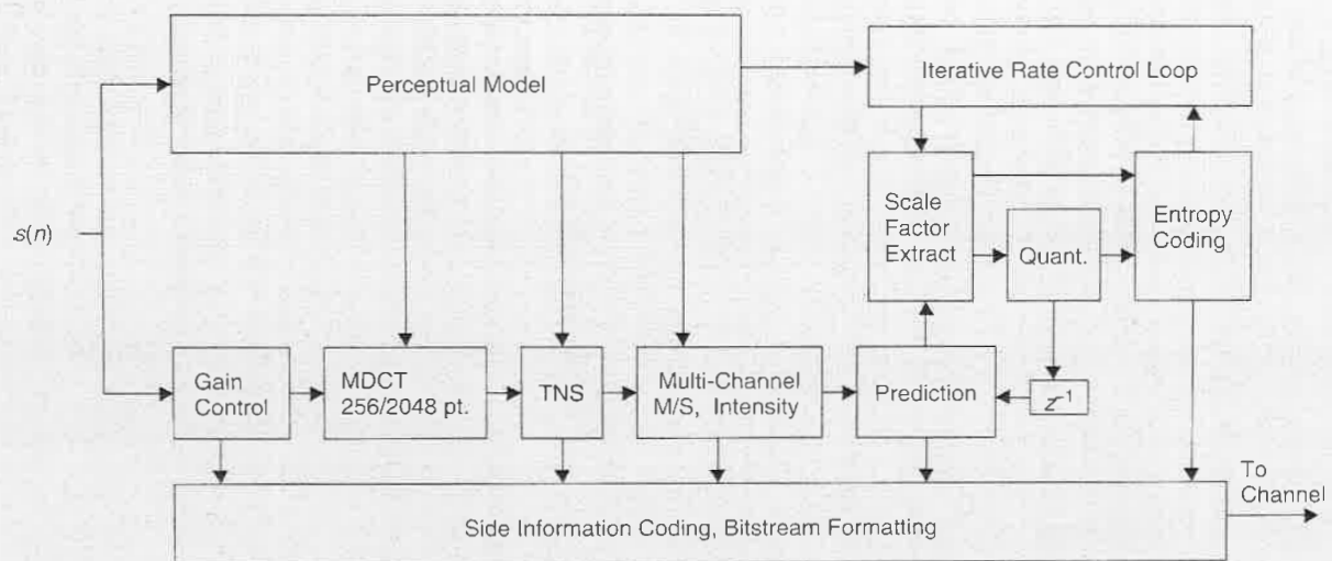
Figure 10.10. ISO/IEC IS13818-7 (MPEG-2 NBC/AAC) encoder ([Bosi96]).
