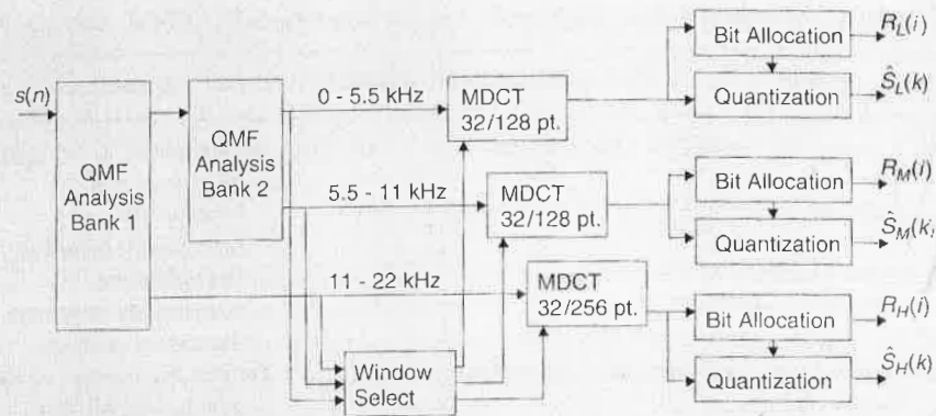
Figure 10.24. Sony ATRAC (embedded in MiniDisc, SDDS).
