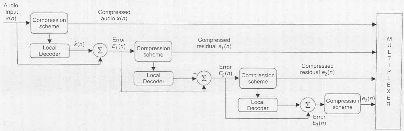
Figure 10.16. MPEG-4 scalable audio coding.
