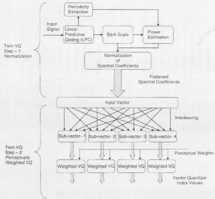
Figure 10.15. Twin VQ scheme in MPEG-4 GA coder.
