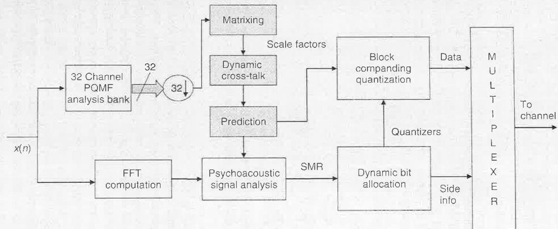
Figure 10.9. ISO/MPEG-2 BC/LSF audio (layer I/II) encoder algorithm.
