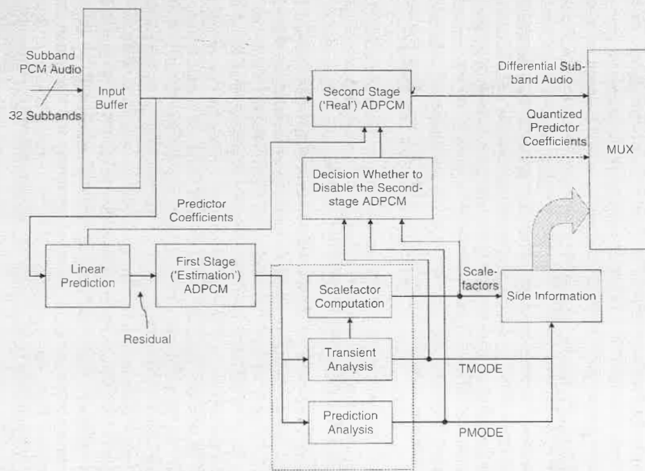
Figure 10.32. Differential subband (ADPCM) coding in the DTS-CA encoder.
