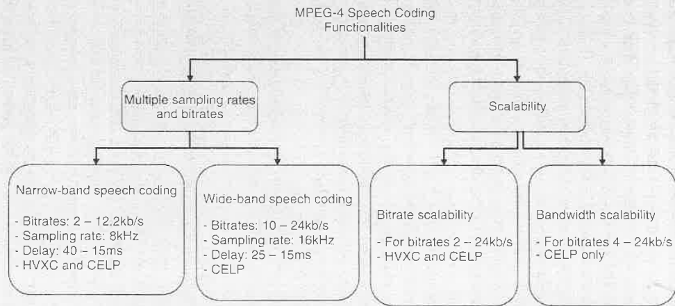
Figure 10.17. MPEG-4 speech coder functionalities.
