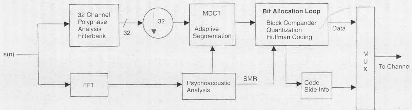
Figure 10.7. ISO/MPEG-1 layer III encoder.
