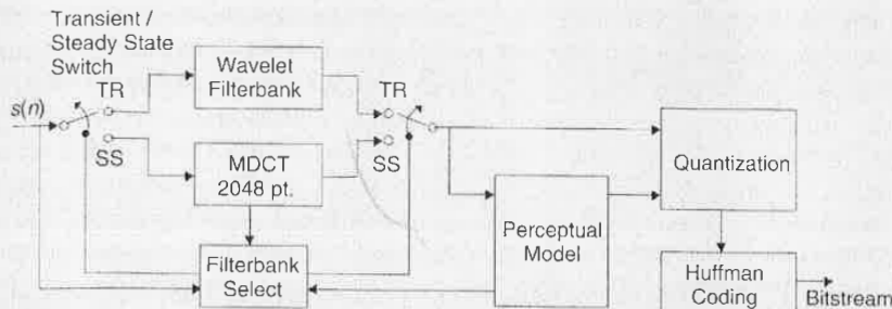
Figure 10.26. Lucent Technologies Enhanced Perceptual Audio Coder (EPAC).
