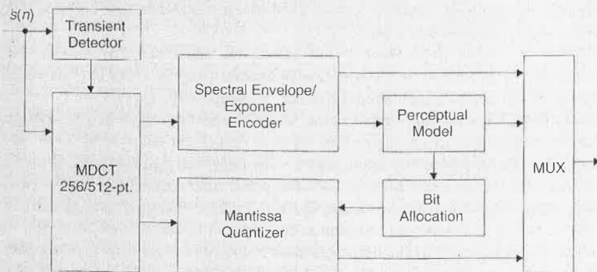
Figure 10.27. Dolby Laboratories AC-3 encoder.
