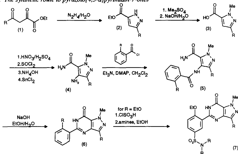
Figure 6. The synthetic route to pyrazolo[4,3-d]pyrimidin-7-ones
