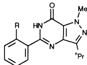
Figure 4 The effect of the 2'-substituent on PDE 5 inhibitory activity. IC_{50} values are in nanomolar unless otherwise stated, and are the mean values of at least 2 determinations. ND = not determined.
