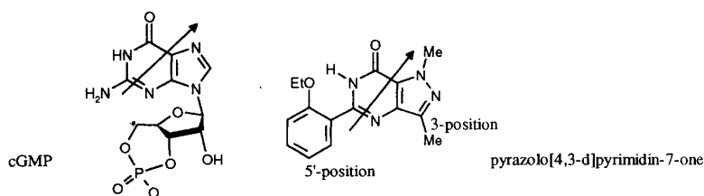
Figure 2 Modelling studies on cGMP and a pyrazolo[4,3-d]pyrimidin-7-one
