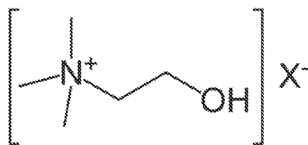
Figure 2. Choline Structure
