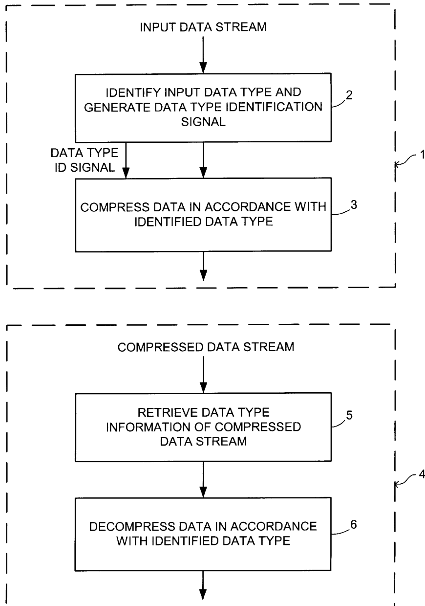
FIG. 1 PRIOR ART
