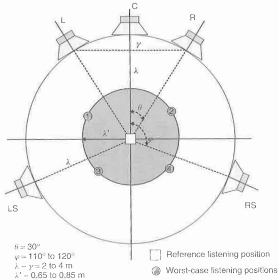
Figure 10.5. A typical 3/2-channel configuration described in the ITU-R BS.775-1 standard [ITU-R94c]. L: left, C: center, R: right, LS: left surround, and RS: right surround loud speakers. Note that the above figure is not according to a scale.
