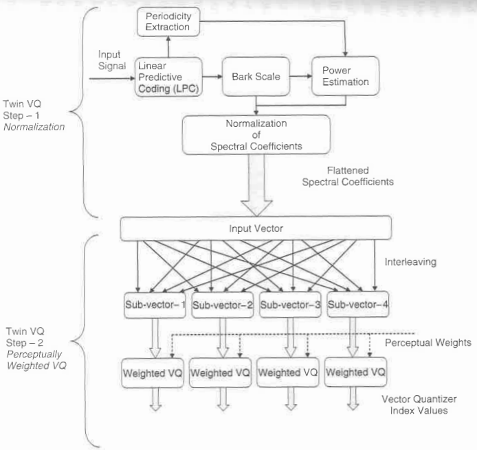
Figure 10.15. Twin VQ scheme in MPEG-4 GA coder.
