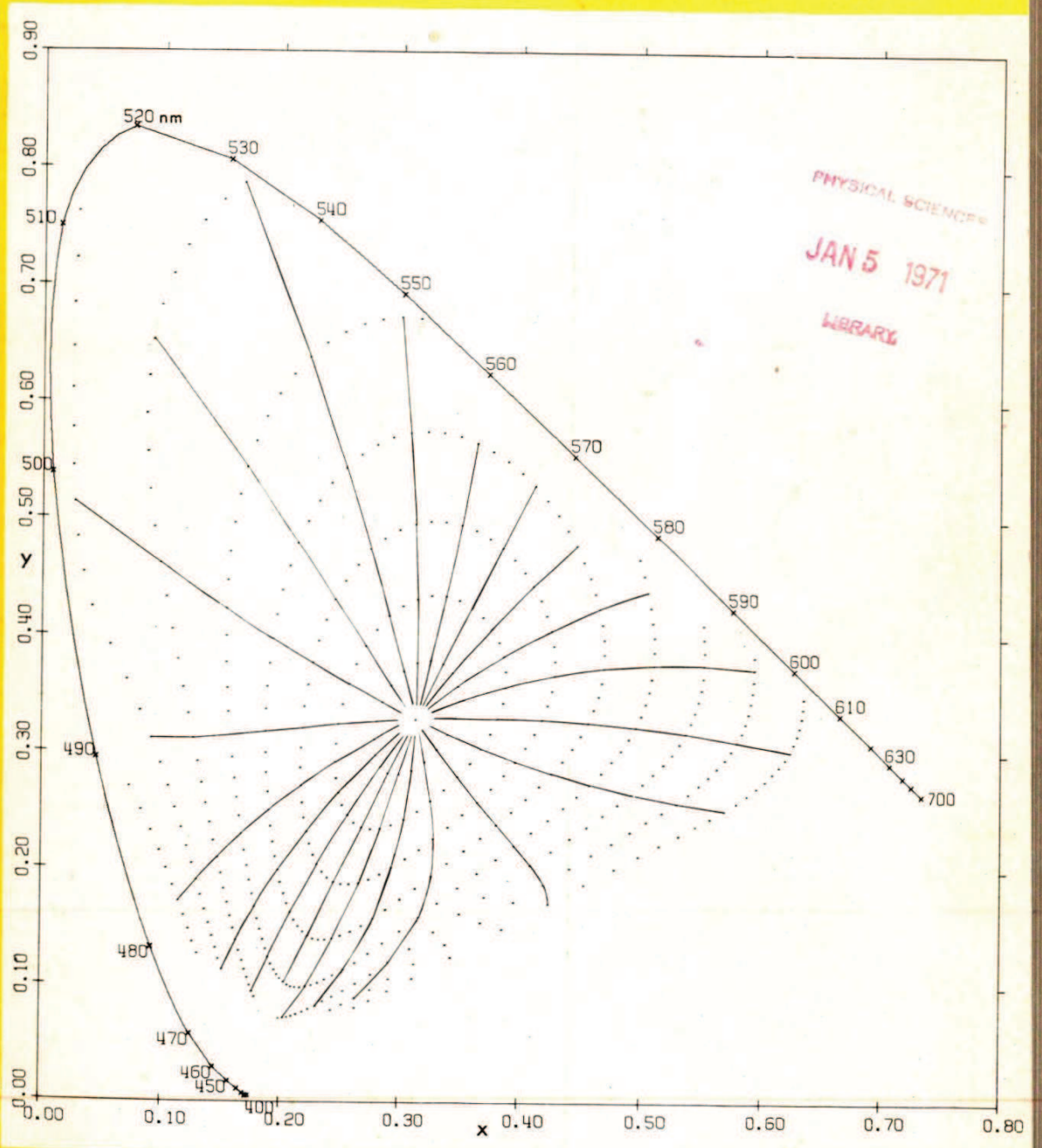
CHROMATICITY DIAGRAM
