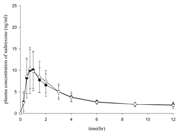
Fig. 3. Time course of the mean plasma concentration in healthy subjects after a single naltrexone 50-mg oral dose. Each point represents the mean + standard deviation. (n= 22, ●; Levia® (naltrexone 50 mg reference tablet), ○; Traxone (naltrexone 50 mg test tablet))
