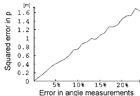
Figure 6.2: Simulation results using the algorithm Position Estimator on an input of noisy angle measurements. The squared error in the position estimate p (in meters) is shown as a function of measurement errors (in percent of the actual angle). (Reproduced and adapted with permission from [Betke and Gurvits, 1994].)
