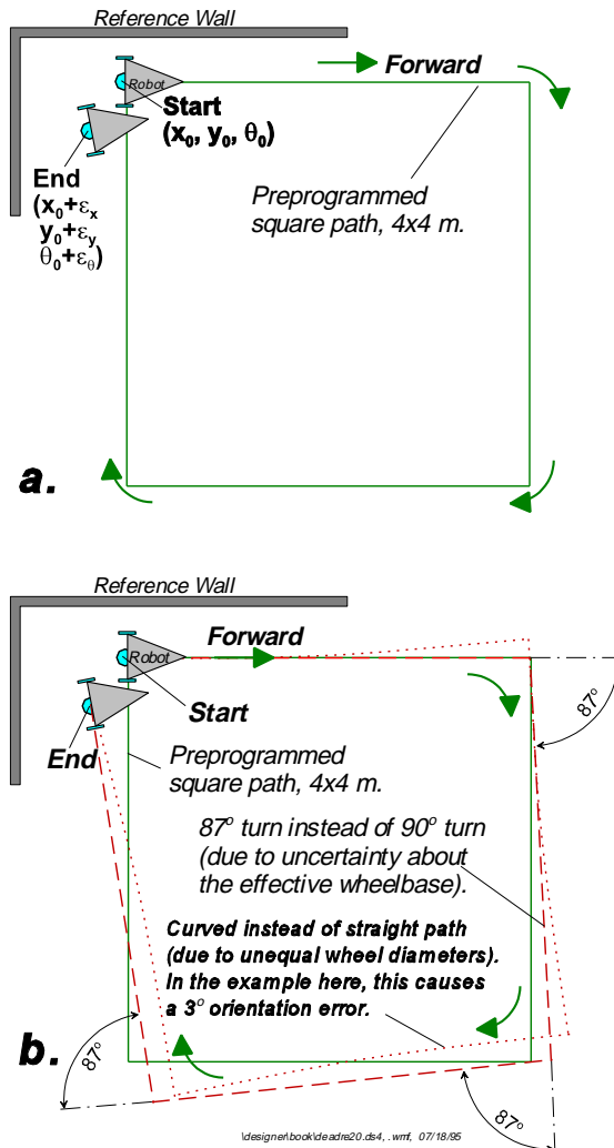
Figure 5.2: The unidirectional square path experiment. a. The nominal path. b. Either one of the two significant errors E_b or E_d can cause the same final position error.
