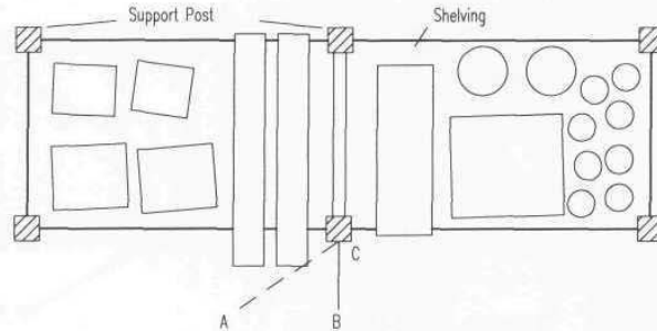
Figure 15-27. Protruding objects in the vicinity of a reflective marker will interfere with the sonar range measurements and can also occlude an off-normal optical sensor view such as along path AC.
