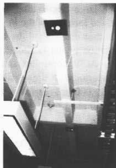
Figure 16-18. Asymmetrical retroreflective targets of known orientation and location serve as passive overhead markers for the Landmark Tracking Camera System (courtesy Georgia Institute of Technology).
