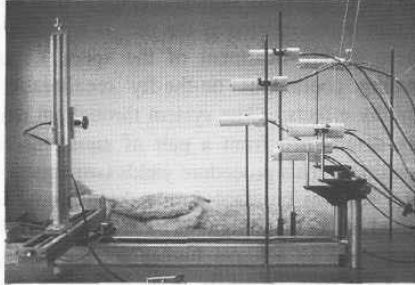
Figure 15-6. Experimental setup of the 3-D position location system showing the transmitter mounted on an X-Y-Z translation stage, and seven receivers distributed around the periphery of the work envelope (courtesy Tulane University).
