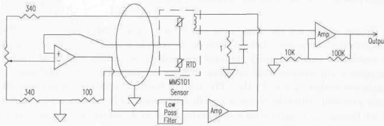
Figure 12-24. Typical application circuit for the SEI MMS101 MicroMag that provides an output voltage proportional to the cosine of magnetic azimuth for a gimbale sensor in the horizontal plane (courtesy Space Electronics, Inc.).
