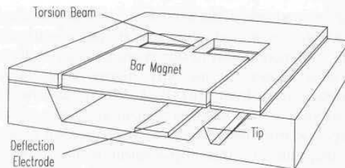
Figure 12-29. Cross-sectional diagram of the NRL/JPL micromachined magnetic-field sensor based on an electron-tunneling displacement transducer (courtesy Naval Research Lab).
