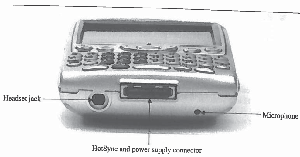
FIGURE 2-5 Components on the bottom of your Treo
