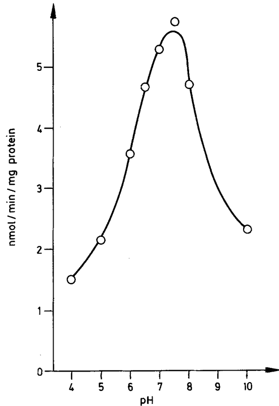
Fig. 4. pH dependence of adenosine deaminase. The homogenate was used as the enzyme source. 50 mM acetate buffer (pH 4–5), 50 mM phosphate buffer (pH 6–8), 50 mM borate-NaOH buffer (pH 9–10) were used
