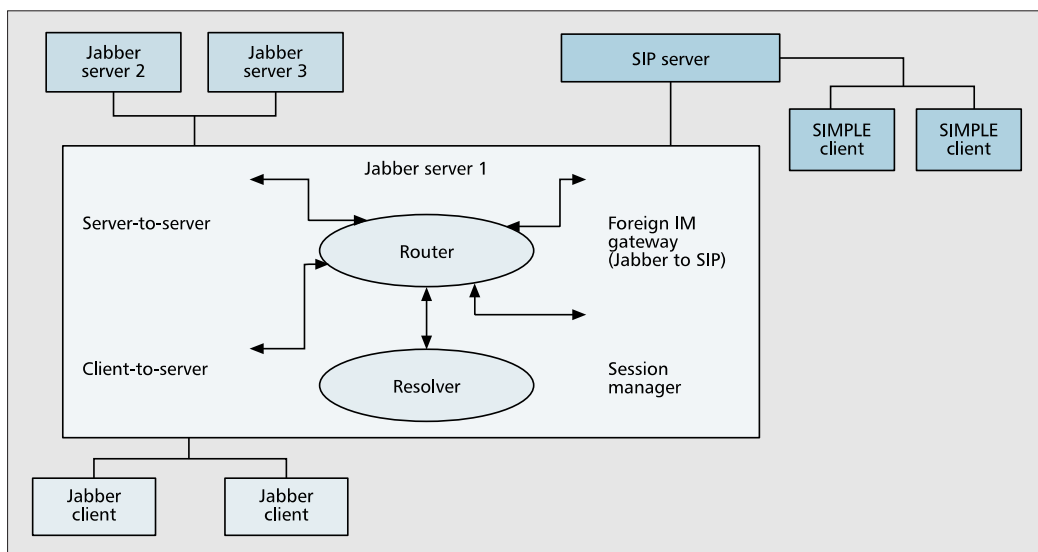
Figure 3. Jabber architecture.
