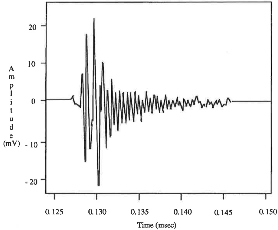
Figure 39 – Test Impulse #1
