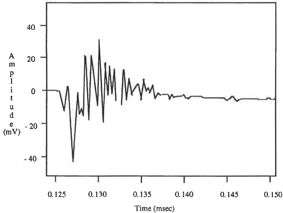
Figure 40 – Test Impulse #2
