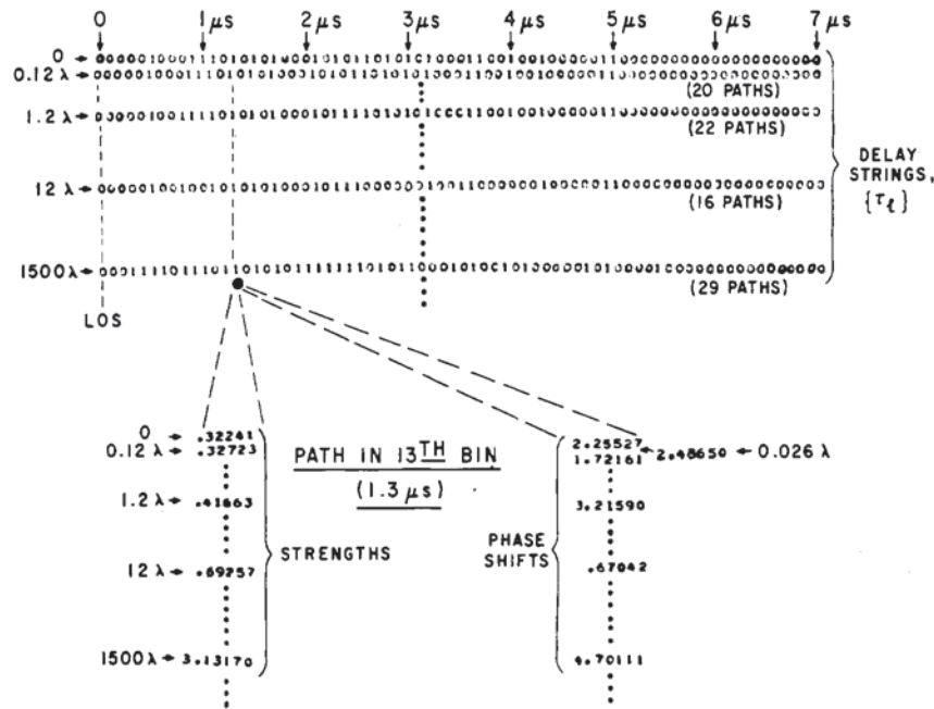
Fig. 25. Typical \{\tau_l\} strings and a_k and \theta_k values generated for L-band, using SURP.
