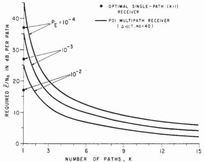
Fig. 22. Required \bar{E}/N_0 per path for DPSK/PDI system: K independent, Rayleigh-fading paths.
