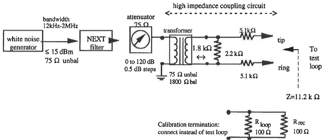
Figure 42 – High impedance crosstalk injection circuit
