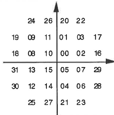
Figure 16 – Constellation labels for b = 5
