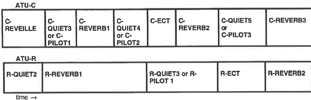
Figure 31 – Timing diagram of transceiver training (12.4-12.5)
