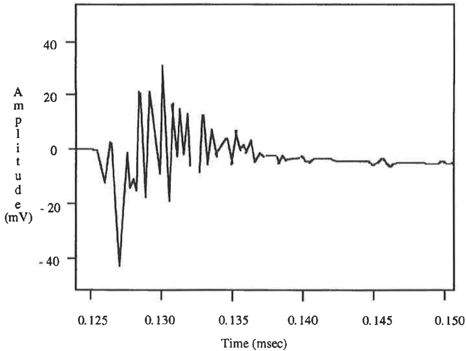
Figure 40 – Test Impulse #2
