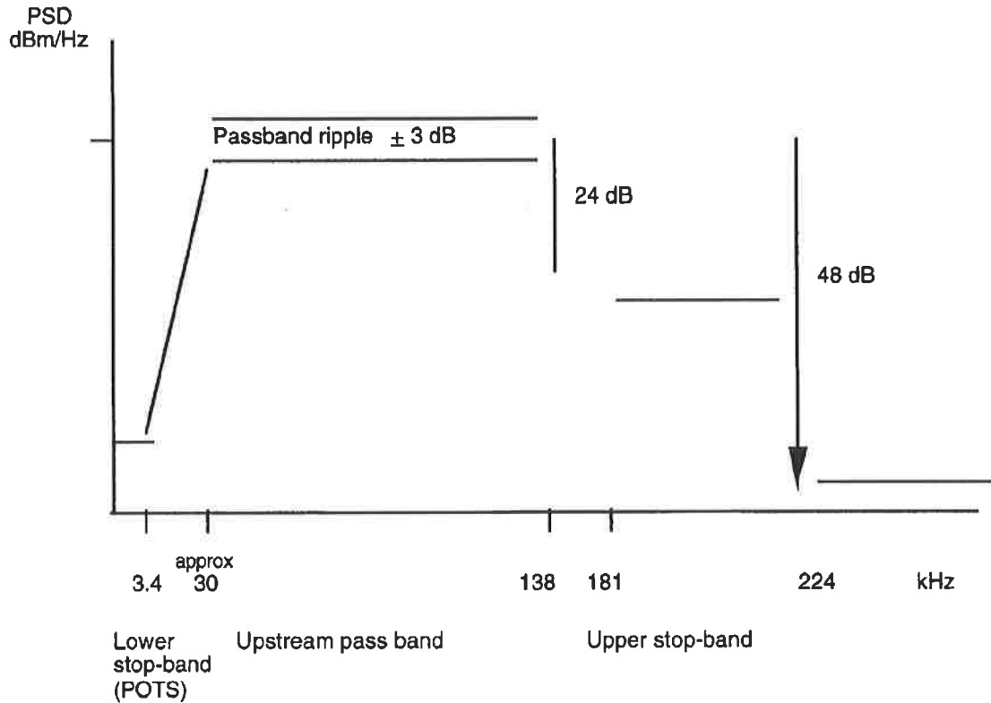
Figure 22 – ATU-R transmitter PSD mask
