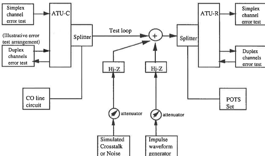
Figure 41 – Laboratory test setup for measuring performance margins
