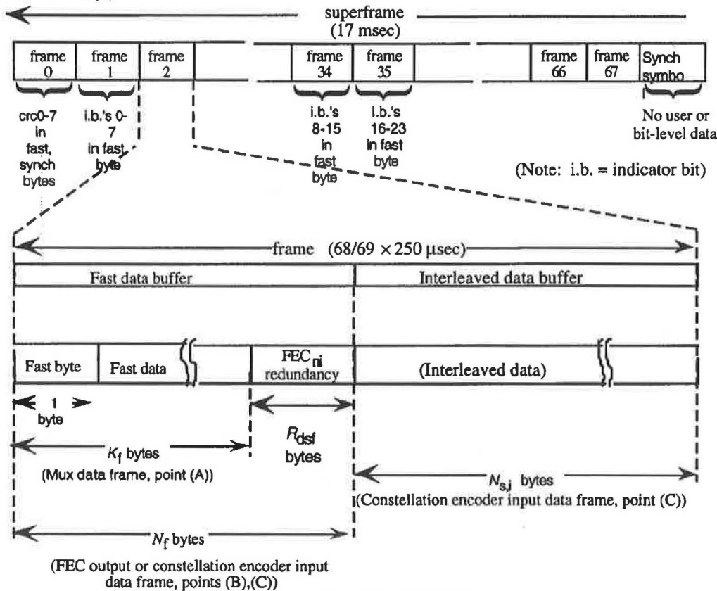
Figure 5 – ADSL superframe structure – ATU-C transmitter
