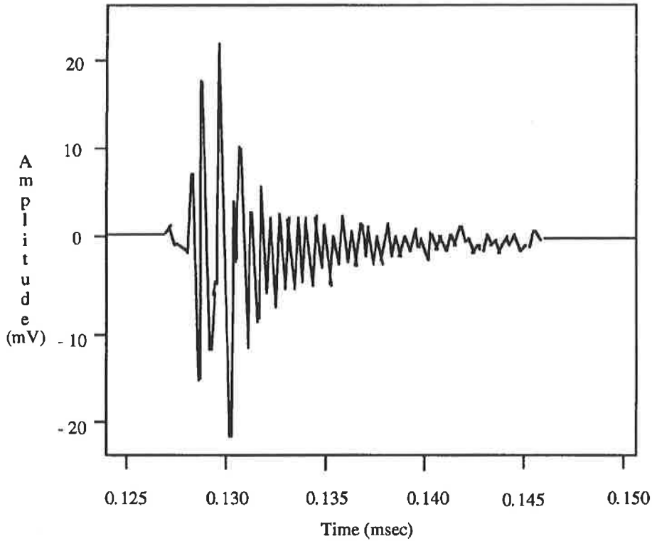
Figure 39 – Test Impulse #1
