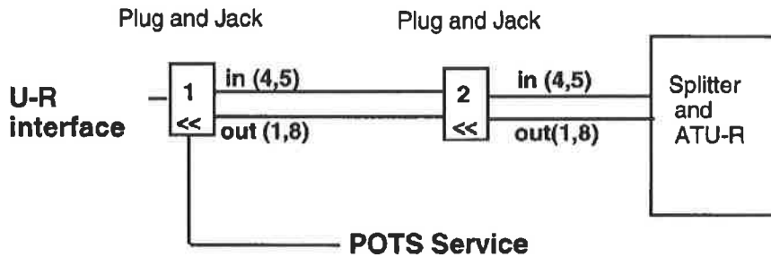
Figure 44 – Wiring for a remotely located POTS splitter/ATU-R
