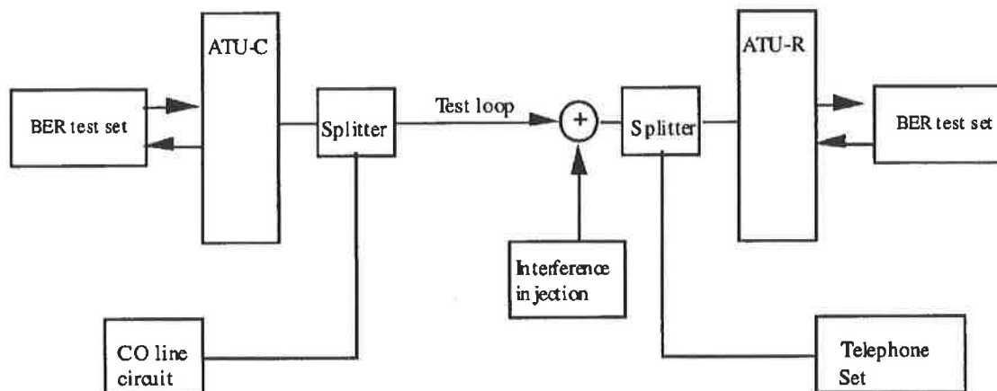
Figure 37 – Overview of test setup
