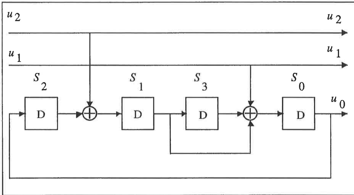
Figure 11 – Finite state machine for Wei's encoder
