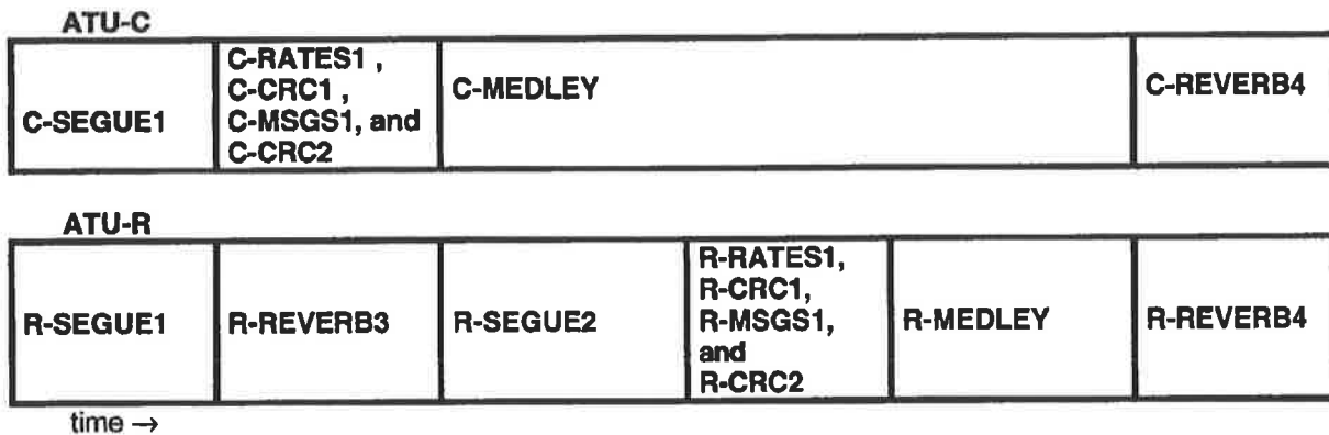
Figure 32 – Timing diagram of channel analysis (12.6-12.7)
