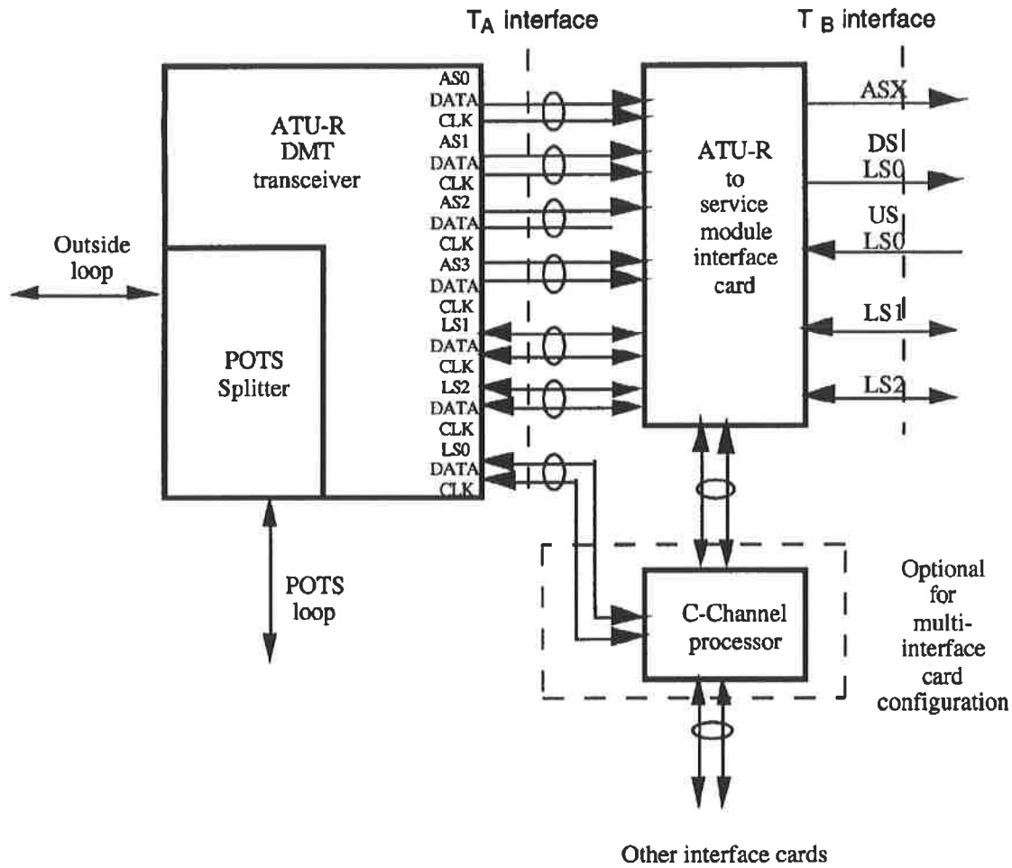
Figure 23 – ADSL entrance unit block diagram
