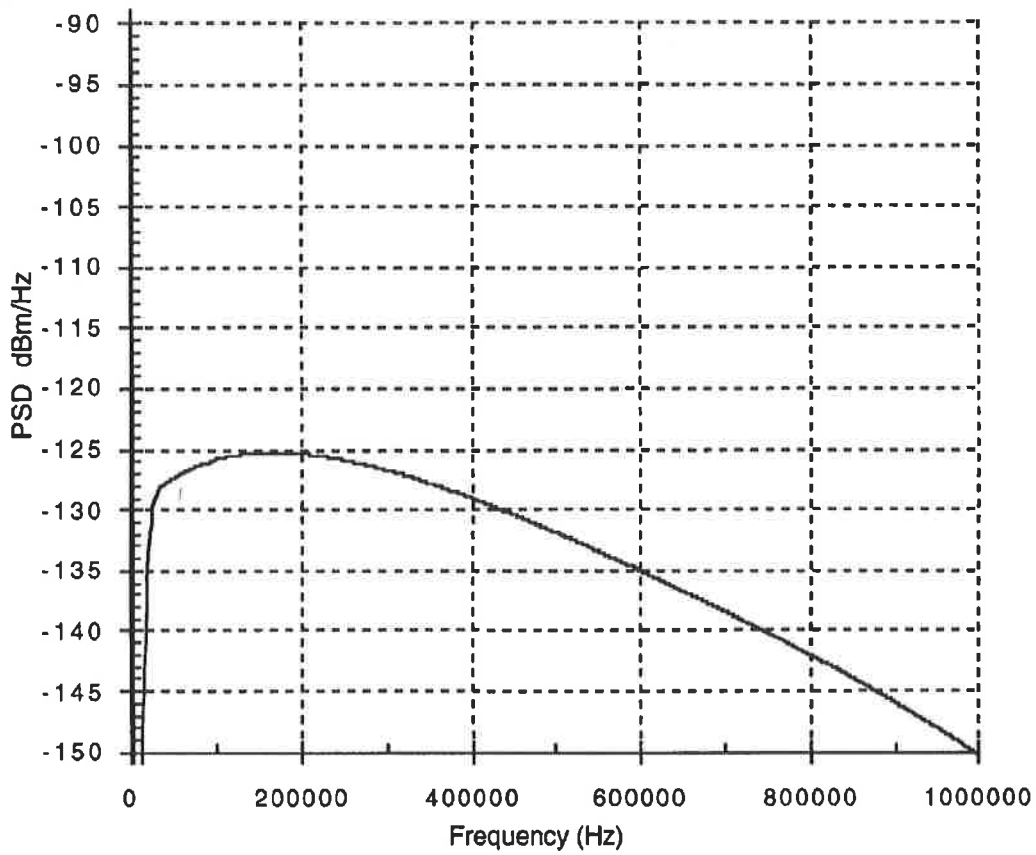
Figure B.4 – Theoretical 10-disturber ADSL FEXT
