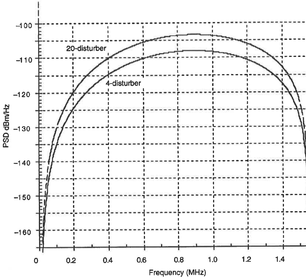
Figure B.3 – 4 and 20-disturber T1 NEXT
