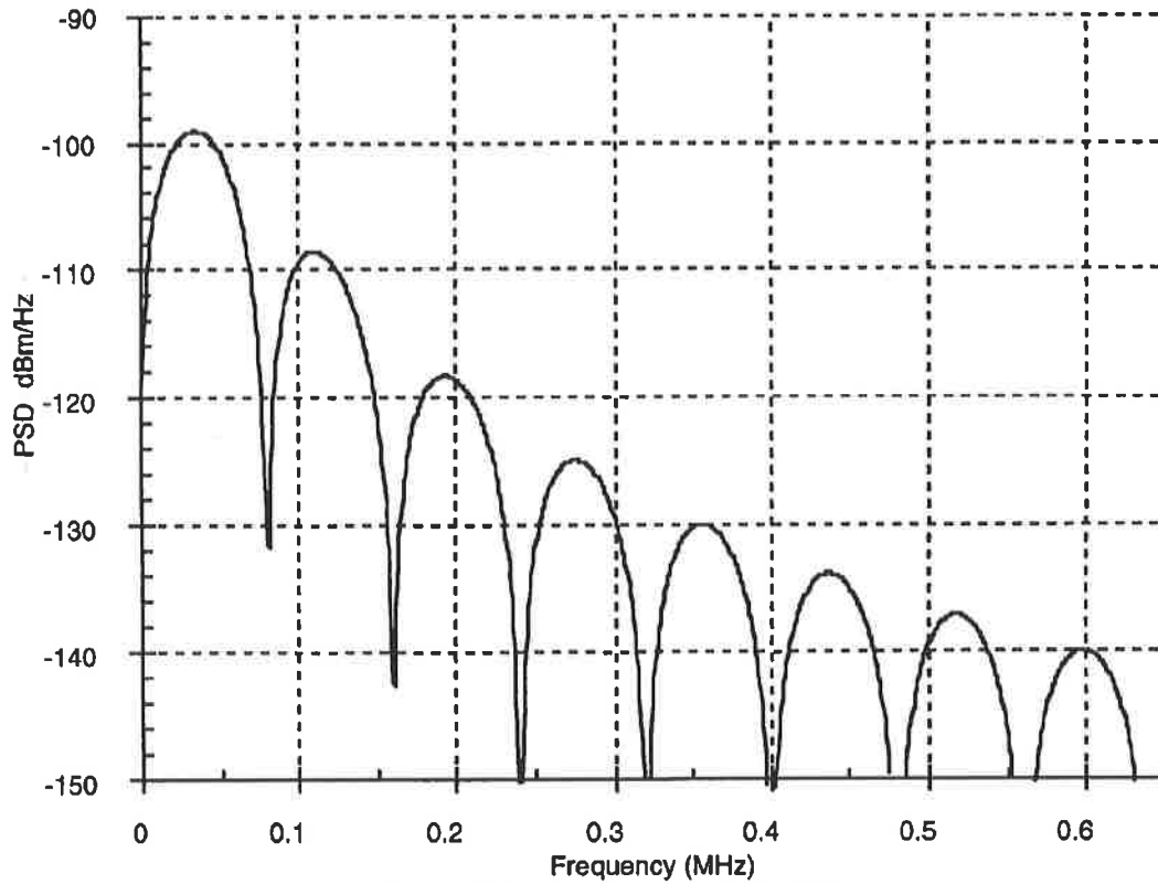
Figure B.1 – 24-disturber DSL NEXT
