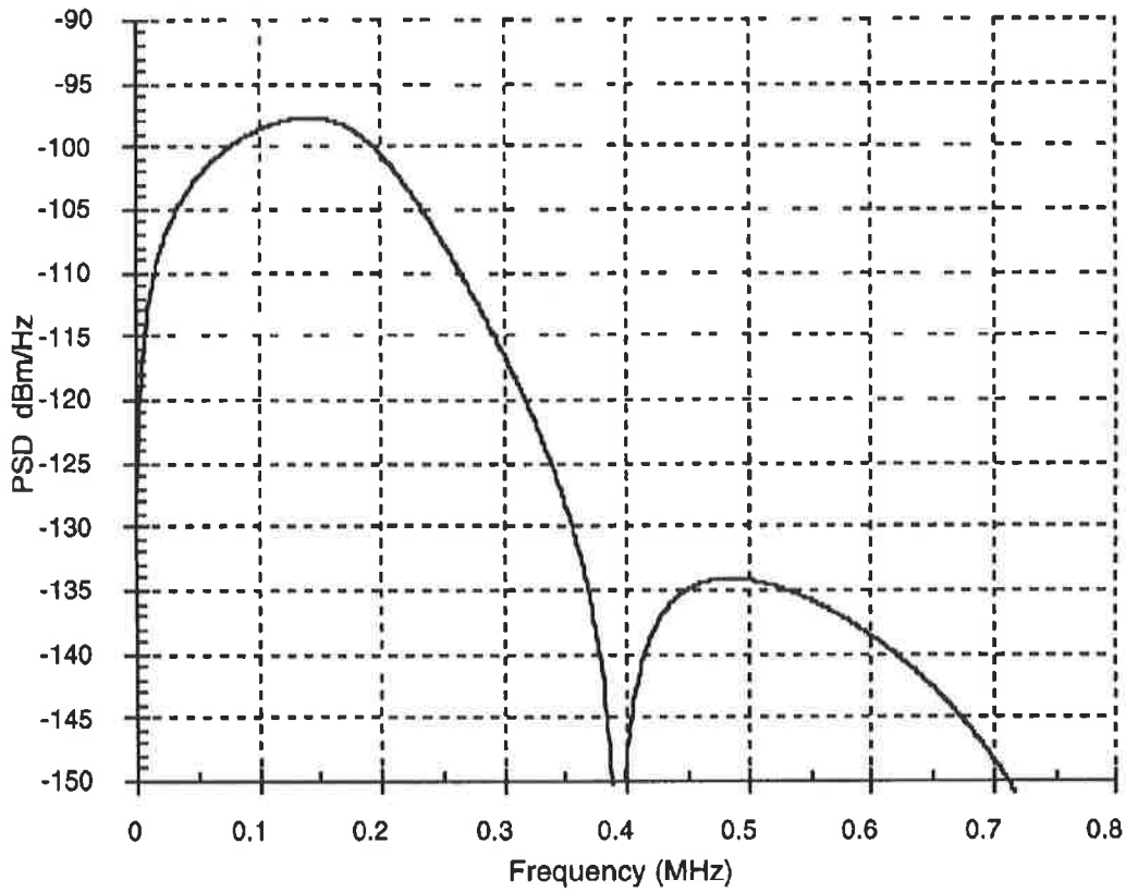
Figure B.2 – 10-disturber HDSL NEXT
