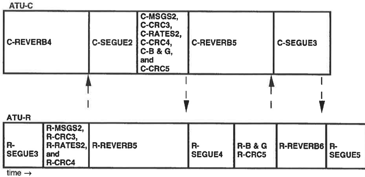
Figure 34 – Timing diagram of exchange (12.8-12.9)
