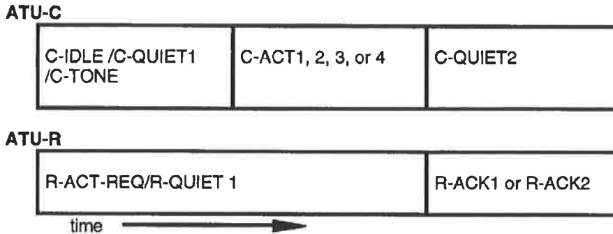
Figure 30 – Timing diagram of activation and acknowledgment (12.2-12.3)
