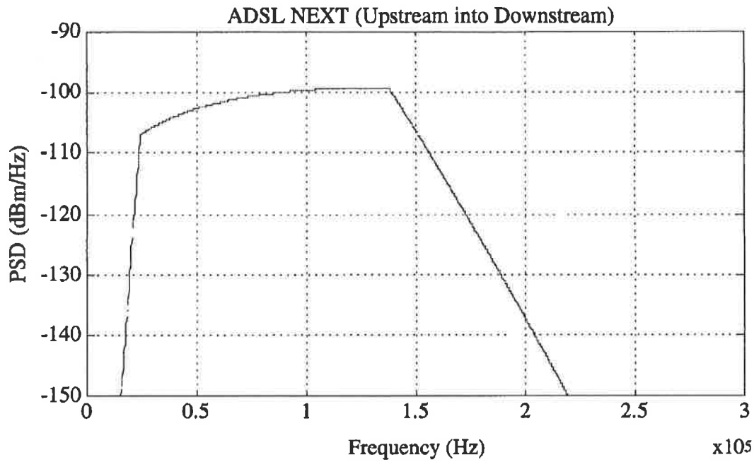
Figure B.5 – Theoretical 10-disturber ADSL NEXT
