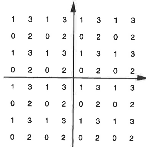
Figure 13 – Constituent 2-dimensional cosets for Wei's code
