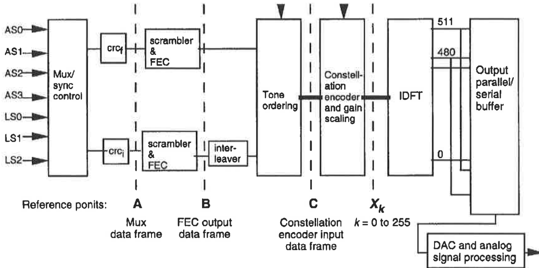
Figure 2 - ATU-C transmitter reference diagram
