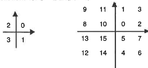
Figure 14 – Constellation labels for b = 2 and b = 4
