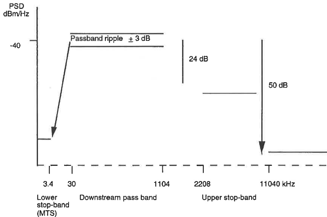
Figure 17 – ATU-C transmitter PSD mask
