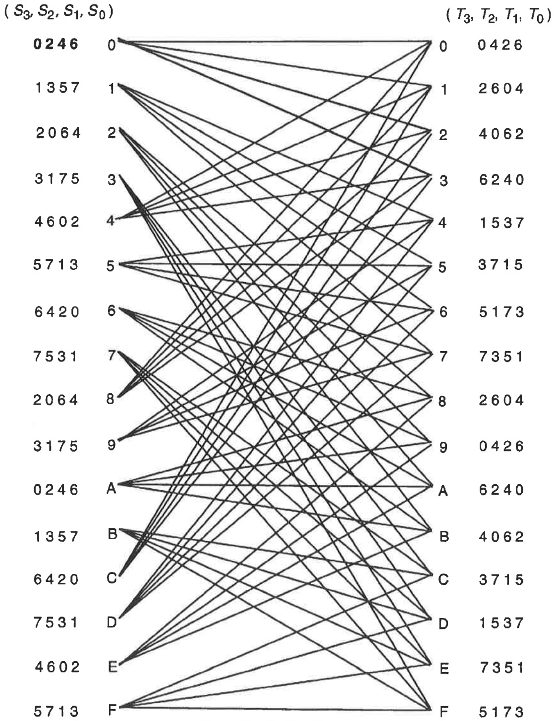
Figure 12 – Trellis diagram
