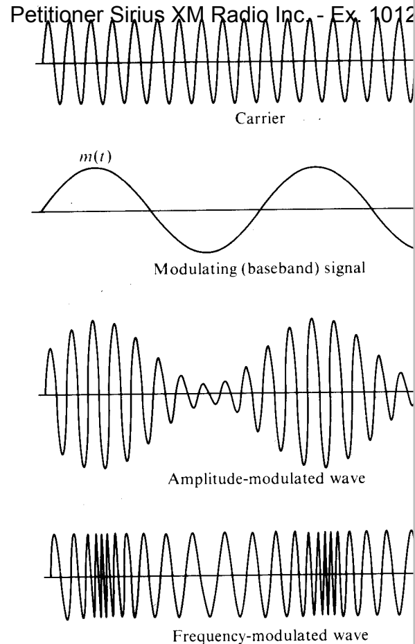
Figure 1.7 Modulation.
