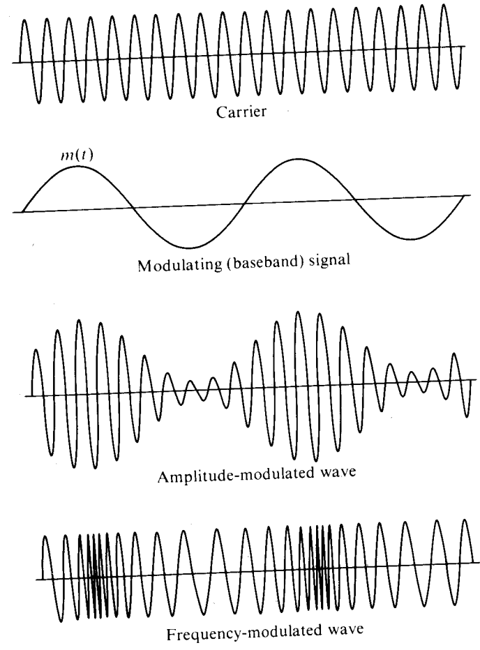
Figure 1.7 Modulation.
