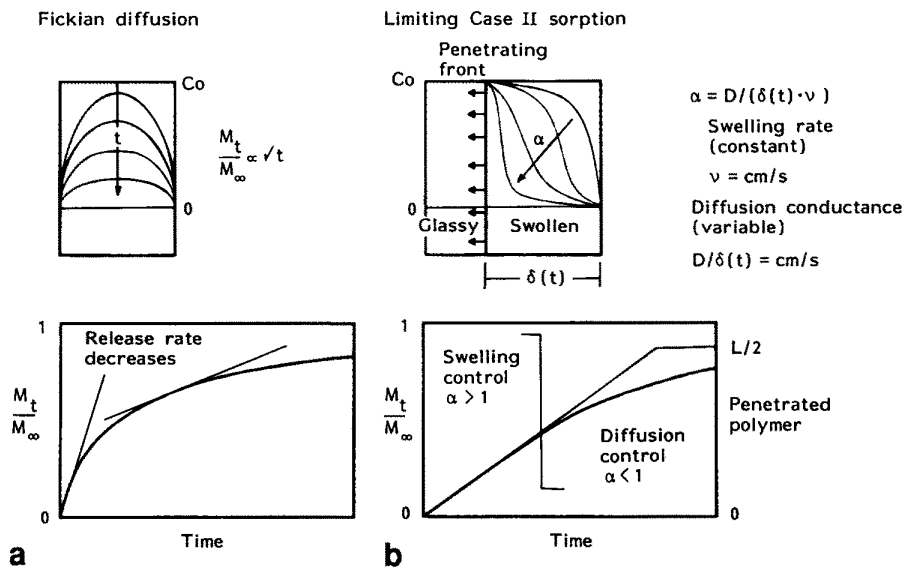
Figure 1 Release mechanisms from monolithic devices. a , Fickian diffusion; b , limiting Case II sorption.
