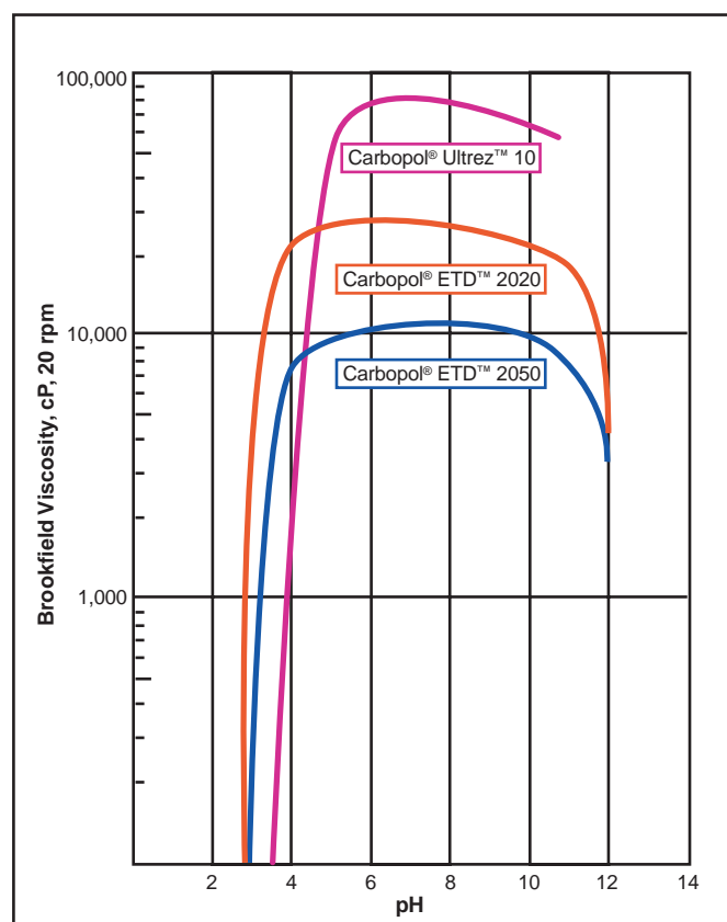
Figure 1 Carbopol Polymers Viscosity vs. pH (0.5% Concentration)
