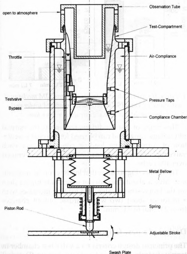
Figure 5: Schematic cross-section of newly developed test compartment for accelerated valve testing.
