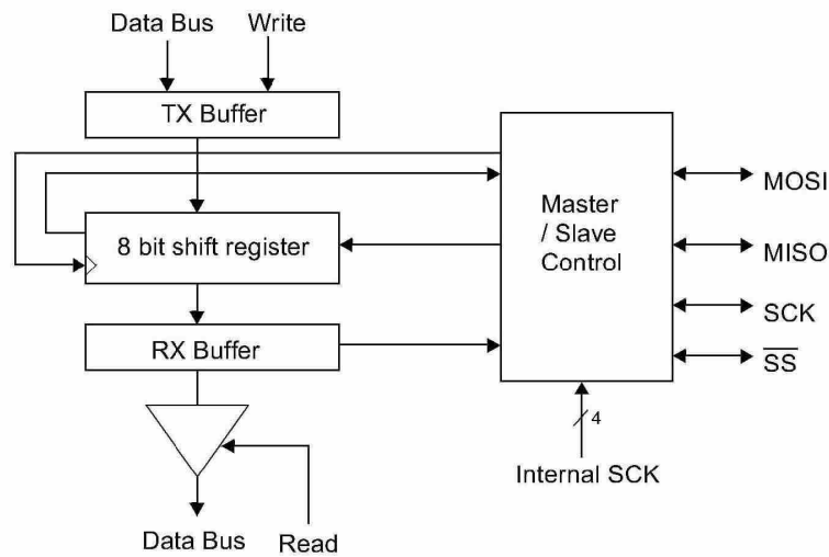
Figure 17-1. SPI Block Diagram
