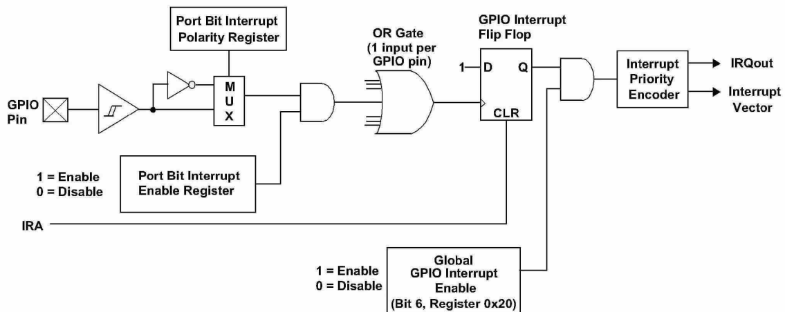
Figure 21-8. GPIO Interrupt Diagram
