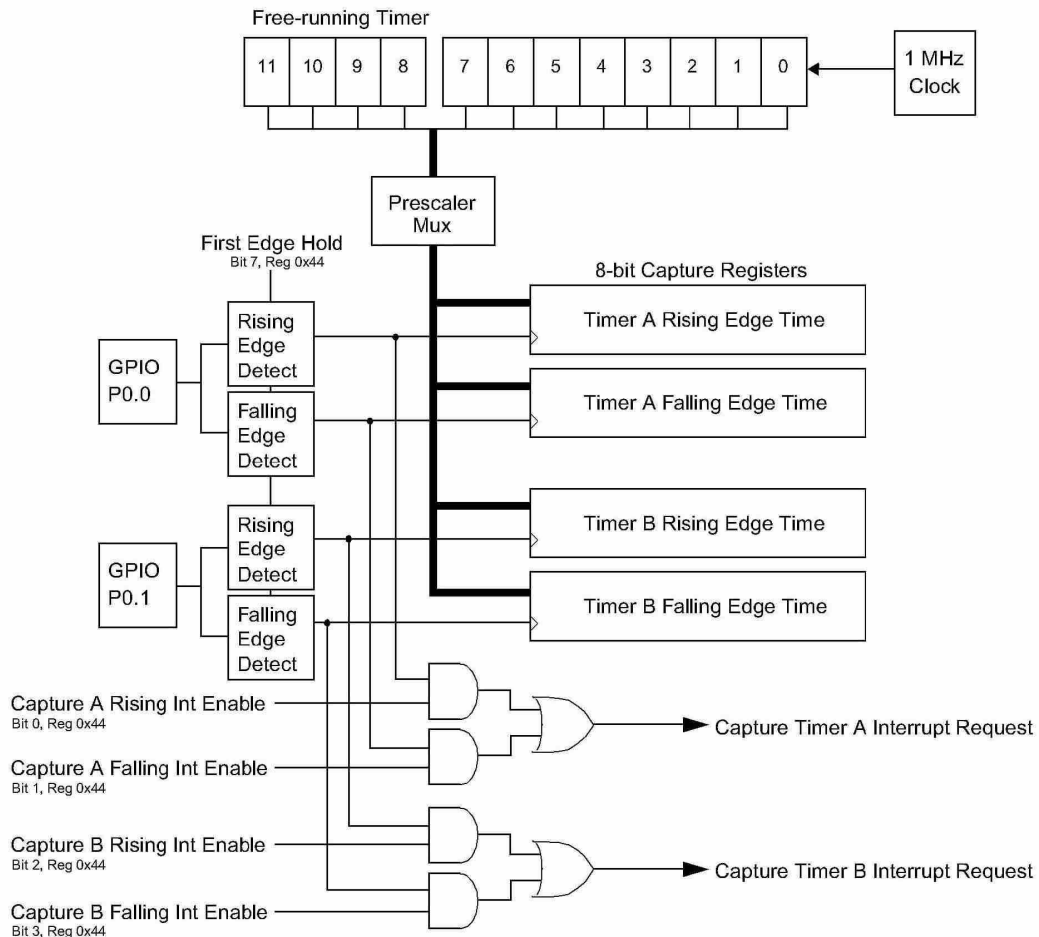
Figure 19-1. Capture Timers Block Diagram
