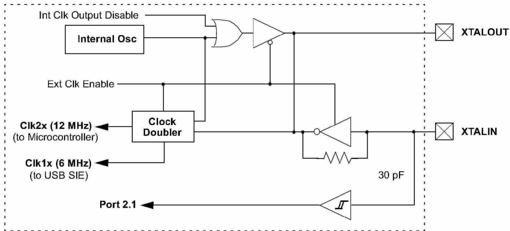
Figure 9-1. Clock Oscillator On-chip Circuit
