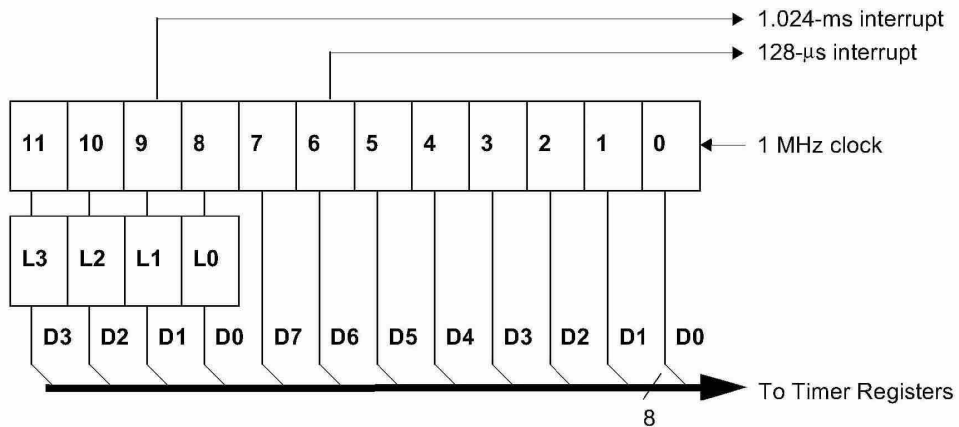
Figure 18-3. Timer Block Diagram
