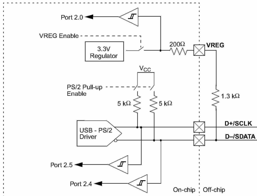
Figure 16-1. Diagram of USB - PS/2 System Connections
