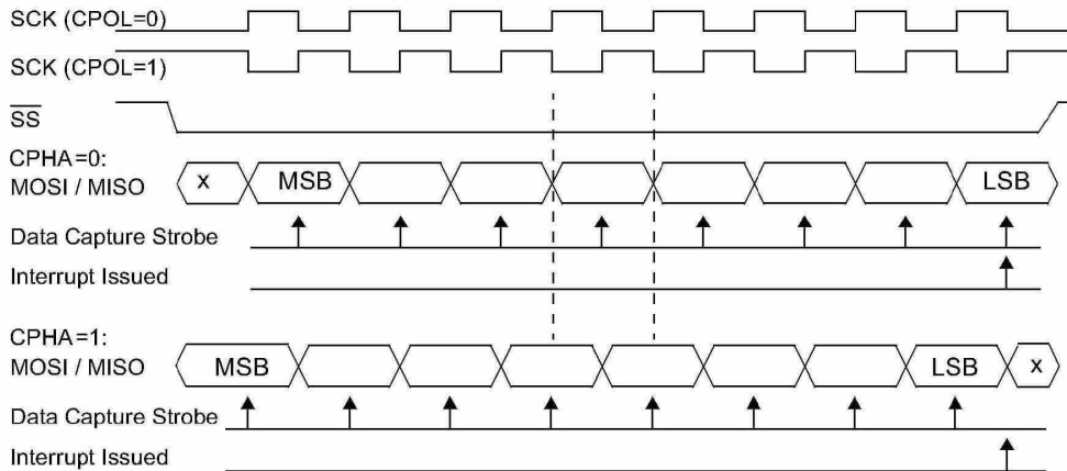
Figure 17-4. SPI Data Timing
