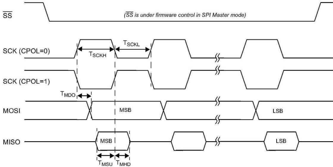
Figure 25-6. SPI Master Timing, CPHA=0
