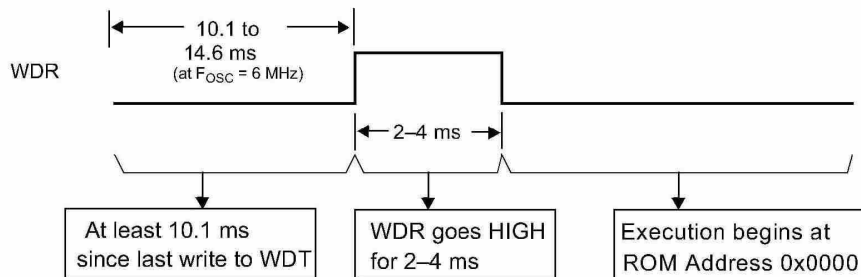
Figure 10-1. Watch Dog Reset (WDR)
