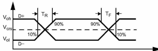
Figure 25-2. USB Data Signal Timing
