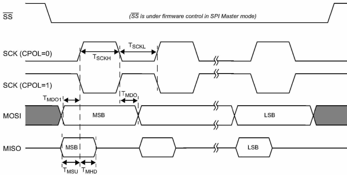
Figure 25-8. SPI Master Timing, CPHA=1
