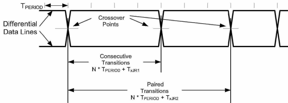
Figure 25-5. Differential Data Jitter
