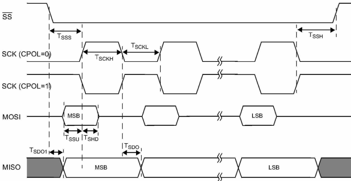
Figure 25-9. SPI Slave Timing, CPHA=1
