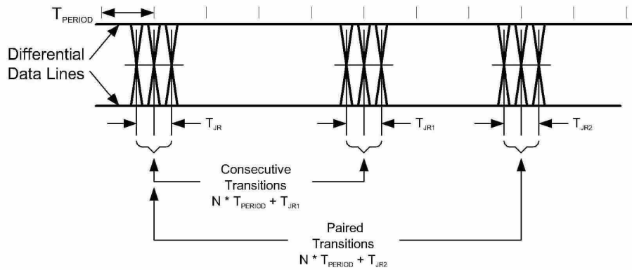
Figure 25-3. Receiver Jitter Tolerance
