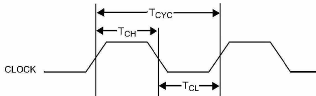
Figure 25-1. Clock Timing
