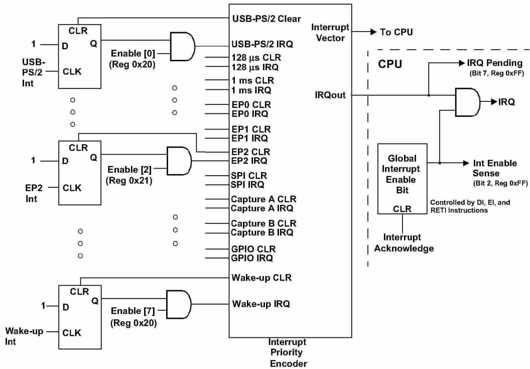
Figure 21-3. Interrupt Controller Logic Block Diagram
