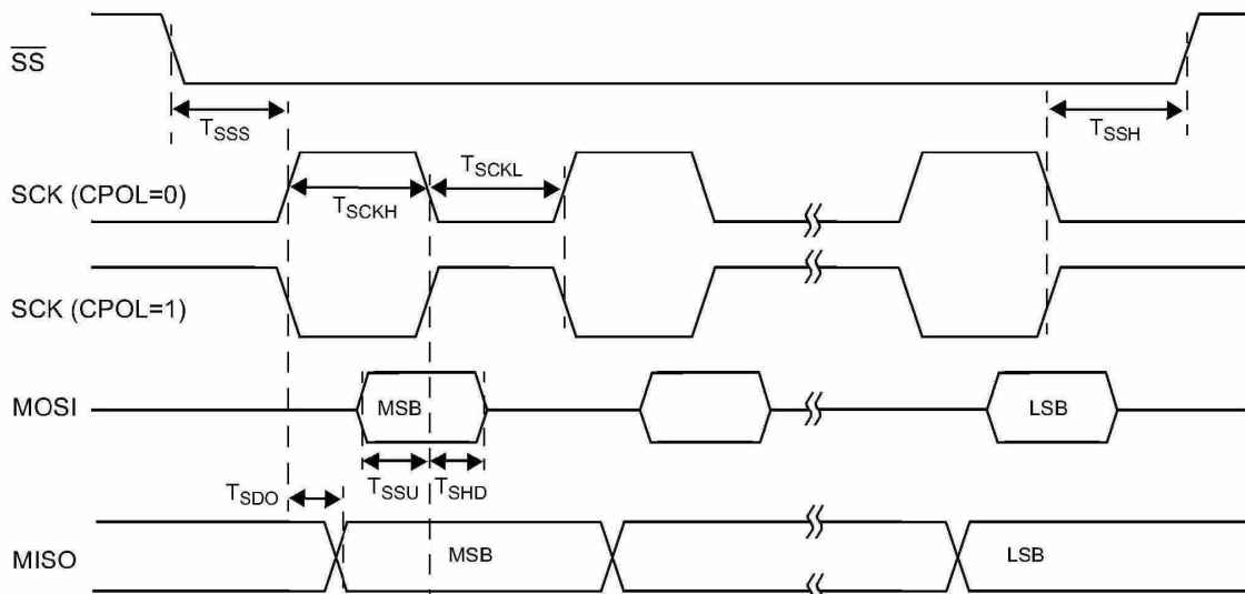
Figure 25-7. SPI Slave Timing, CPHA=0
