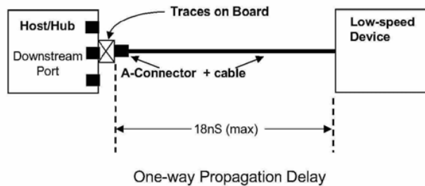
Figure 7-40. Low-speed Cable Delay
