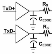
Figure 7-22. Placement of Optional Edge Rate Control Capacitors for Low-/full-speed
