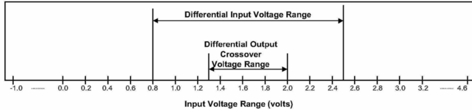
Figure 7-19. Differential Input Sensitivity Range for Low-/full-speed
