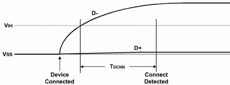
Figure 7-28. Low-speed Device Connect Detection
