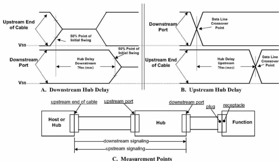
Figure 7-38. Hub Propagation Delay of Full-speed Differential Signals
