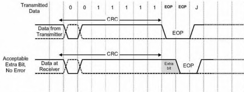
Figure 7-33. Illustration of Extra Bit Preceding EOP (Full-/low-speed)
