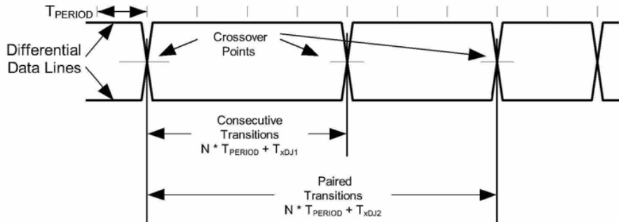
Figure 7-49. Differential Data Jitter for Low-/full-speed
