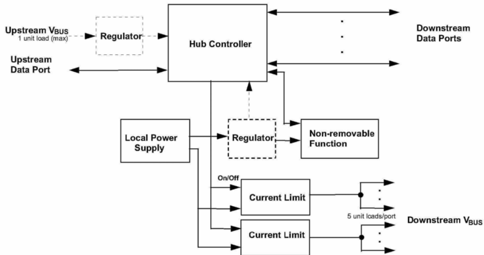
Figure 7-43. Compound Self-powered Hub
