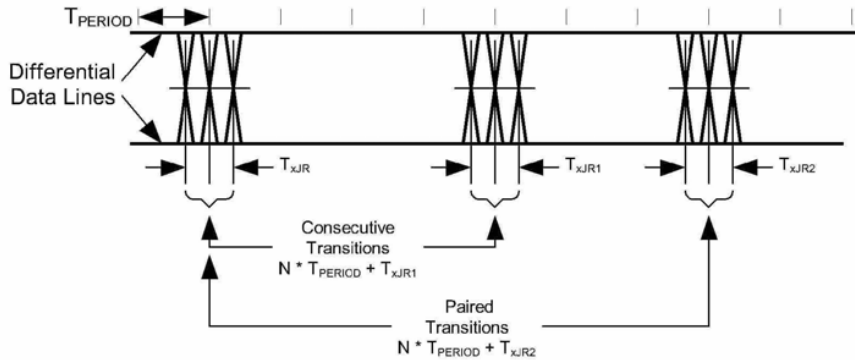
Figure 7-51. Receiver Jitter Tolerance for Low-/full-speed
