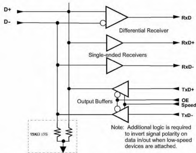
Figure 7-25. Downstream Facing Low-/full-speed Port Transceiver
