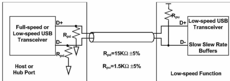
Figure 7-21. Low-speed Device Cable and Resistor Connections
