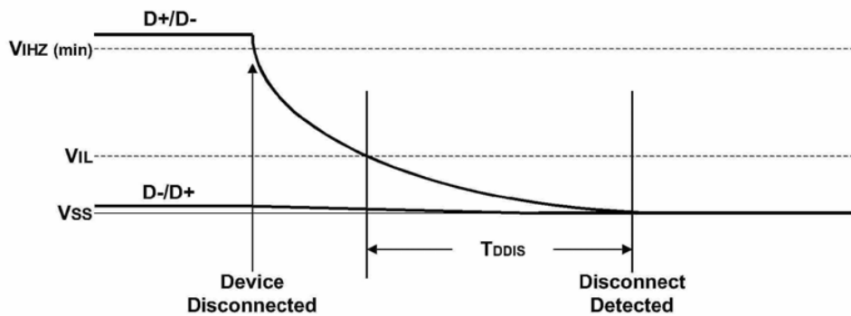
Figure 7-26. Low-/full-speed Disconnect Detection
