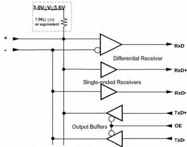
Figure 7-24. Upstream Facing Full-speed Port Transceiver
