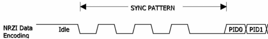
Figure 7-35. Sync Pattern (Low-/full-speed)
