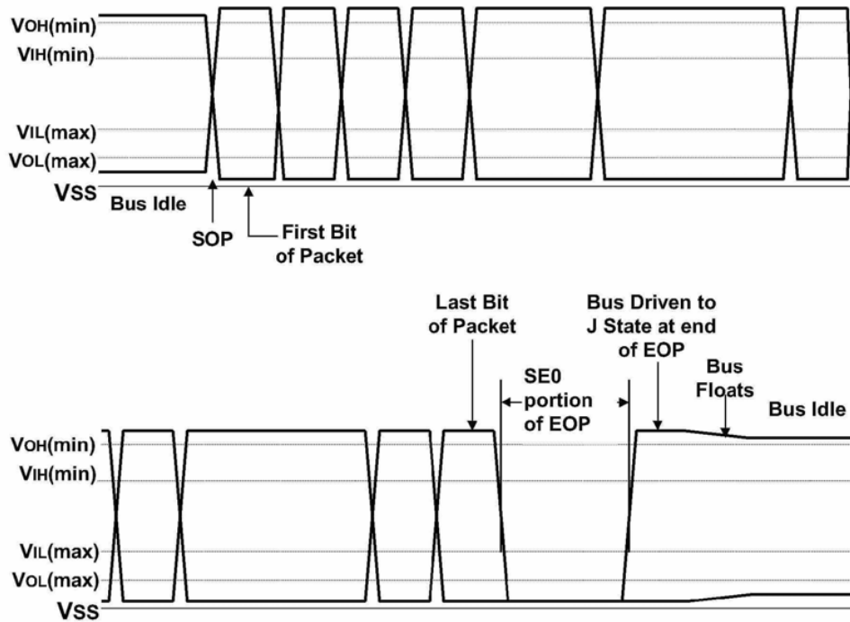
Figure 7-30. Low-/full-speed Packet Voltage Levels
