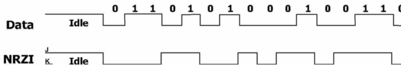
Figure 7-31. NRZI Data Encoding
