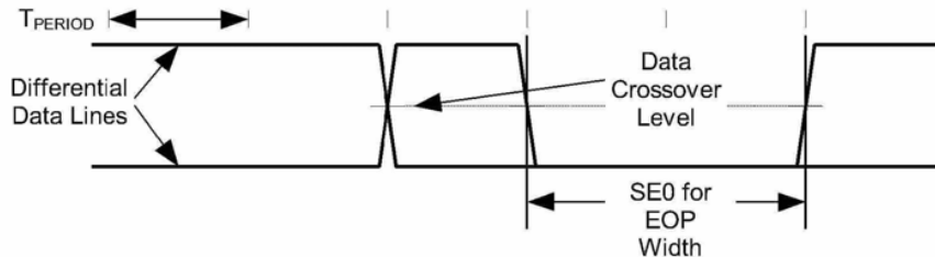
Figure 7-37. SE0 for EOP Width Timing
