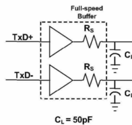
Figure 7-9. Full-speed Load
