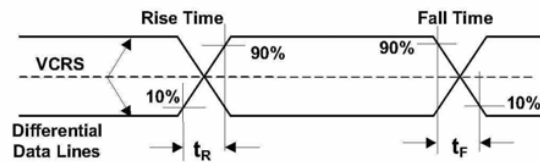
Figure 7-8. Data Signal Rise and Fall Time
