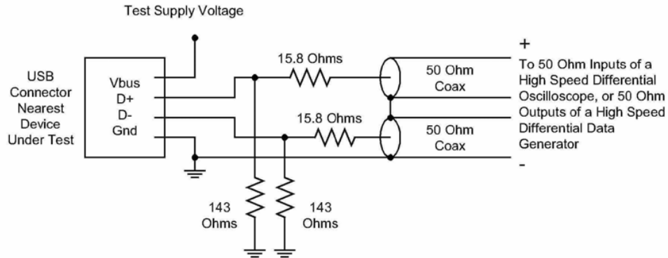
Figure 7-12. Transmitter/Receiver Test Fixture
