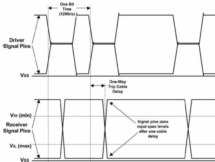
Figure 7-6. Full-speed Signal Waveforms
