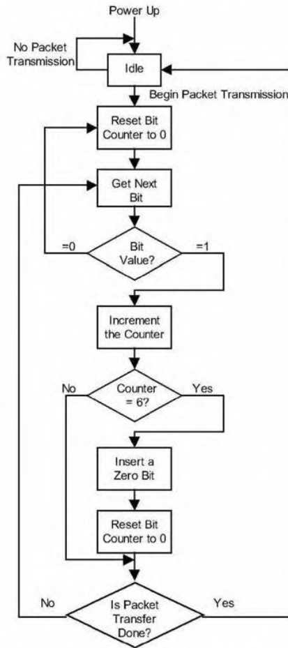
Figure 7-34. Flow Diagram for Bit Stuffing
