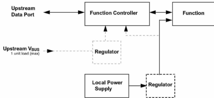
Figure 7-46. Self-powered Function
