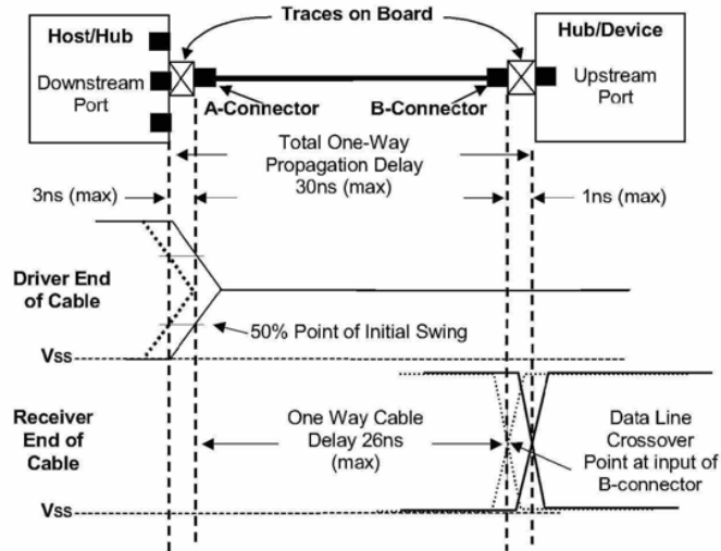
Figure 7-39. Full-speed Cable Delay
