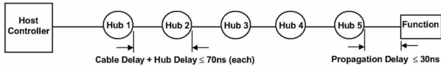
Figure 7-41. Worst-case End-to-end Signal Delay Model for Low-/full-speed
