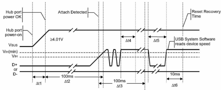
Figure 7-29. Power-on and Connection Events Timing
