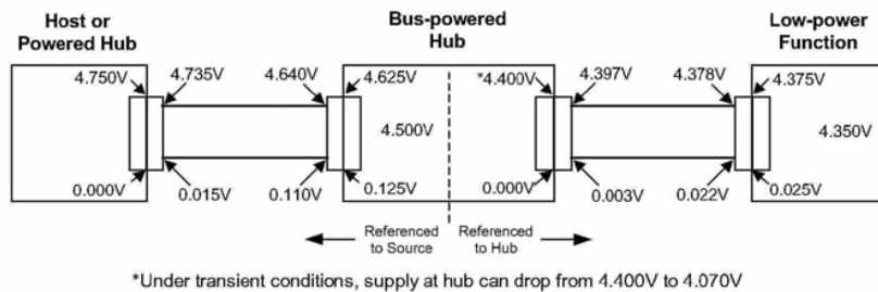
Figure 7-47. Worst-case Voltage Drop Topology (Steady State)
