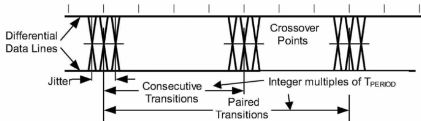
Figure 7-36. Data Jitter Taxonomy
