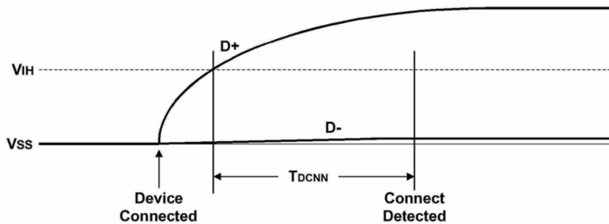
Figure 7-27. Full-/high-speed Device Connect Detection
