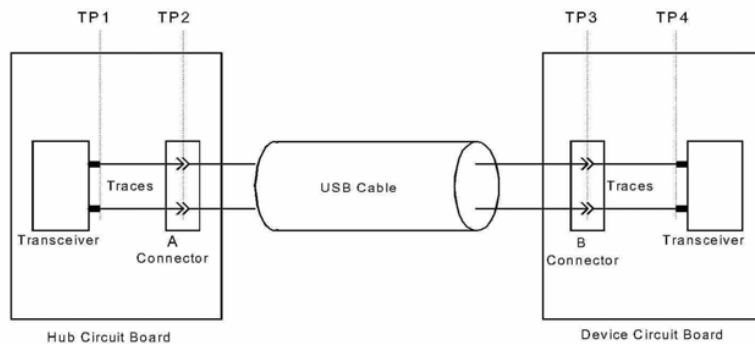
Figure 7-11. Measurement Planes
