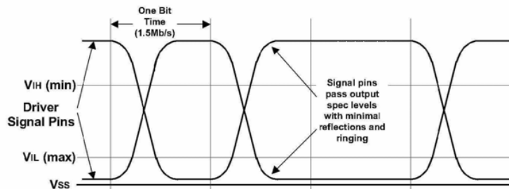
Figure 7-7. Low-speed Driver Signal Waveforms
