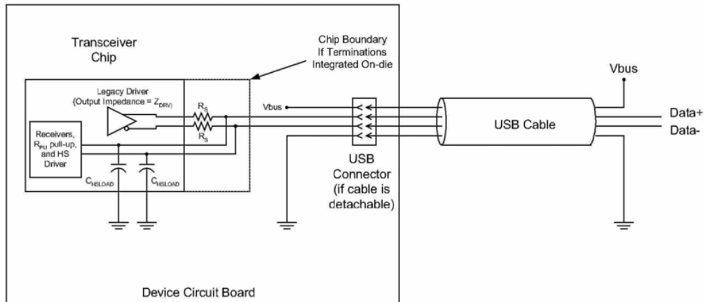
Figure 7-23. Diagram for High-speed Loading Equivalent Circuit
