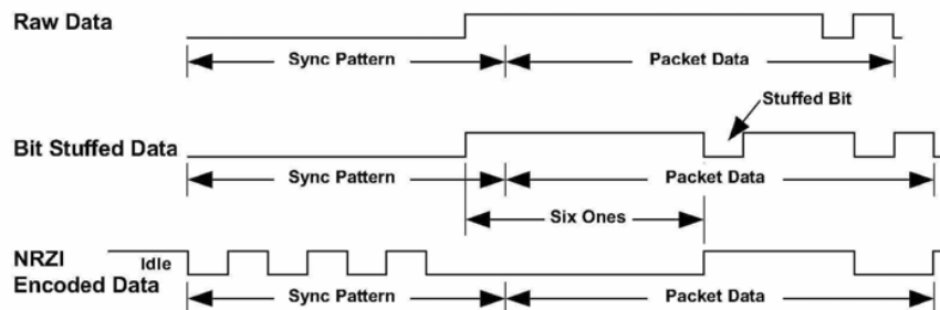
Figure 7-32. Bit Stuffing
