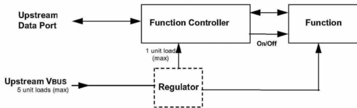
Figure 7-45. High-power Bus-powered Function
