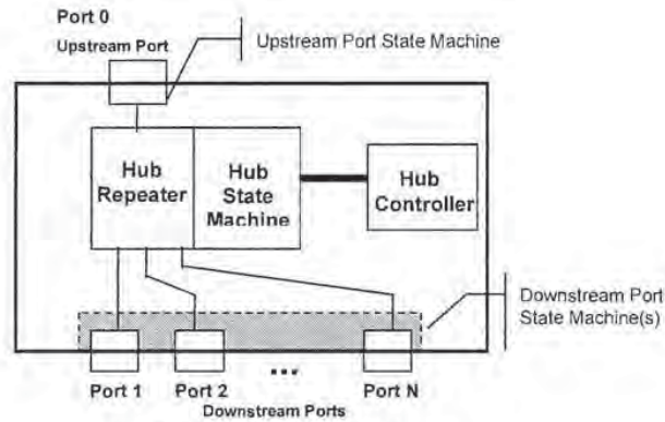
Figure 11-1. Hub Architecture
