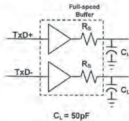
Figure 7-7. Full-speed Load
