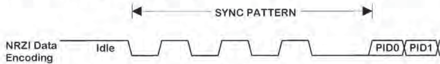
Figure 7-25. Sync Pattern
