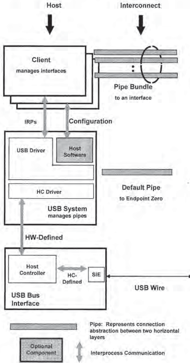
Figure 10-2. Host Communications
