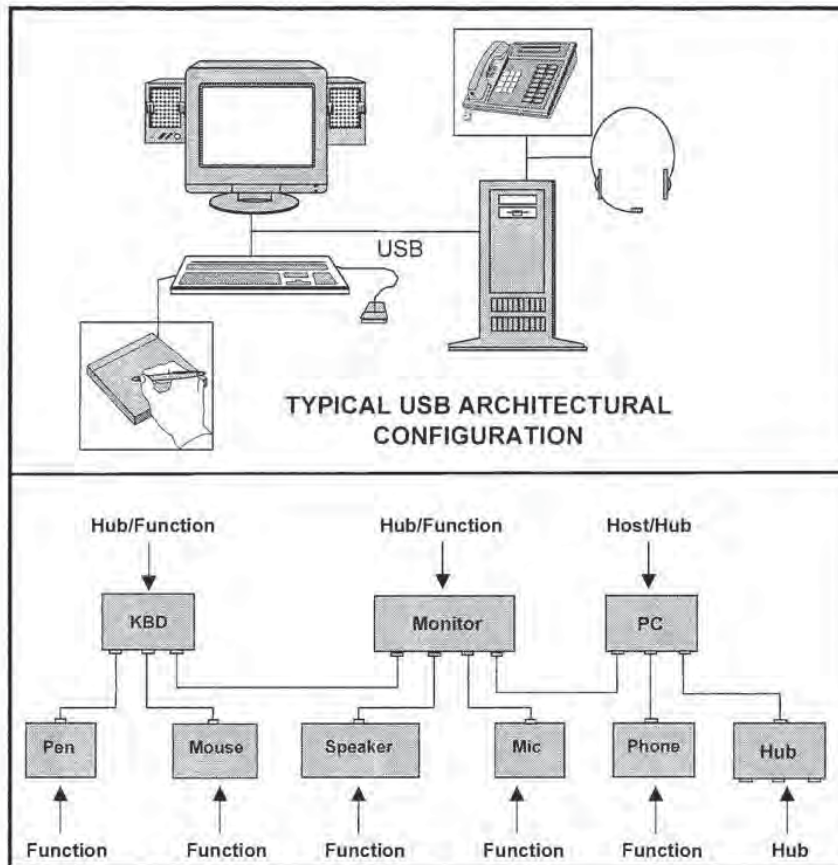
Figure 4-4. Hubs in a Desktop Computer Environment
