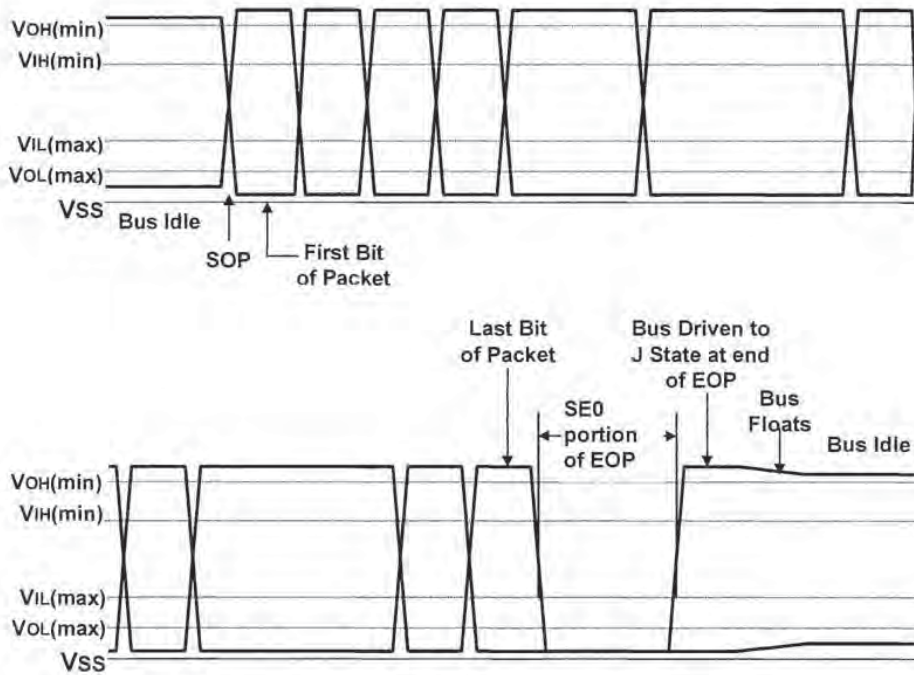
Figure 7-20. Packet Voltage Levels
