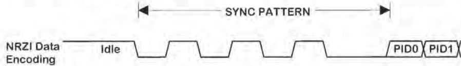
Figure 7-25. Sync Pattern
