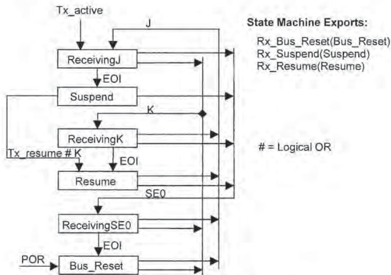
Figure 11-7. Upstream Port Receiver State Machine
