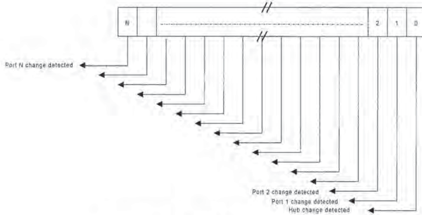
Figure 11-14. Hub and Port Status Change Bitmap
