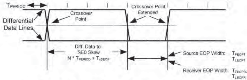
Figure 7-40. Differential-to-EOP Transition Skew and EOP Width
