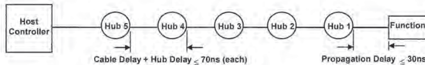
Figure 7-31. Worst-case End to End Signal Delay Model
