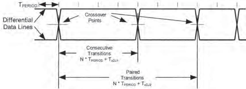
Figure 7-39. Differential Data Jitter
