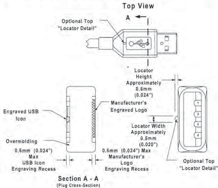
Figure 6-6. Typical USB Plug Orientation
