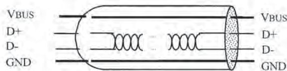
Figure 4-2. USB Cable
