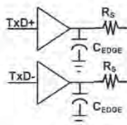
Figure 7-12. Placement of Optional Edge Rate Control Capacitors
