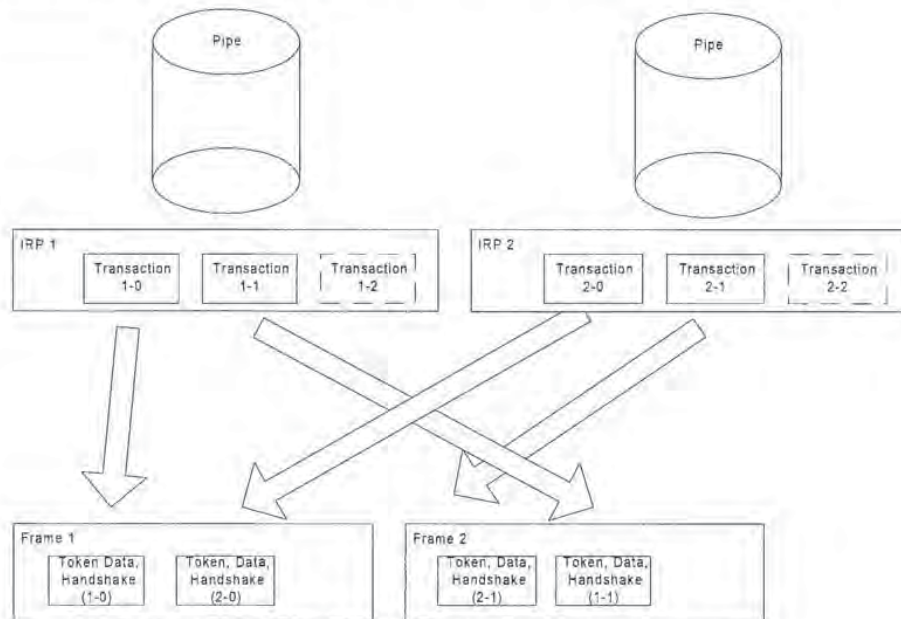
Figure 5-12. Arrangement of IRPs to Transactions/Frames
