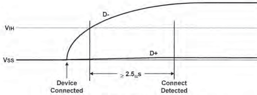
Figure 7-17. Low-speed Device Connect Detection
