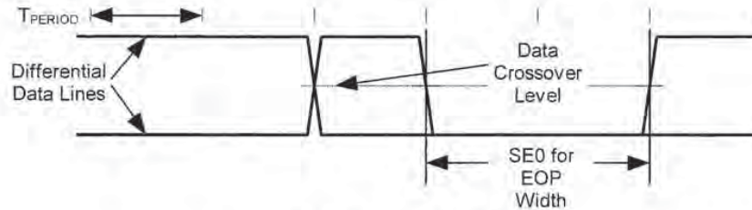
Figure 7-27. SE0 for EOP Width Timing
