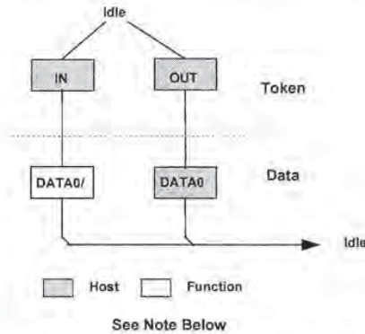
Figure 8-14. Isochronous Transaction Format
