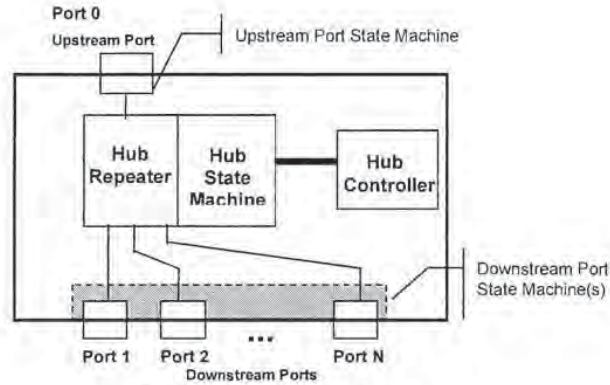
Figure 11-1. Hub Architecture
