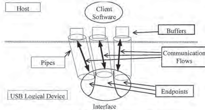
Figure 5-9. USB Communication Flow
