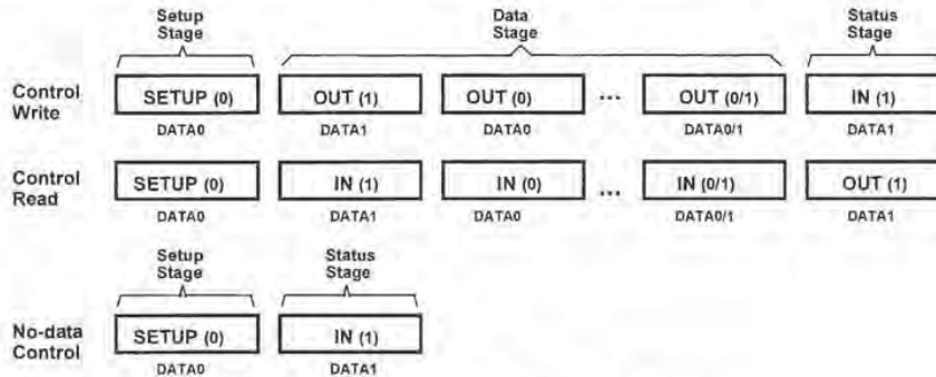
Figure 8-12. Control Read and Write Sequences
