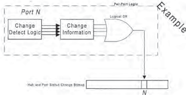
Figure 11-15. Example Hub and Port Change Bit Sampling
