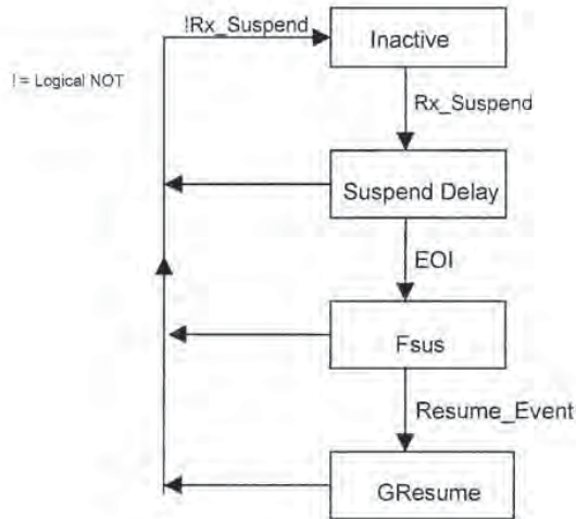
Figure 11-5. Internal Port State Machine
