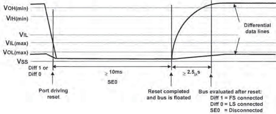
Figure 7-18. Bus State Evaluation after reset (optional)
