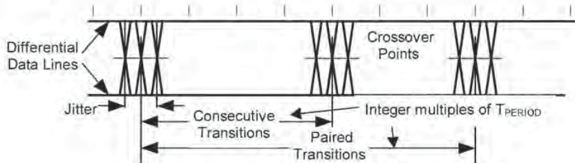
Figure 7-26. Data Jitter Taxonomy
