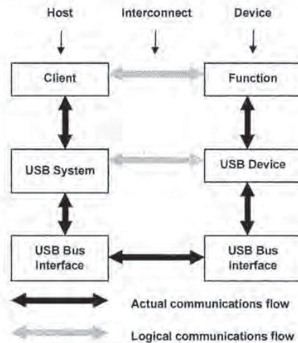
Figure 10-1. Interlayer Communications Model
