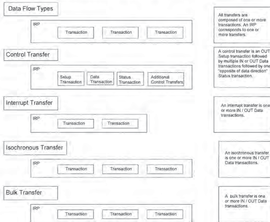
Figure 5-11. Transfers for Communication Flows
