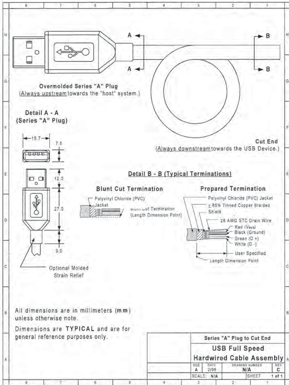
Figure 6-3. USB Full-speed Hardwired Cable Assembly
