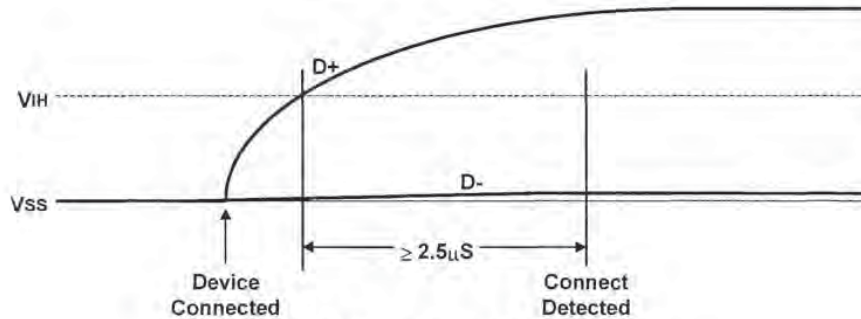
Figure 7-16. Full-speed Device Connect Detection
