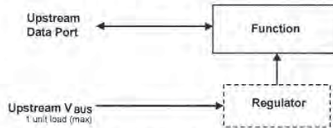
Figure 7-34. Low-power Bus-powered Function
