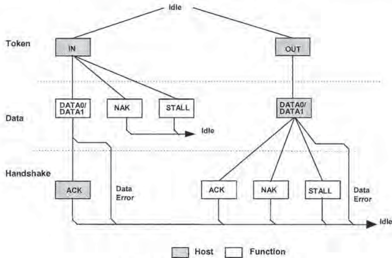
Figure 8-9. Bulk Transaction Format
