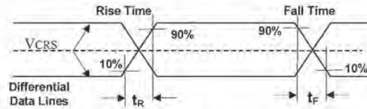
Figure 7-6. Data Signal Rise and Fall Time
