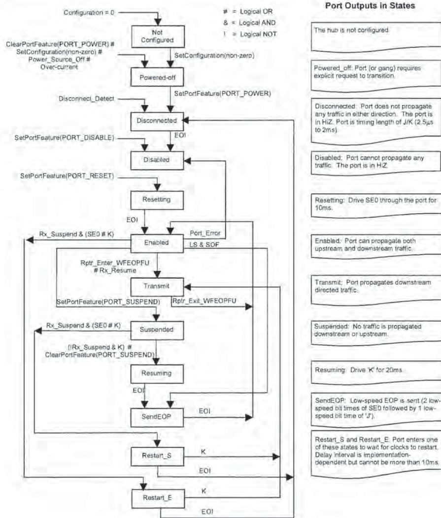
Figure 11-6. Downstream Hub Port State Machine
