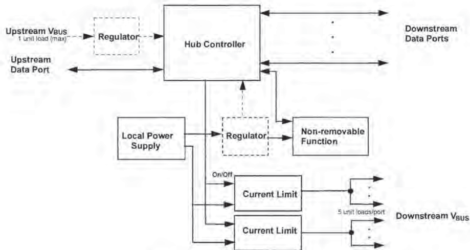
Figure 7-33. Compound Self-powered Hub
