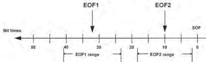
Figure 11-4. EOF Timing Points
