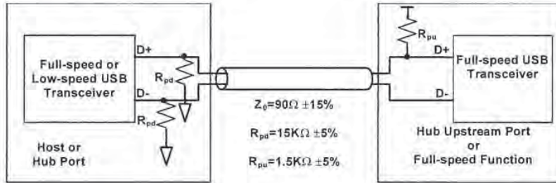
Figure 7-10. Full-speed Device Cable and Resistor Connections
