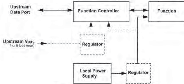
Figure 7-36. Self-powered Function
