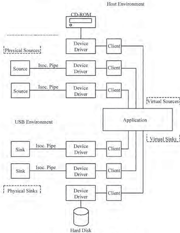
Figure 5-15. Example Source/Sink Connectivity
