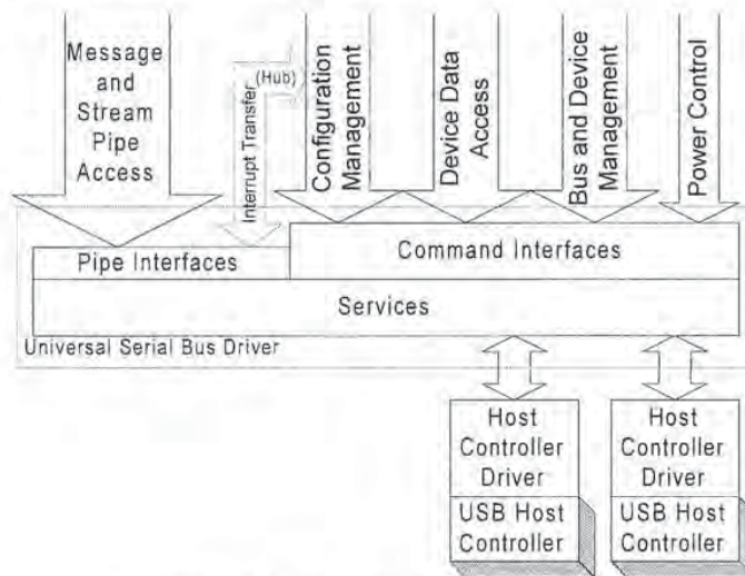
Figure 10-5. Universal Serial Bus Driver Structure
