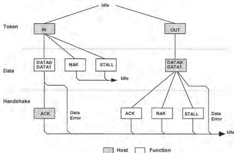
Figure 8-13. Interrupt Transaction Format
