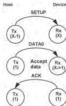
Figure 8-15. SETUP Initialization
