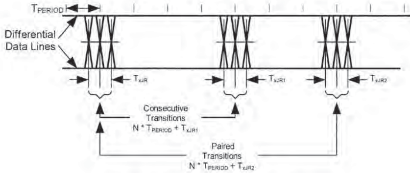
Figure 7-41. Receiver Jitter Tolerance
