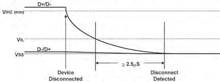
Figure 7-15. Disconnect Detection
