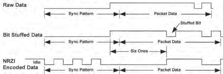
Figure 7-22. Bit Stuffing
