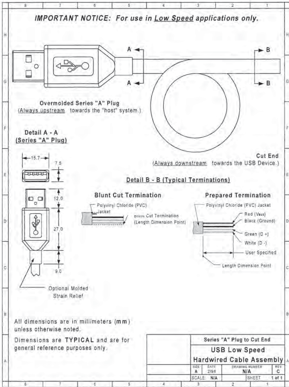
Figure 6-4. USB Low-speed Hardwired Cable Assembly
