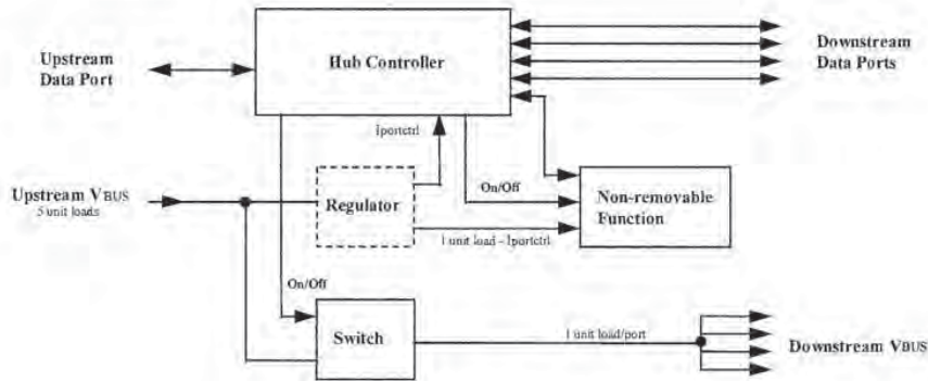
Figure 7-32. Compound Bus-powered Hub
