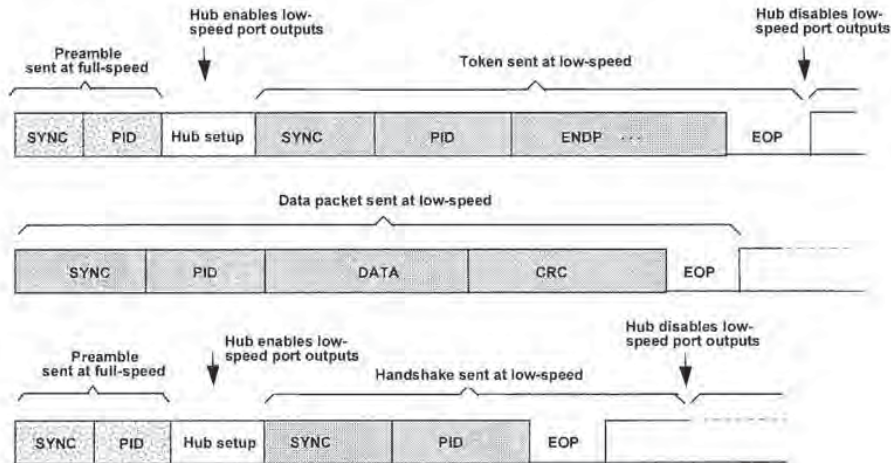
Figure 8-19. Low-speed Transaction
