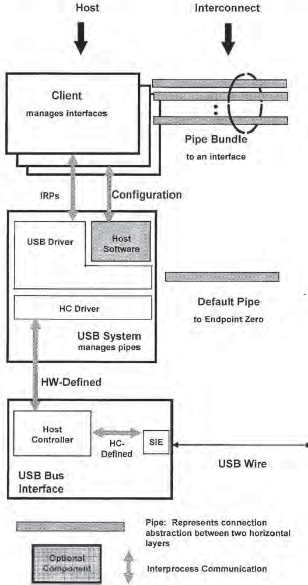
Figure 10-2. Host Communications
