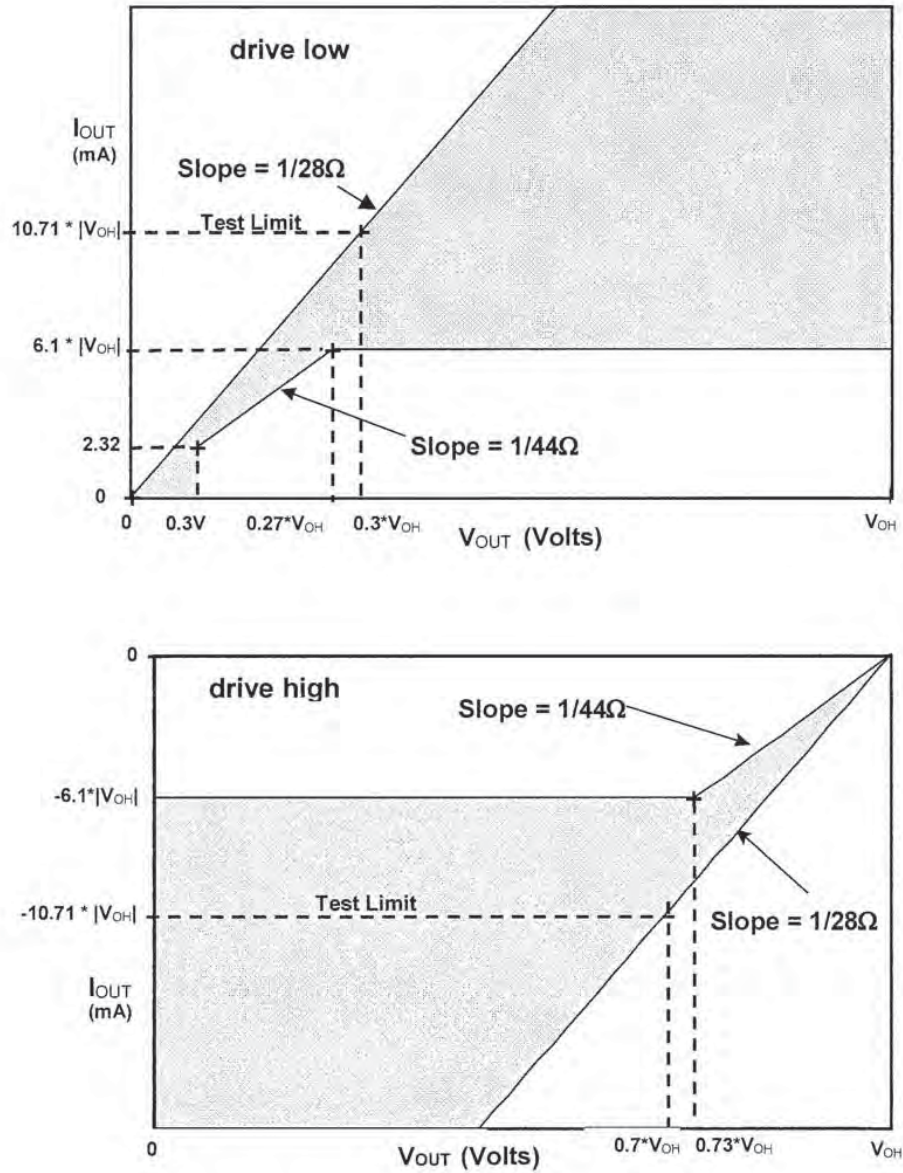
Figure 7-3. Full-speed Buffer V/I Characteristics
