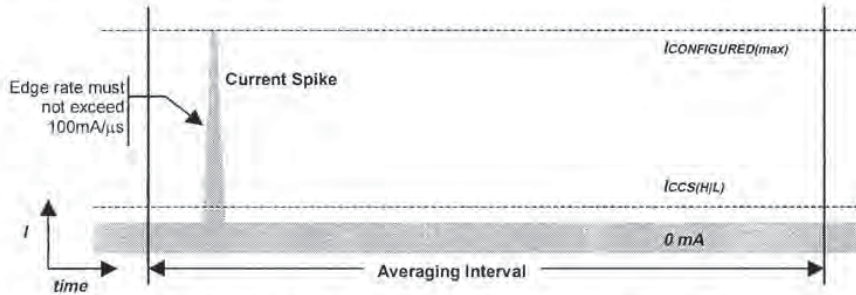
Figure 7-38. Typical Suspend Current Averaging Profile
