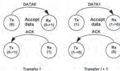
Figure 8-16. Consecutive Transactions
