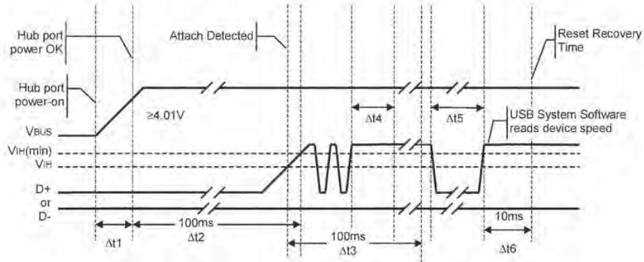
Figure 7-19. Power-on and Connection Events Timing
