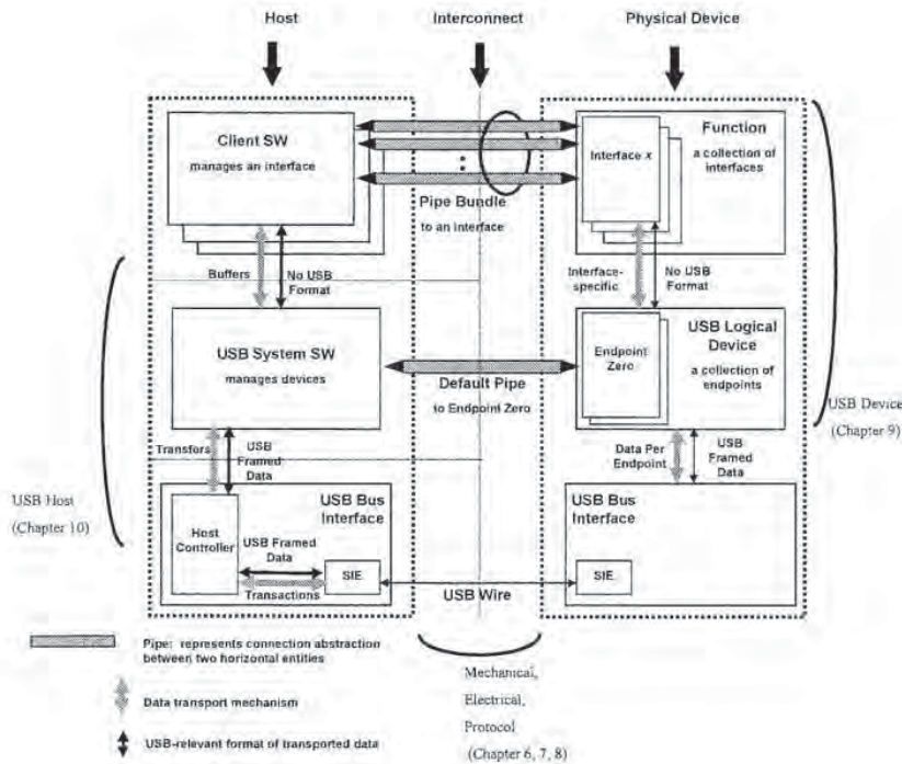
Figure 5-8. USB Host/Device Detailed View
