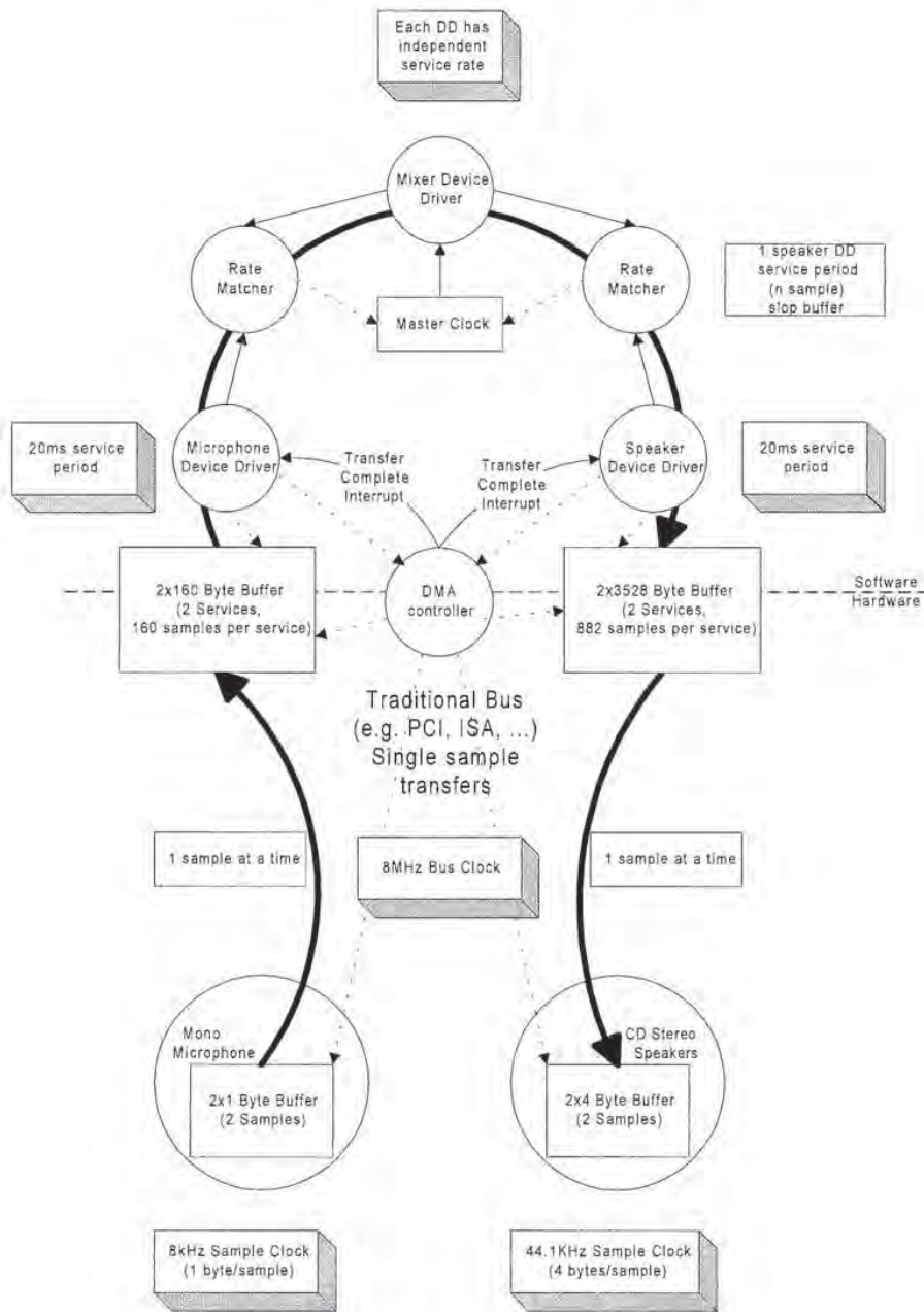
Figure 5-13. Non-USB Isochronous Example
