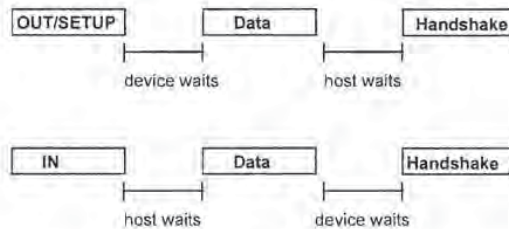
Figure 8-20. Bus Turn-around Timer Usage
