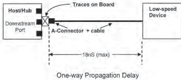
Figure 7-30. Low-speed Cable Delay
