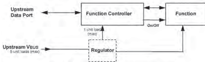
Figure 7-35. High-power Bus-powered Function
