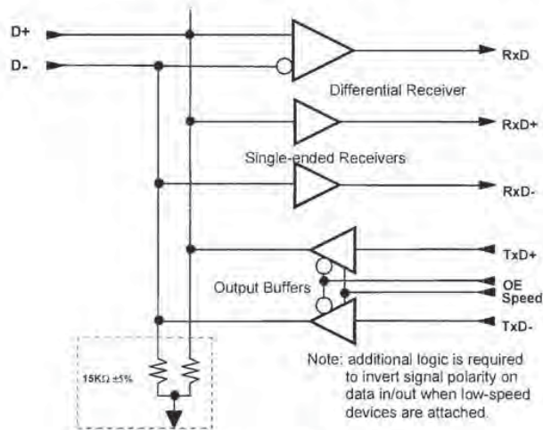
Figure 7-14. Downstream Port Transceiver
