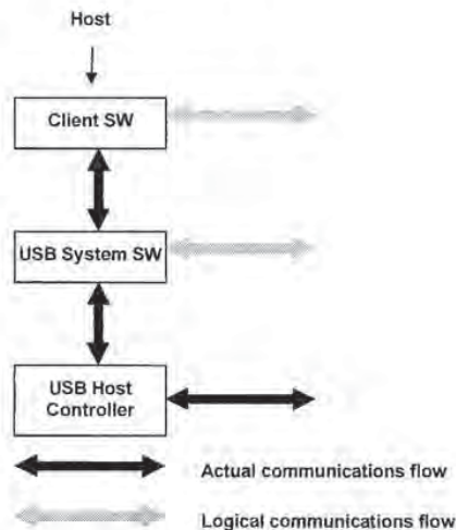
Figure 5-3. Host Composition
