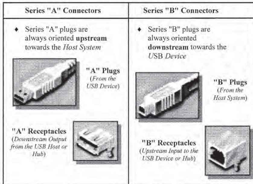
Figure 6-1. Keyed Connector Protocol
