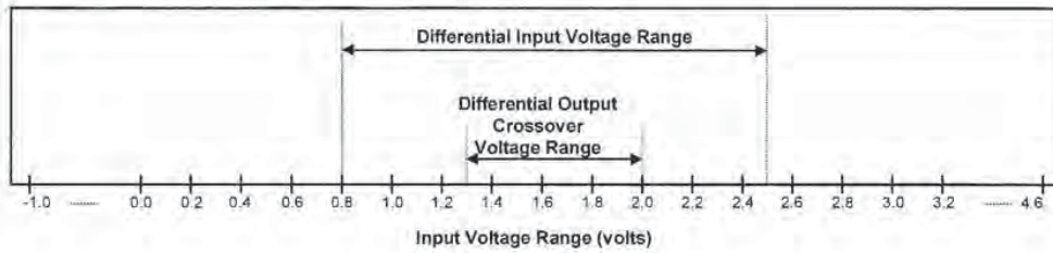
Figure 7-9. Differential Input Sensitivity Range
