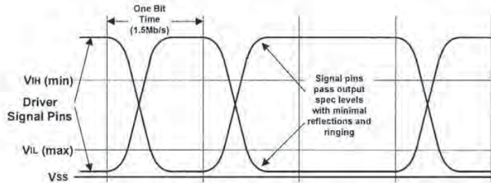
Figure 7-5. Low-speed Driver Signal Waveforms
