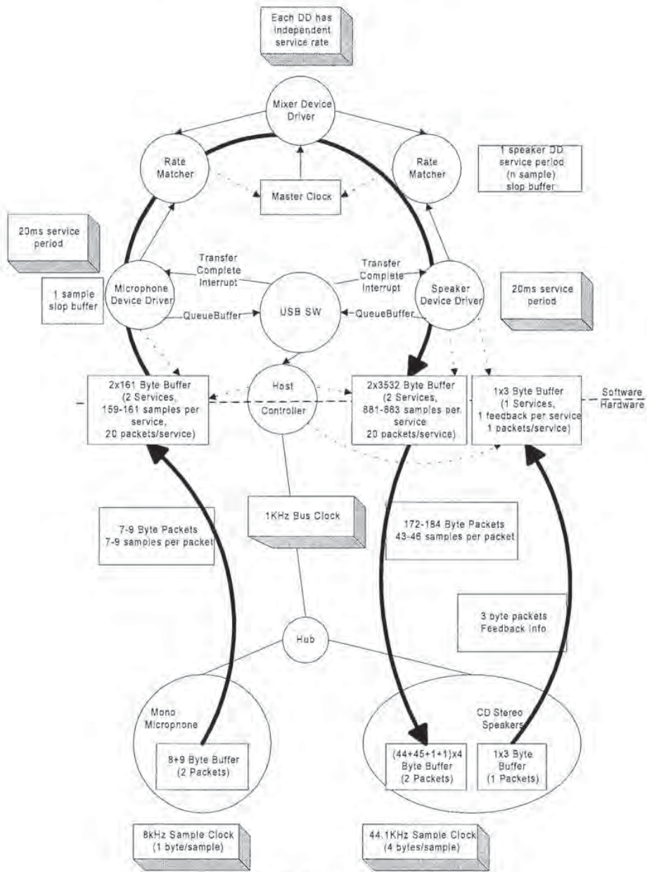
Figure 5-14. USB Isochronous Application
