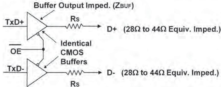
Figure 7-2. Example Full-speed CMOS Driver Circuit
