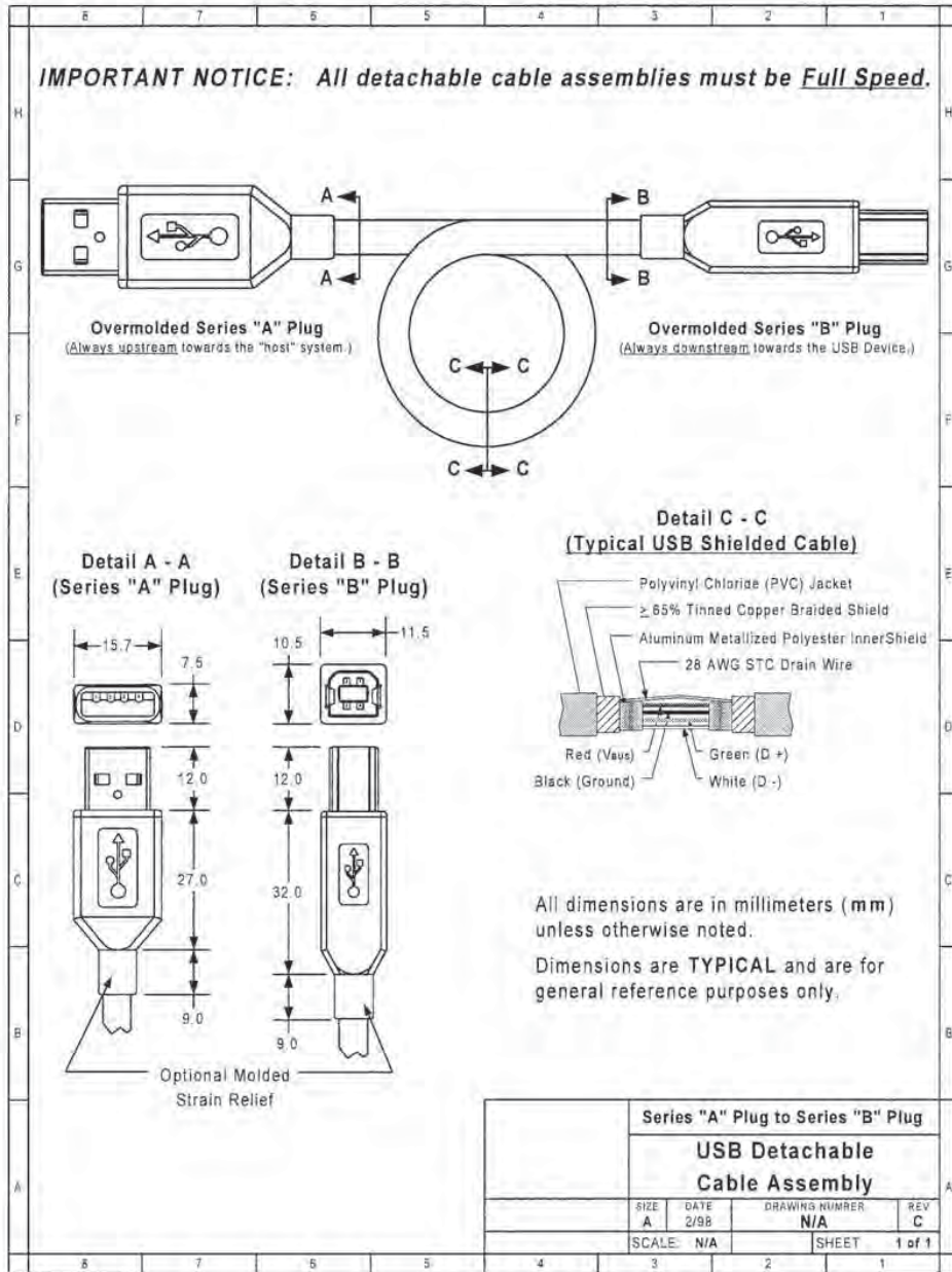
Figure 6-2. USB Detachable Cable Assembly
