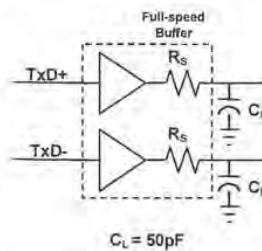
Figure 7-7. Full-speed Load
