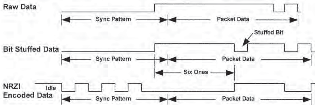
Figure 7-22. Bit Stuffing
