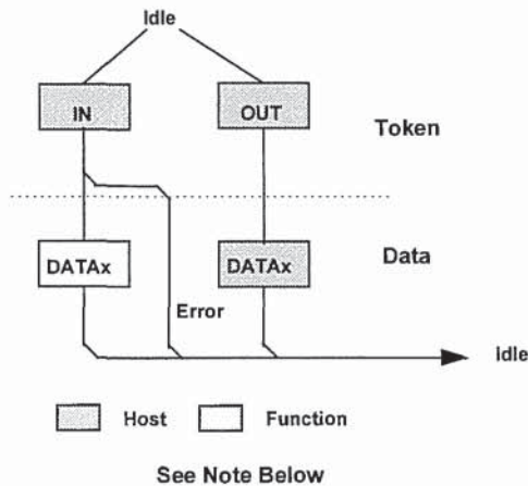
Figure 8-39. Isochronous Transaction Format
