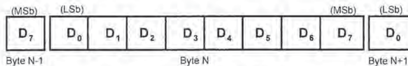
Figure 8-4. Data Field Format
