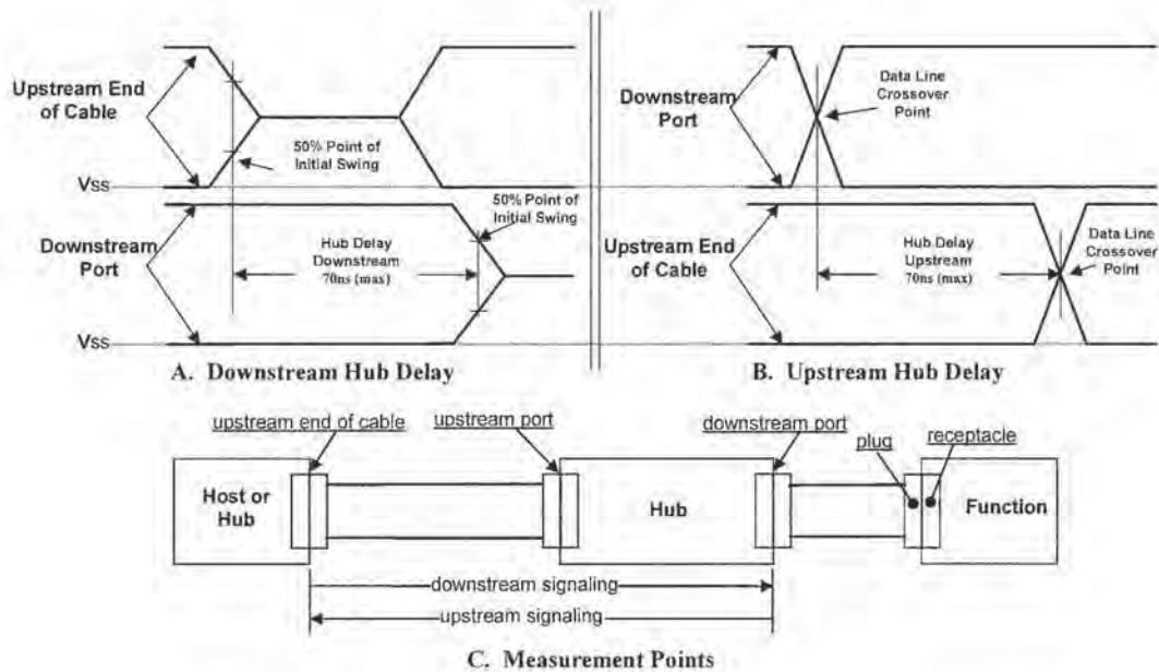
Figure 7-28. Hub Propagation Delay of Full-speed Differential Signals
