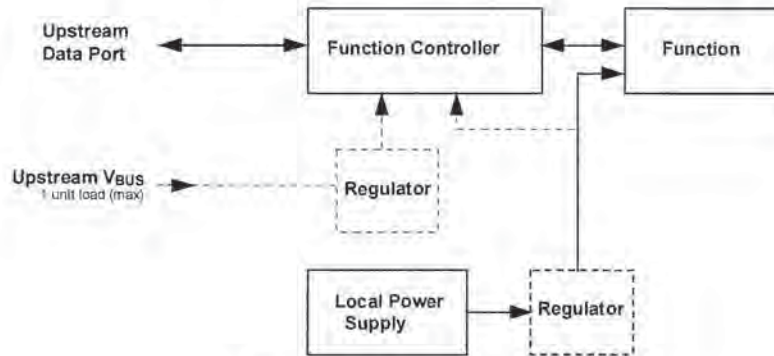
Figure 7-36. Self-powered Function
