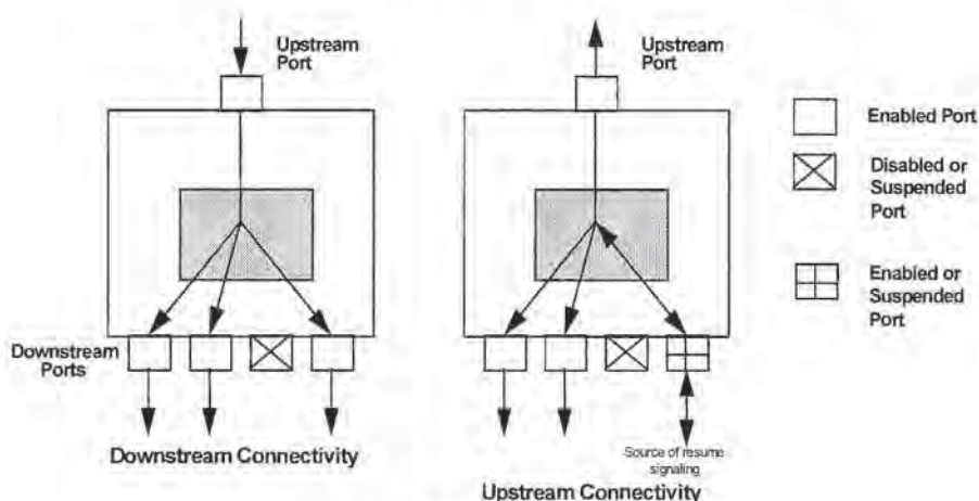
Figure 11-3. Resume Connectivity
