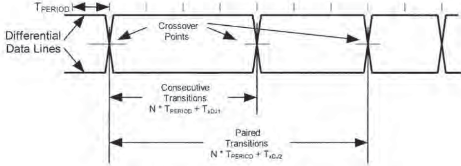
Figure 7-39. Differential Data Jitter
