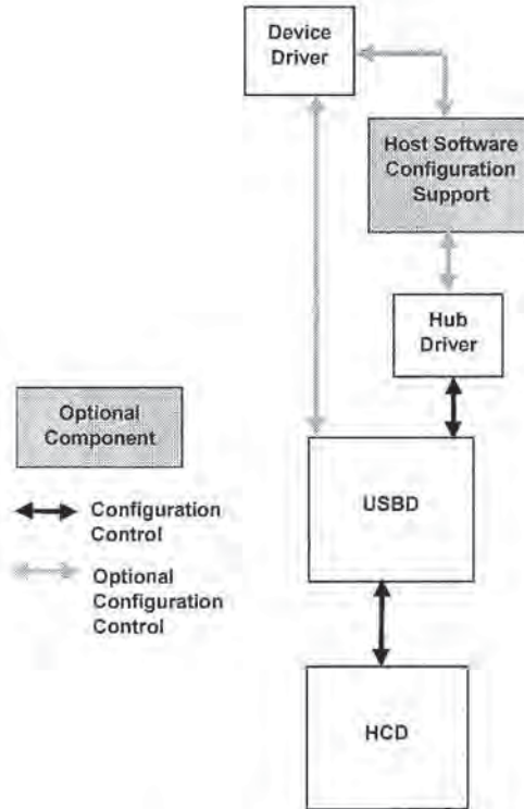
Figure 10-4. Configuration Interactions
