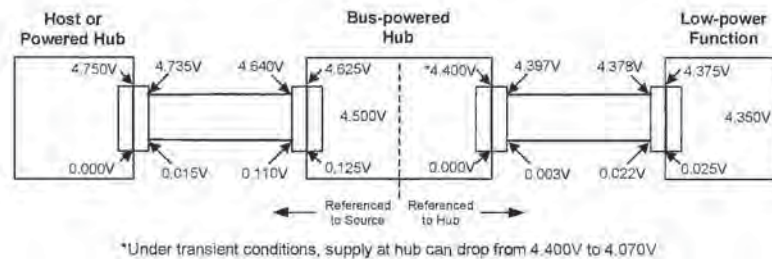
Figure 7-37. Worst-case Voltage Drop Topology (Steady State)
