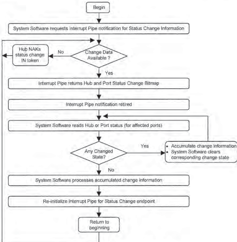
Figure 11-13. Port Status Handling Method
