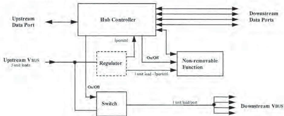
Figure 7-32. Compound Bus-powered Hub
