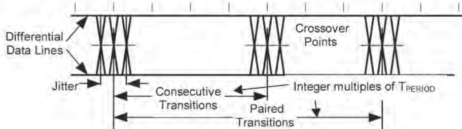
Figure 7-26. Data Jitter Taxonomy
