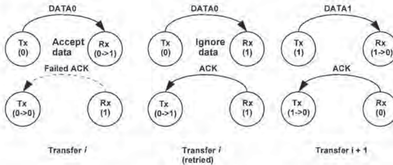
Figure 8-18. Corrupted ACK Handshake with Retry
