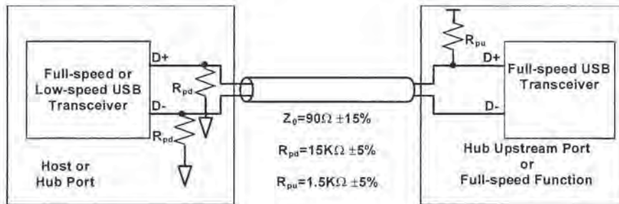
Figure 7-10. Full-speed Device Cable and Resistor Connections
