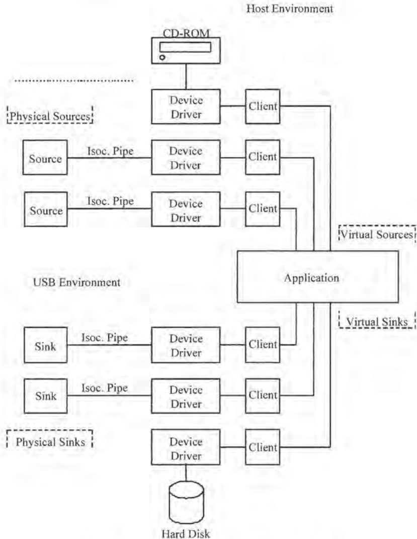
Figure 5-15. Example Source/Sink Connectivity
