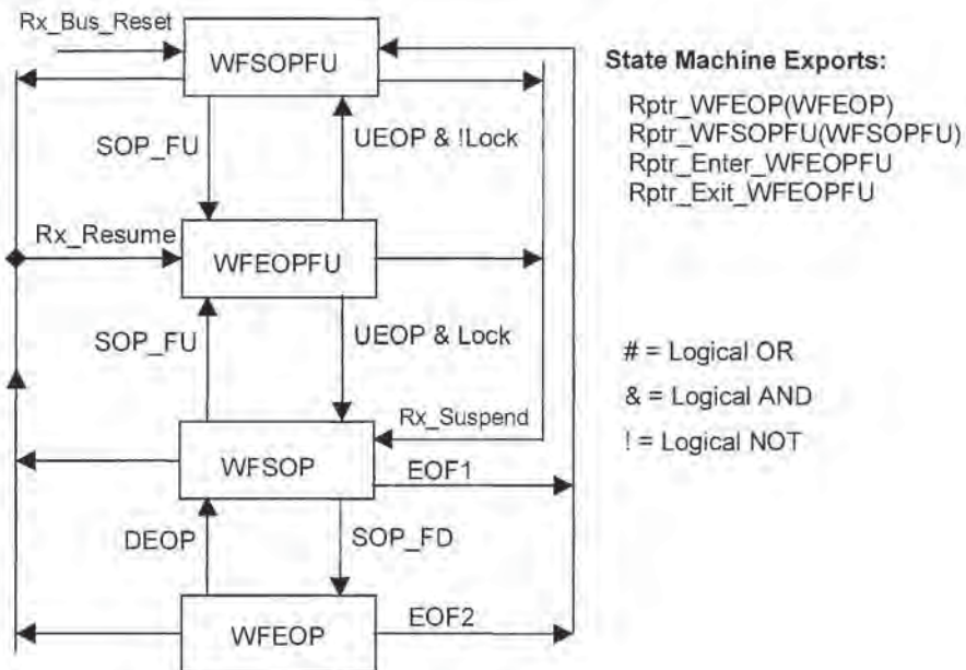
Figure 11-9. Hub Repeater State Machine
