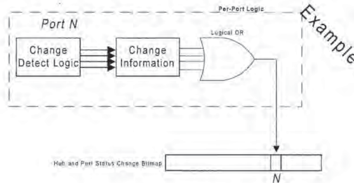
Figure 11-15. Example Hub and Port Change Bit Sampling
