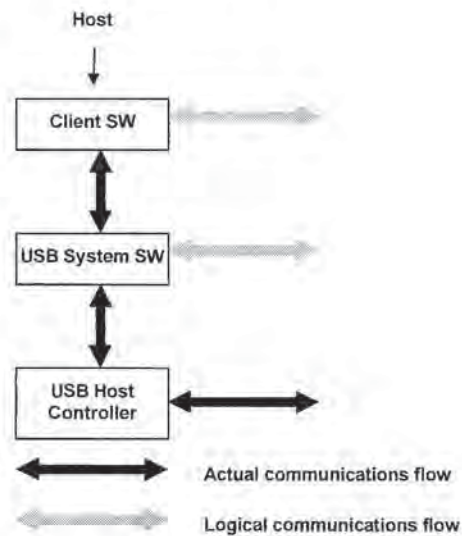
Figure 5-3. Host Composition
