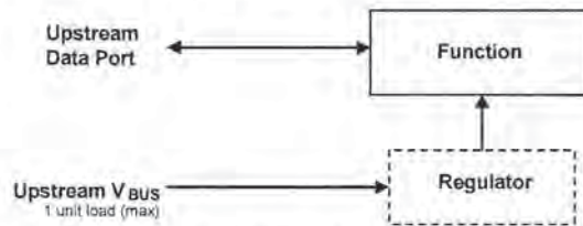
Figure 7-34. Low-power Bus-powered Function
