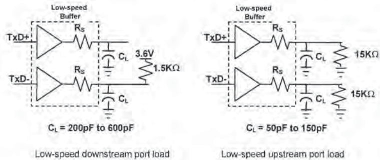
Figure 7-8. Low-speed Port Loads
