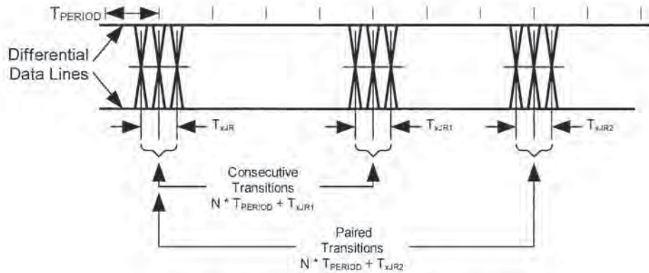
Figure 7-41. Receiver Jitter Tolerance
