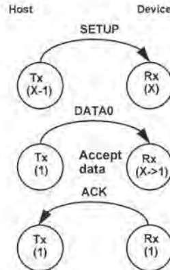
Figure 8-15. SETUP Initialization
