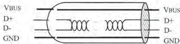
Figure 4-2. USB Cable
