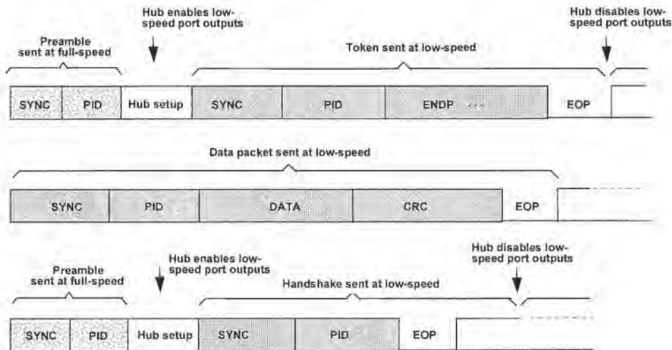
Figure 8-19. Low-speed Transaction
