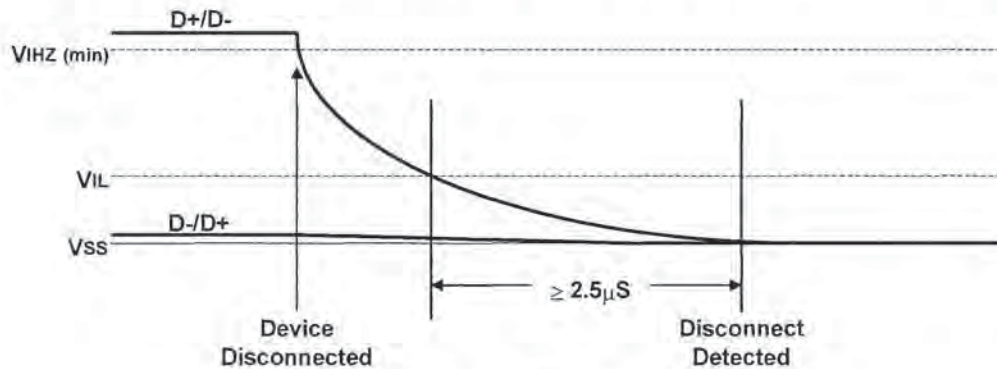
Figure 7-15. Disconnect Detection
