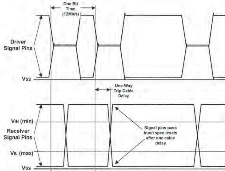
Figure 7-4. Full-speed Signal Waveforms
