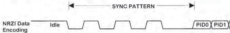
Figure 7-25. Sync Pattern
