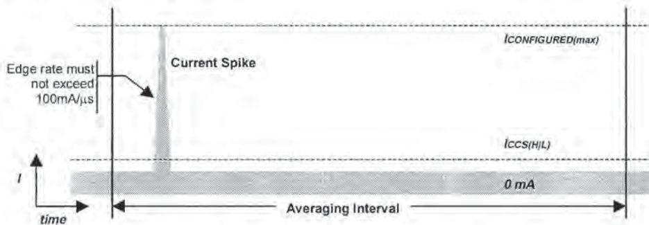
Figure 7-38. Typical Suspend Current Averaging Profile
