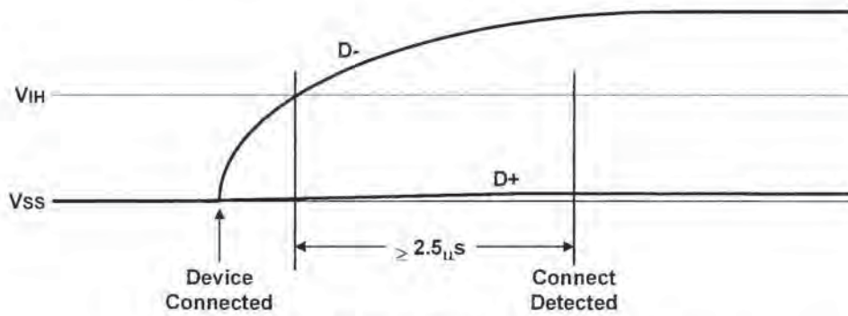
Figure 7-17. Low-speed Device Connect Detection
