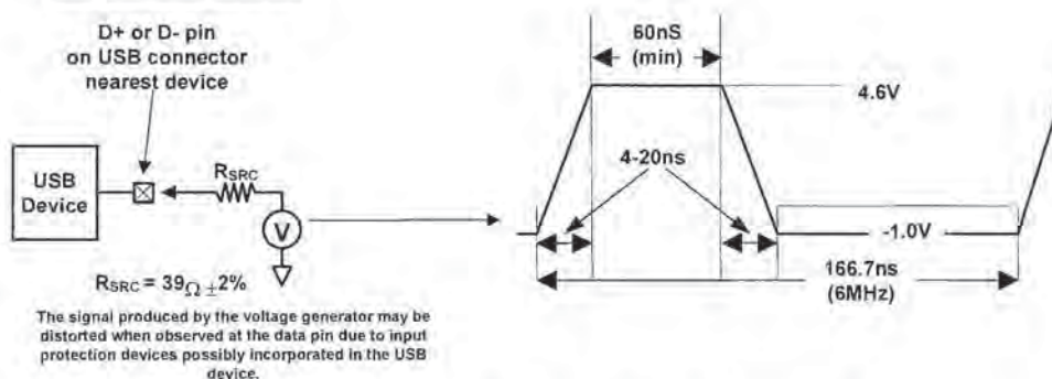
Figure 7-1. Maximum Input Waveforms for USB Signaling
