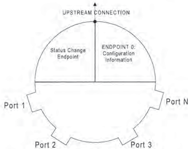
Figure 11-11. Example Hub Controller Organization
