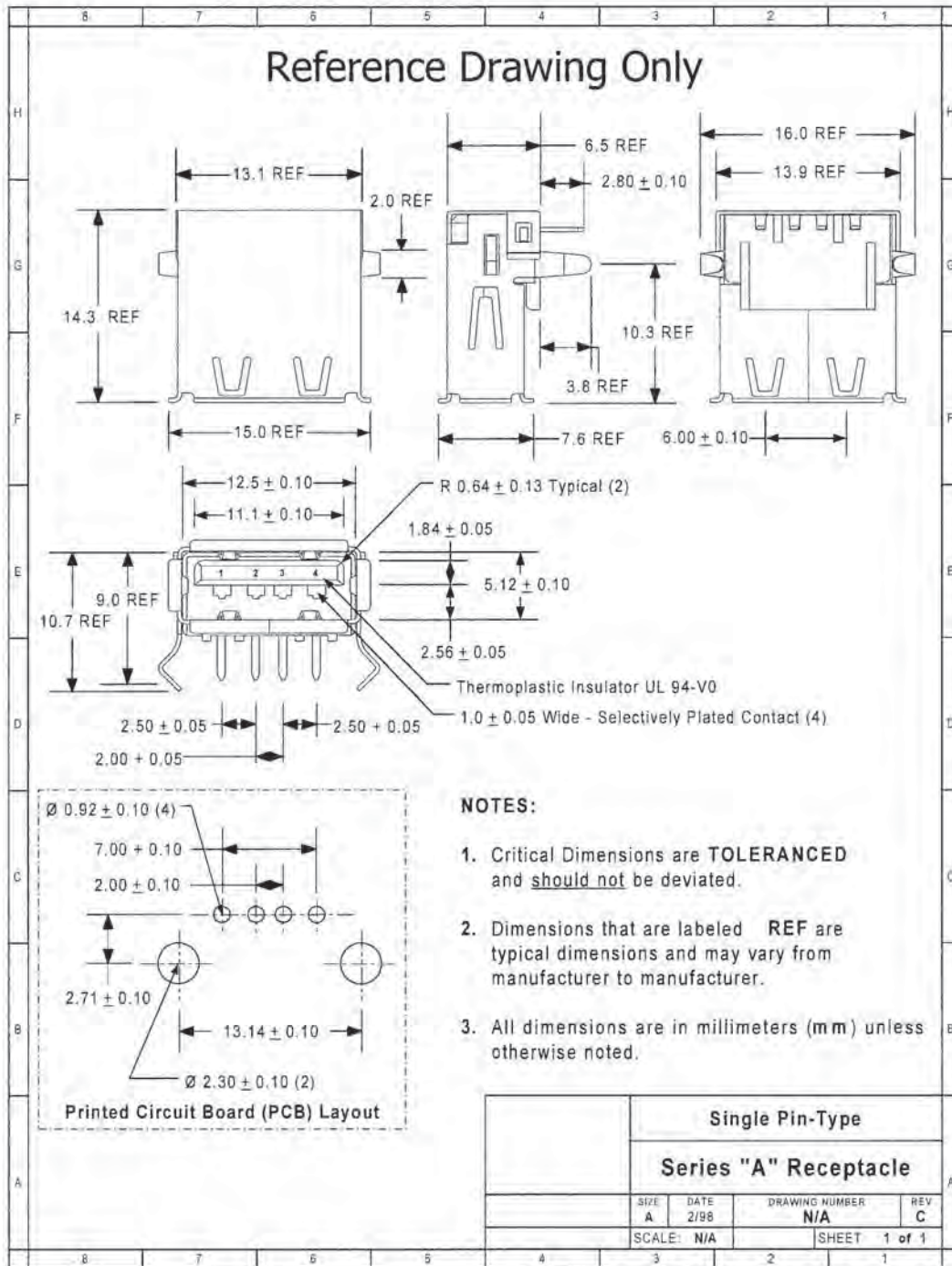
Figure 6-12. Single Pin-Type Series "A" Receptacle
