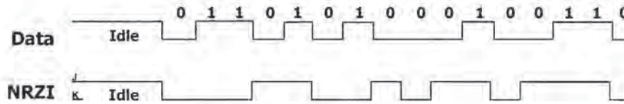
Figure 7-21. NRZI Data Encoding
