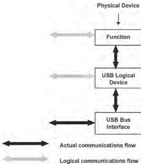
Figure 5-4. Physical Device Composition
