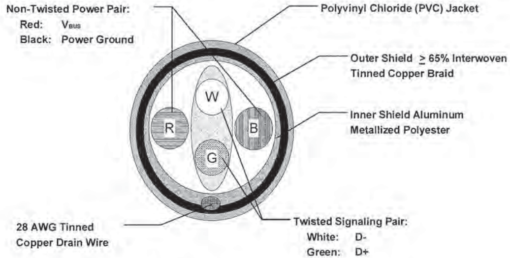
Figure 6-11. Typical Full-speed Cable Construction
