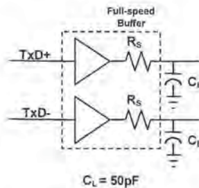
Figure 7-7. Full-speed Load
