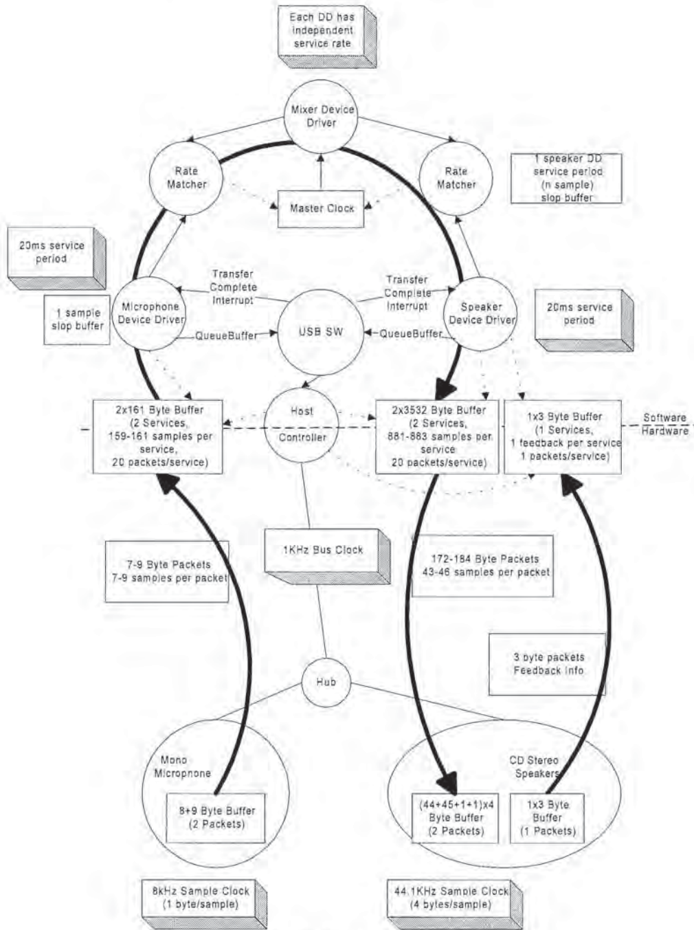
Figure 5-14. USB Isochronous Application
