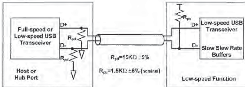
Figure 7-11. Low-speed Device Cable and Resistor Connections
