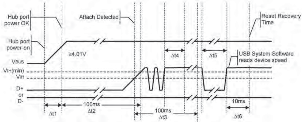
Figure 7-19. Power-on and Connection Events Timing
