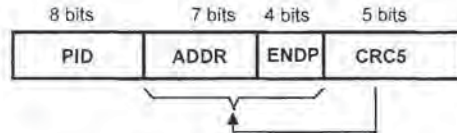
Figure 8-5. Token Format
