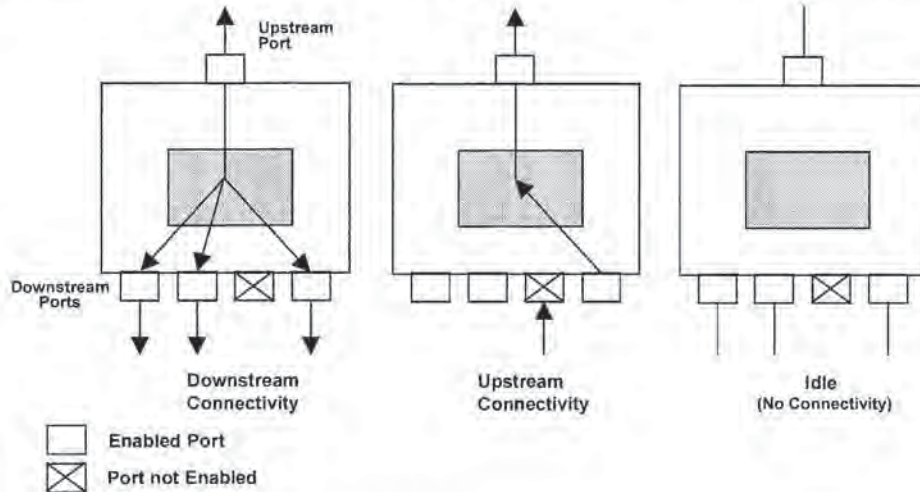
Figure 11-2. Hub Signaling Connectivity
