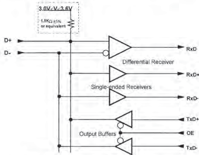
Figure 7-13. Upstream Full-speed Port Transceiver
