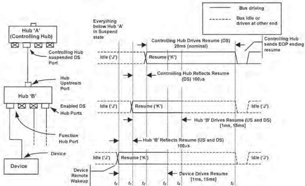
Figure 11-10. Example Remote-Wakeup Resume Signaling
