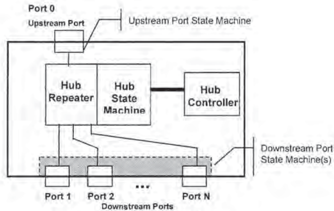
Figure 11-1. Hub Architecture
