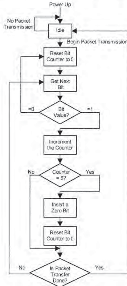
Figure 7-24. Flow Diagram for Bit Stuffing
