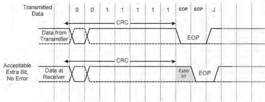
Figure 7-23. Illustration of Extra Bit Preceding EOP
