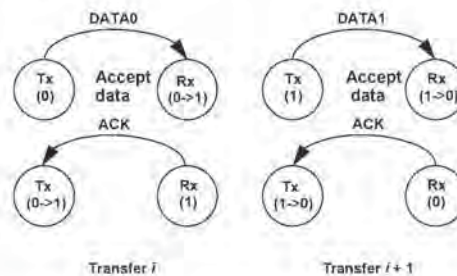
Figure 8-16. Consecutive Transactions
