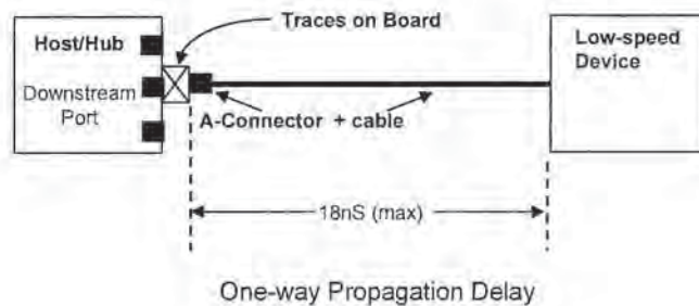
Figure 7-30. Low-speed Cable Delay
