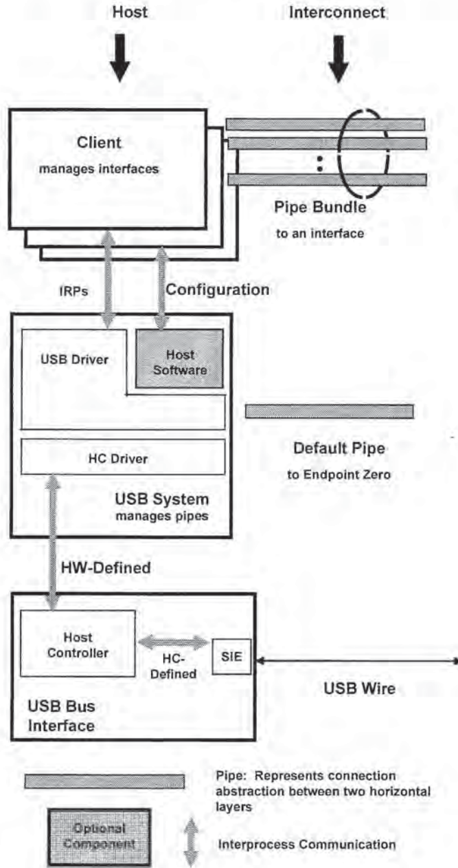
Figure 10-2. Host Communications
