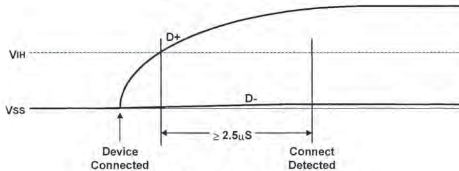
Figure 7-16. Full-speed Device Connect Detection
