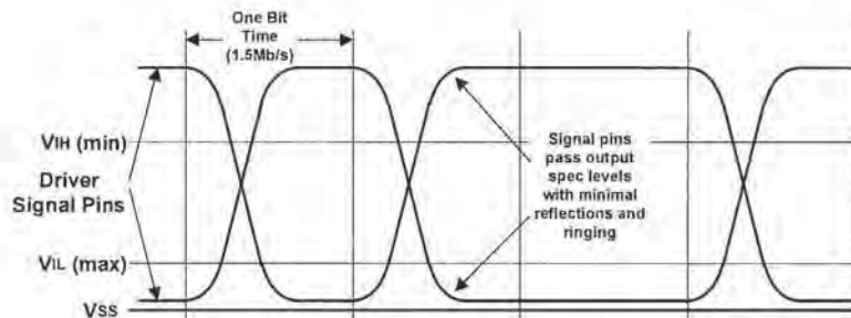
Figure 7-5. Low-speed Driver Signal Waveforms
