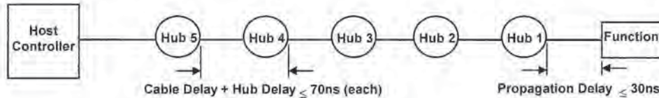
Figure 7-31. Worst-case End to End Signal Delay Model
