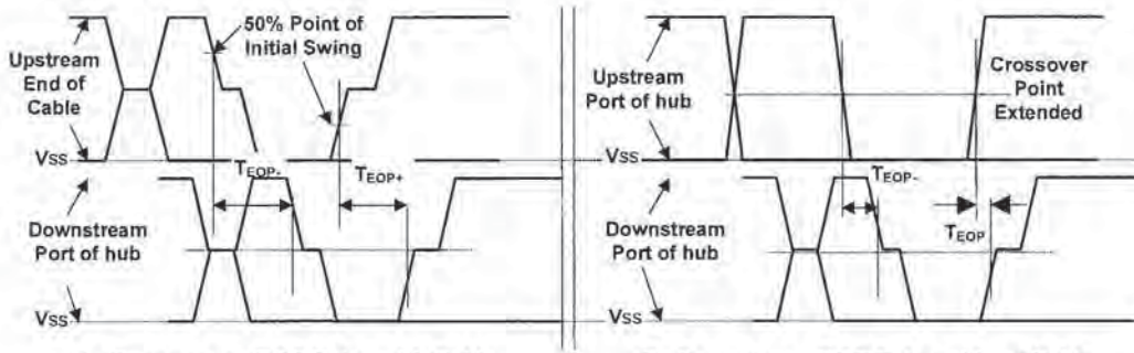
A. Downstream EOP Delay with Cable
