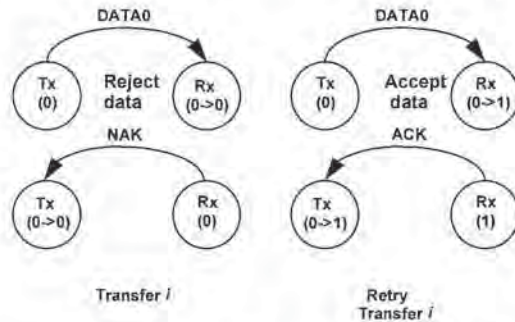
Figure 8-17. NAKed Transaction with Retry
