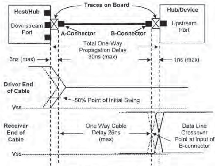
Figure 7-29. Full-speed Cable Delay
