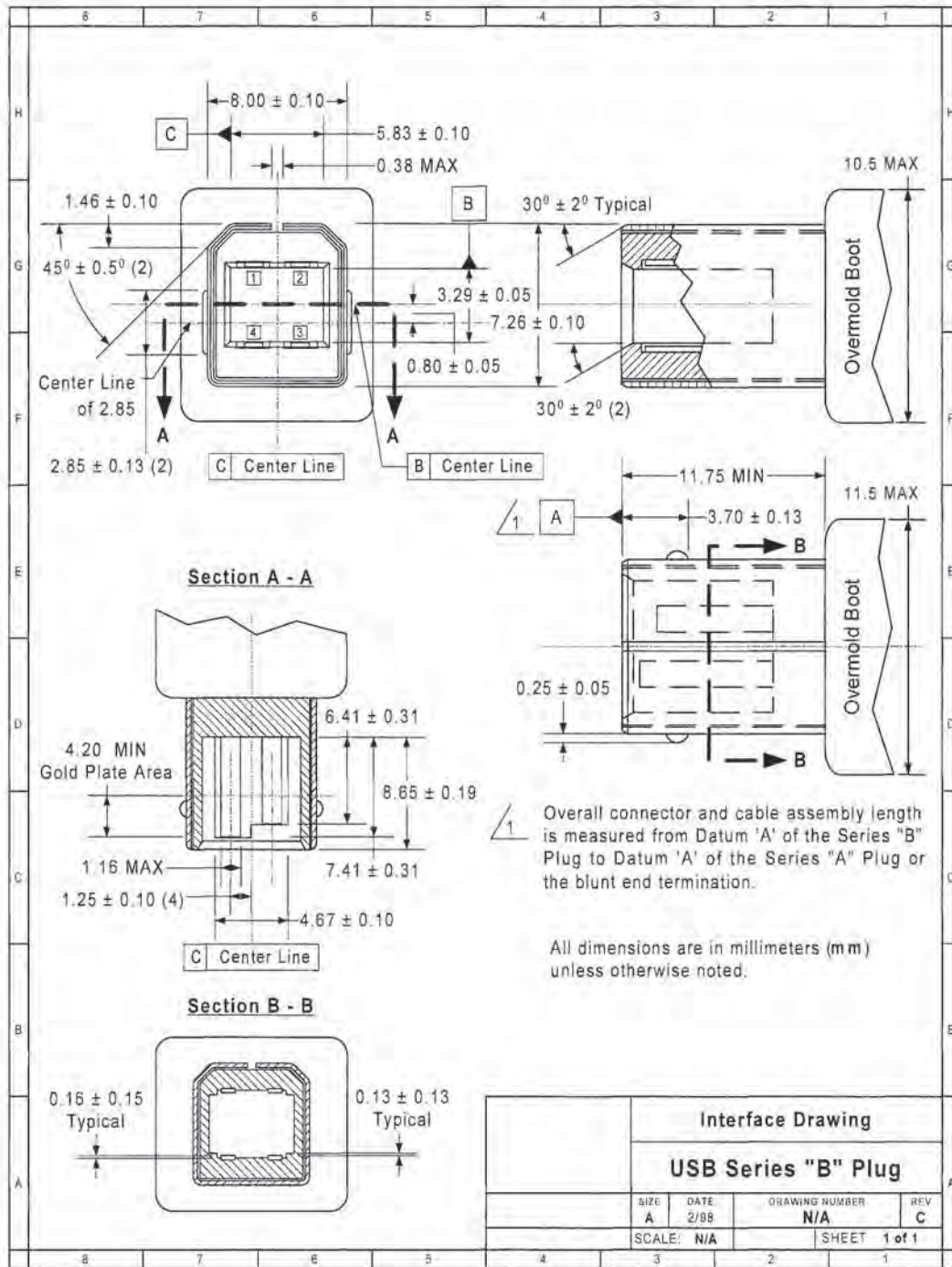
Figure 6-10. USB Series "B" Plug Interface Drawing
