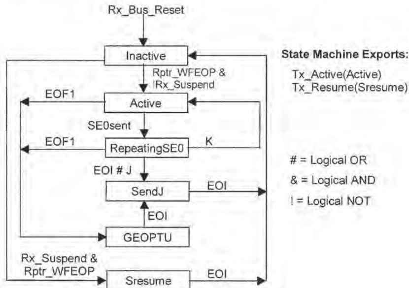
Figure 11-8. Upstream Hub Port Transmitter State Machine
