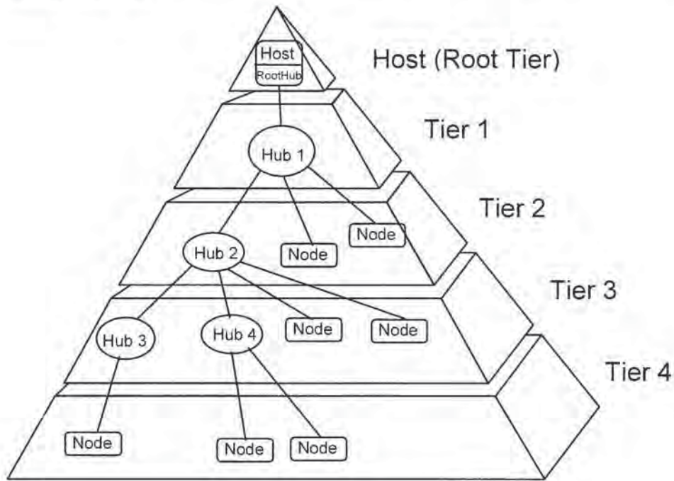
Figure 4-1. Bus Topology
