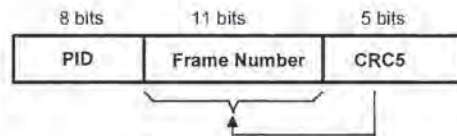
Figure 8-6. SOF Packet
