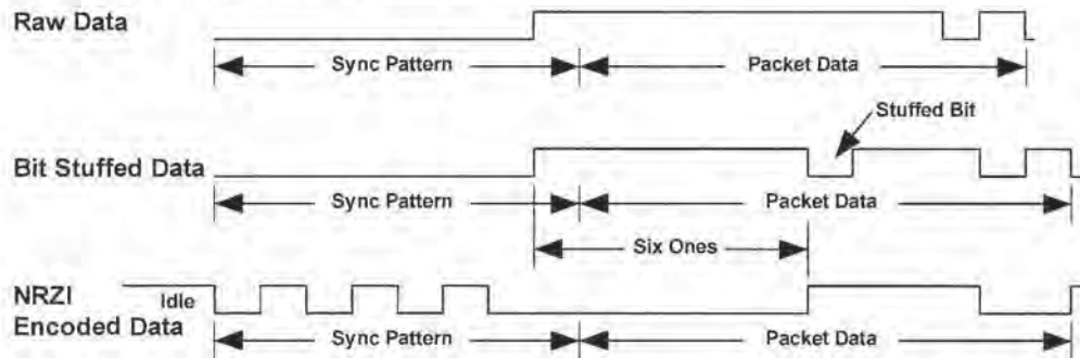
Figure 7-22. Bit Stuffing
