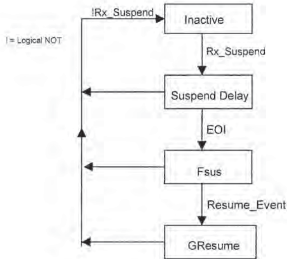
Figure 11-5. Internal Port State Machine
