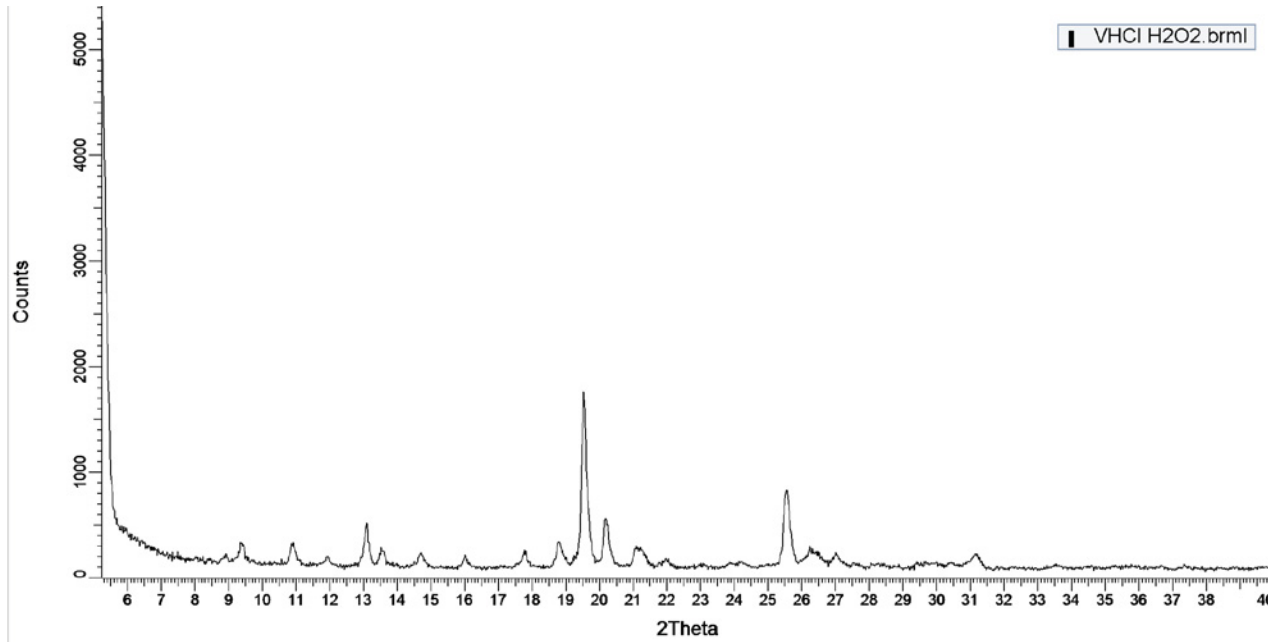
FIG. 6 shows a second PXRD of vilazodone hydrochloride after dispersed in water
