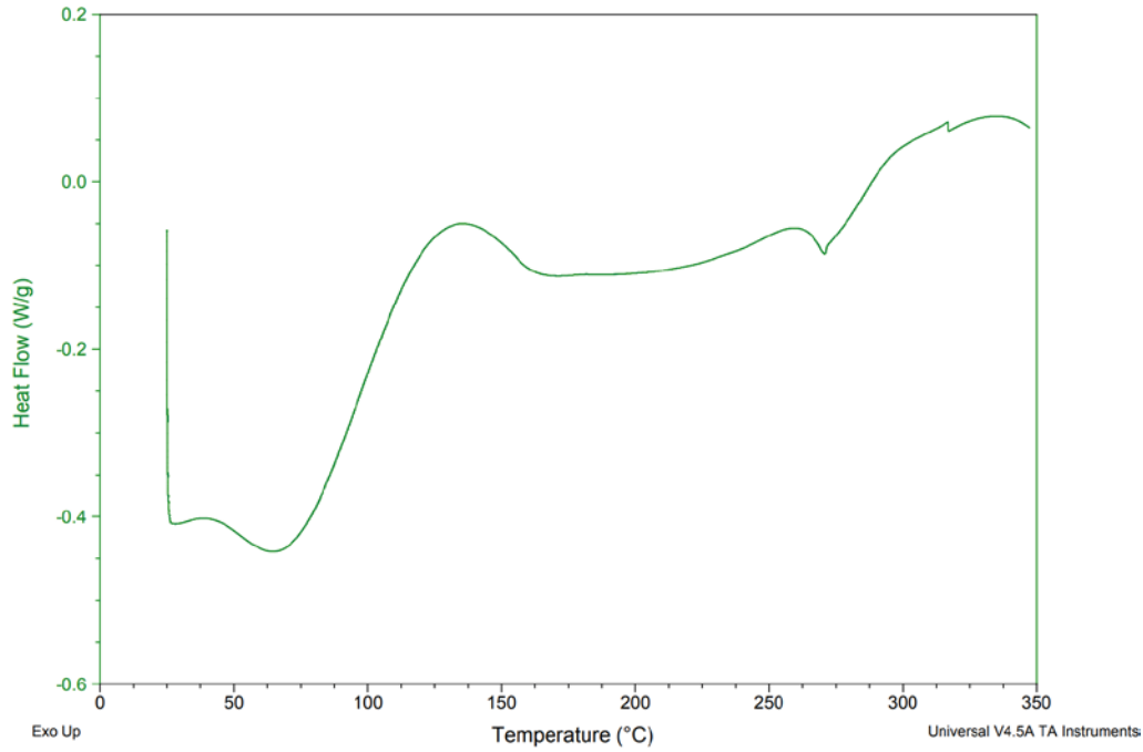
FIG. 9 shows a DSC of vilazodone hydrochloride dispersed in isopropanol
