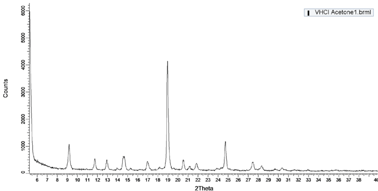
FIG. 2 shows a PXR of vilazodone hydrochloride after being dispersed in acetone
