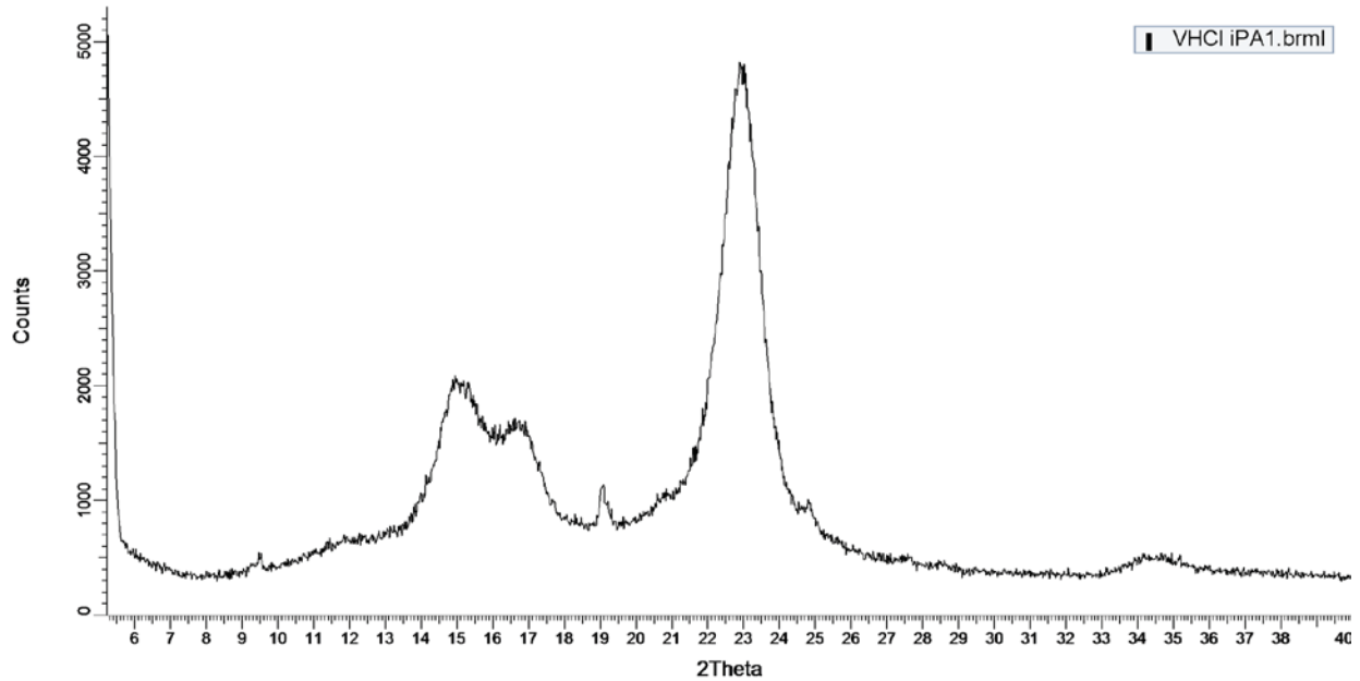
FIG. 4 shows a PXRD of vilazodone hydrochloride after dispersed in isopropanol
