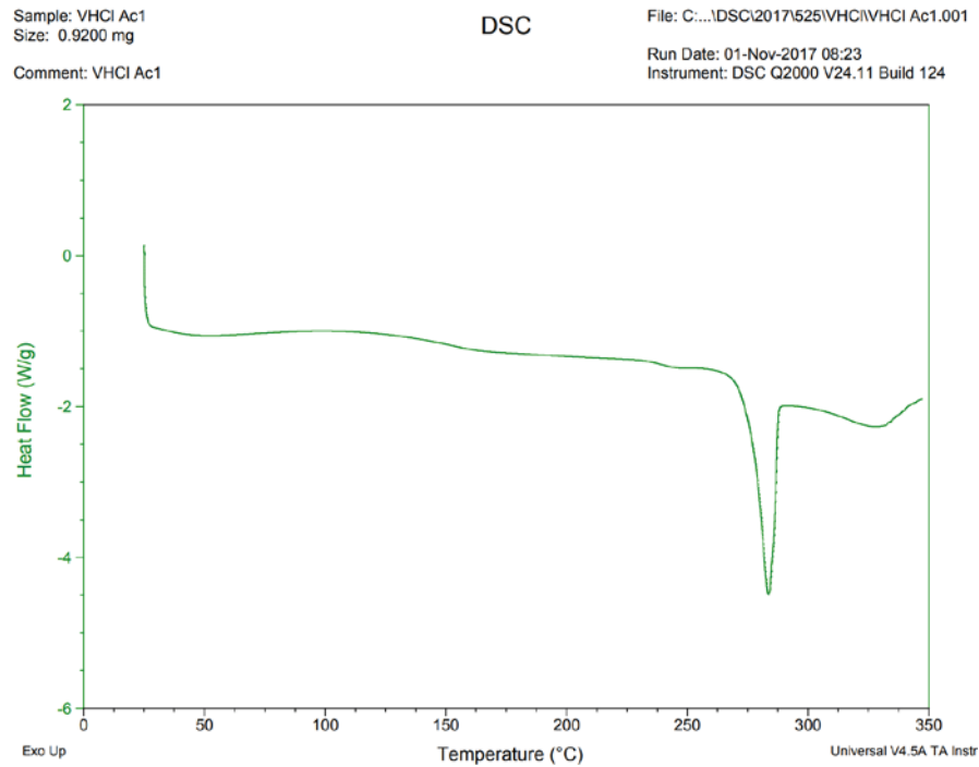
FIG. 8 shows a DSC of vilazodone hydrochloride dispersed in acetone
