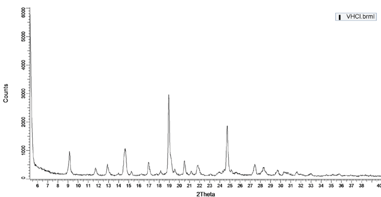
FIG. 1 shows a PXR of the vilazodone hydrochloride starting material bought from Sigma-Aldrich.
