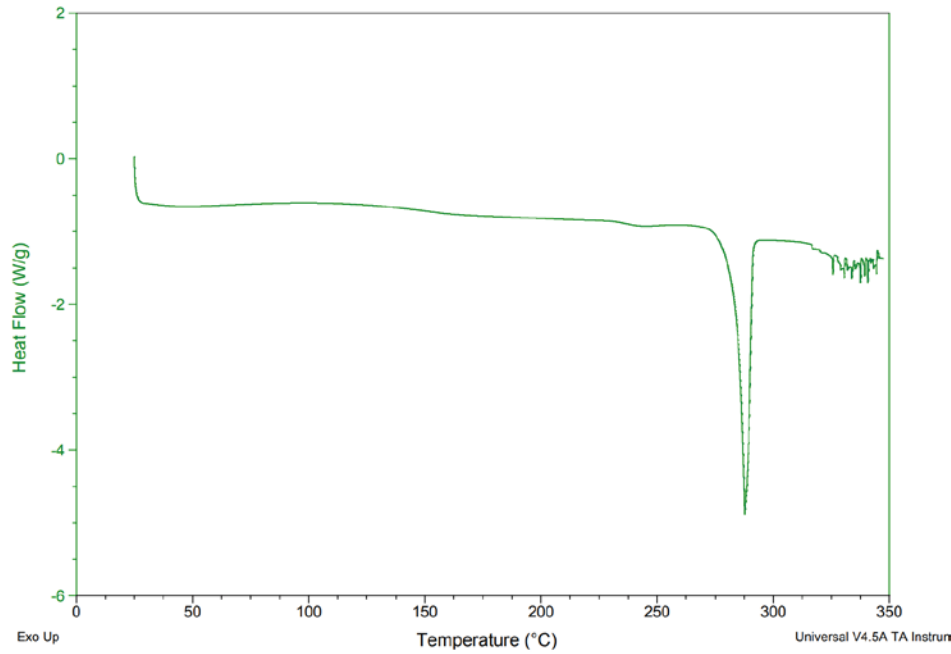
FIG. 10 shows a second DSC of vilazodone hydrochloride dispersed in isopropanol
