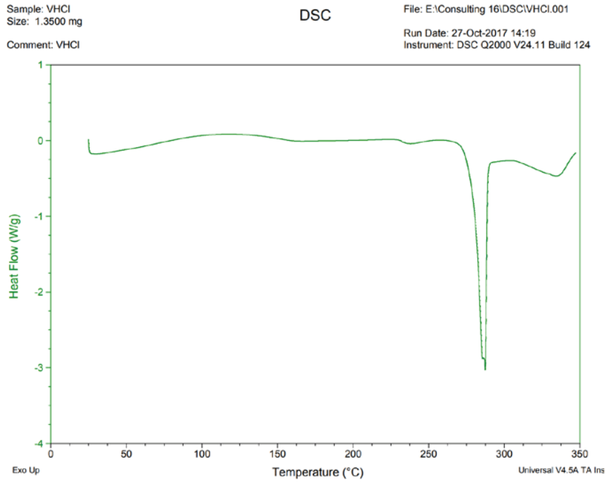
FIG. 7 shows a DSC of vilazodone hydrochloride starting material purchased from Sigma-Aldrich
